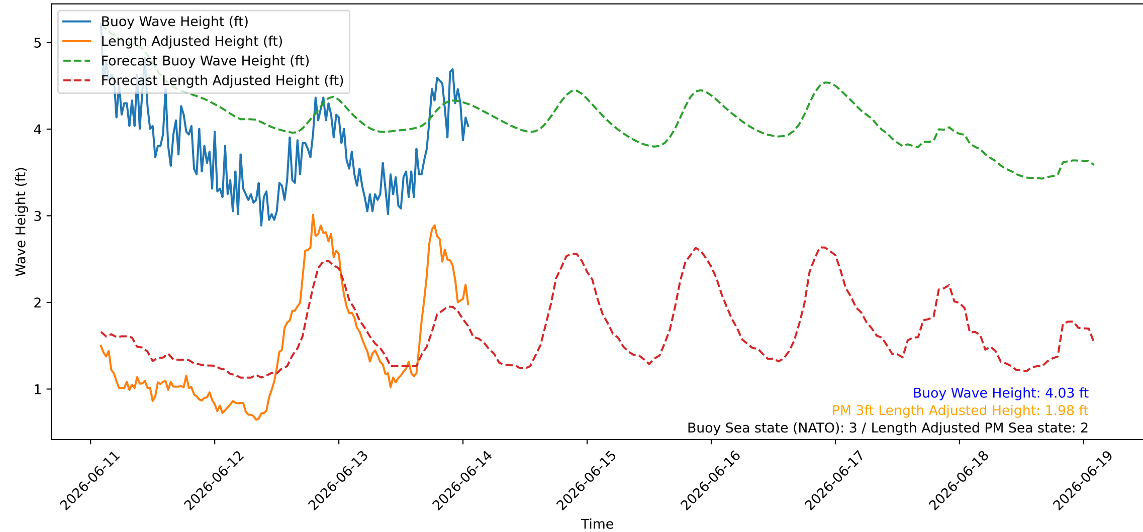
Wave Heights over Time for Green Beach at 2026-06-14 02:01:10
