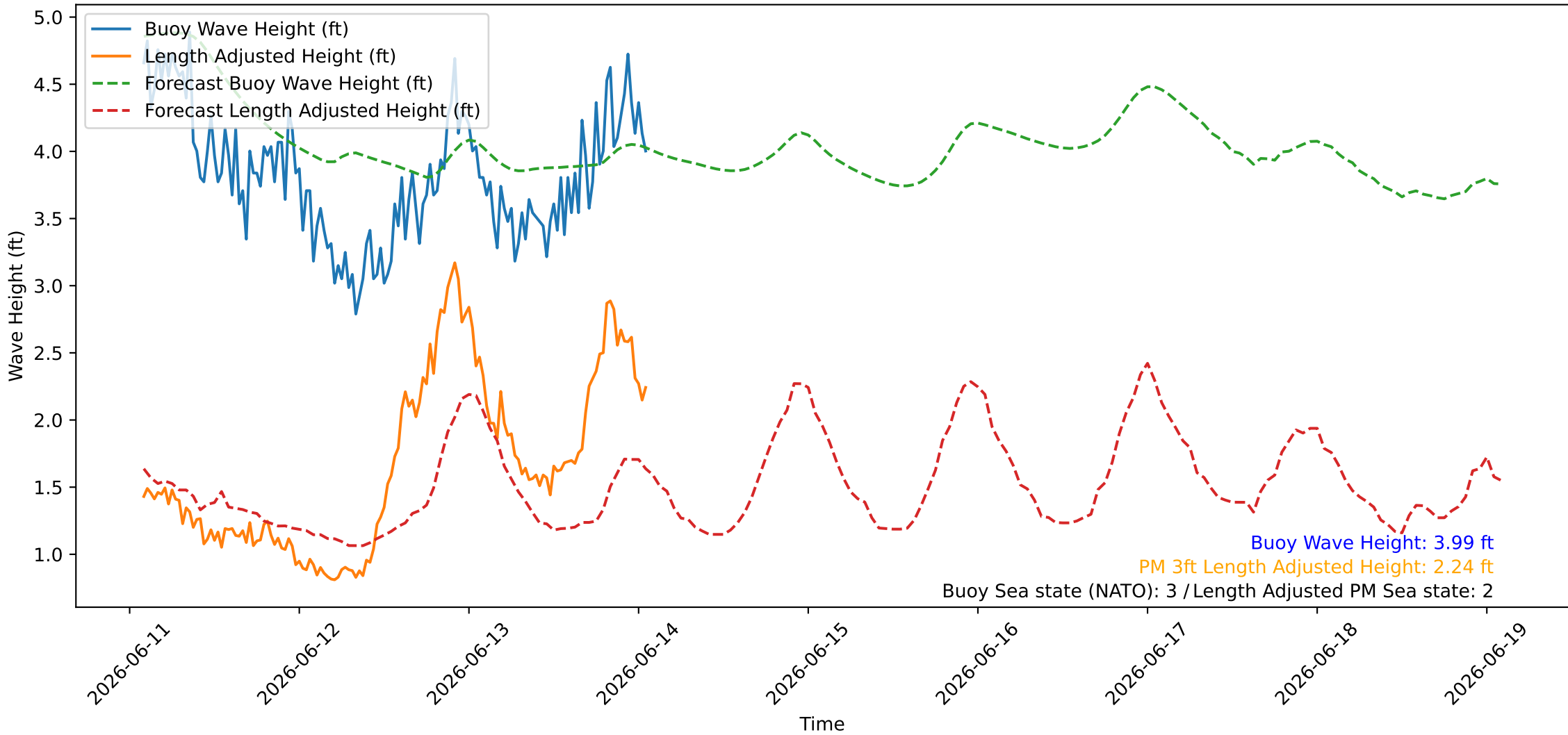
Wave Heights over Time for Oceanside Harbor at 2026-06-14 02:00:26
