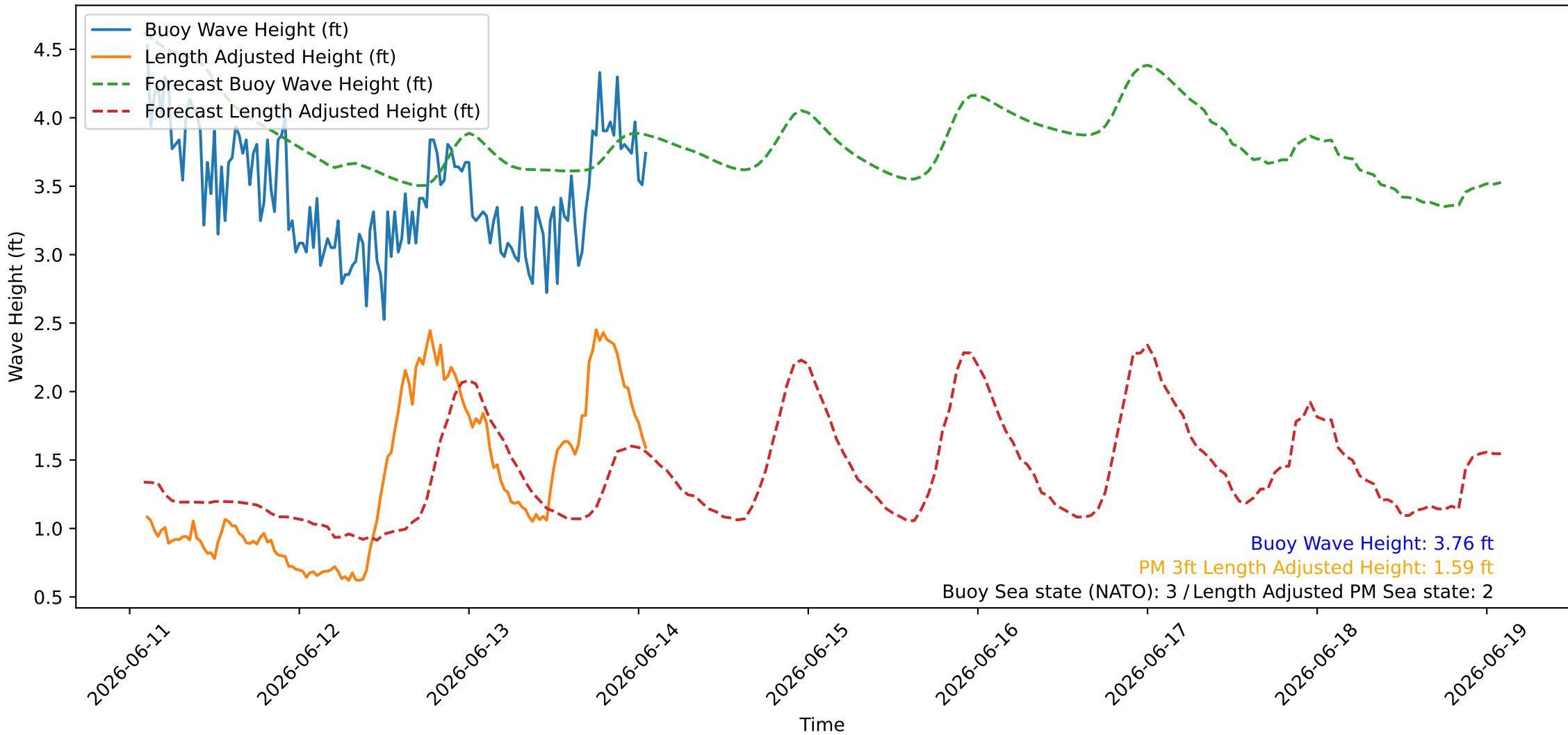
Wave Heights over Time for Red Beach at 2026-06-14 02:00:46
