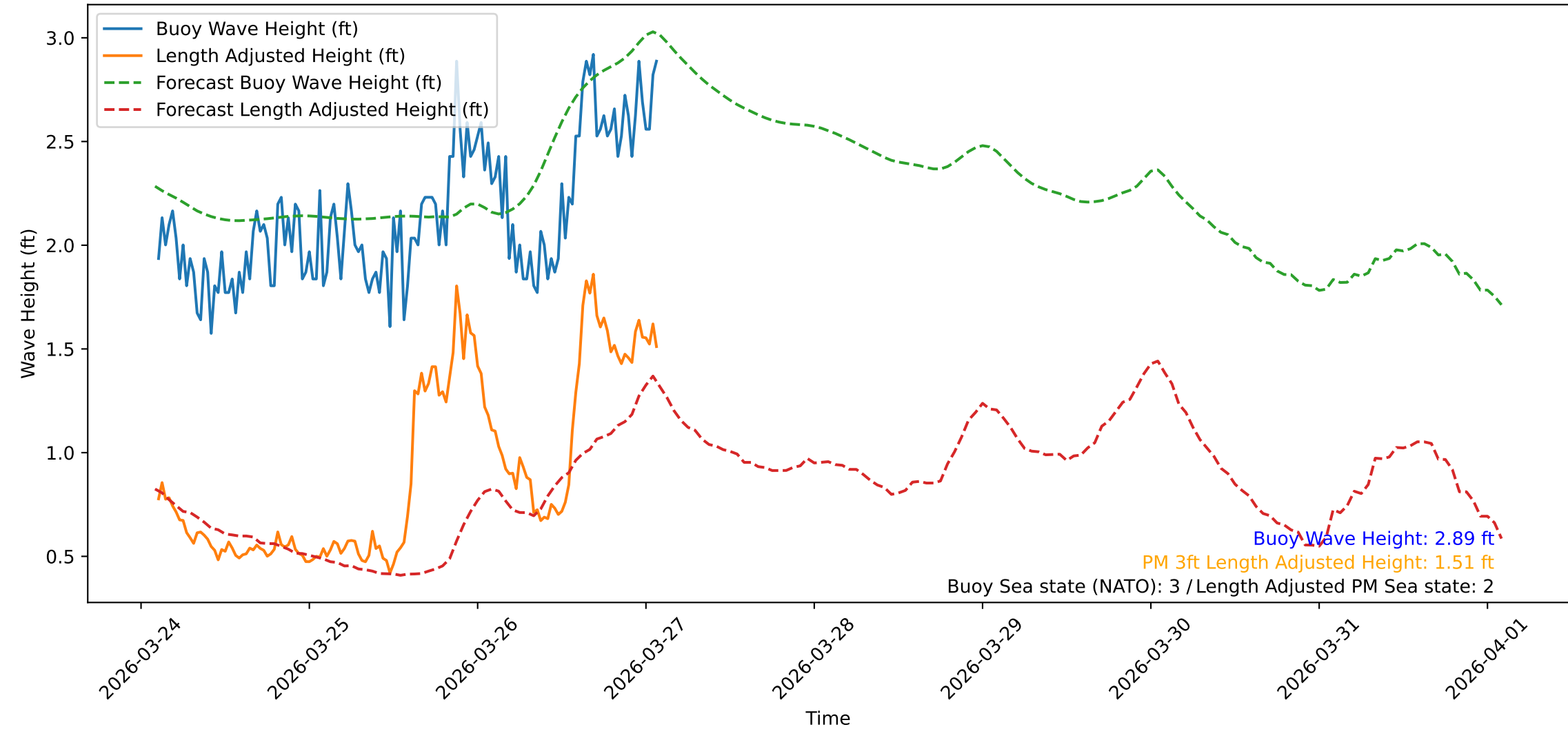
Wave Heights over Time for Oceanside Harbor at 2026-03-27 02:20:32
