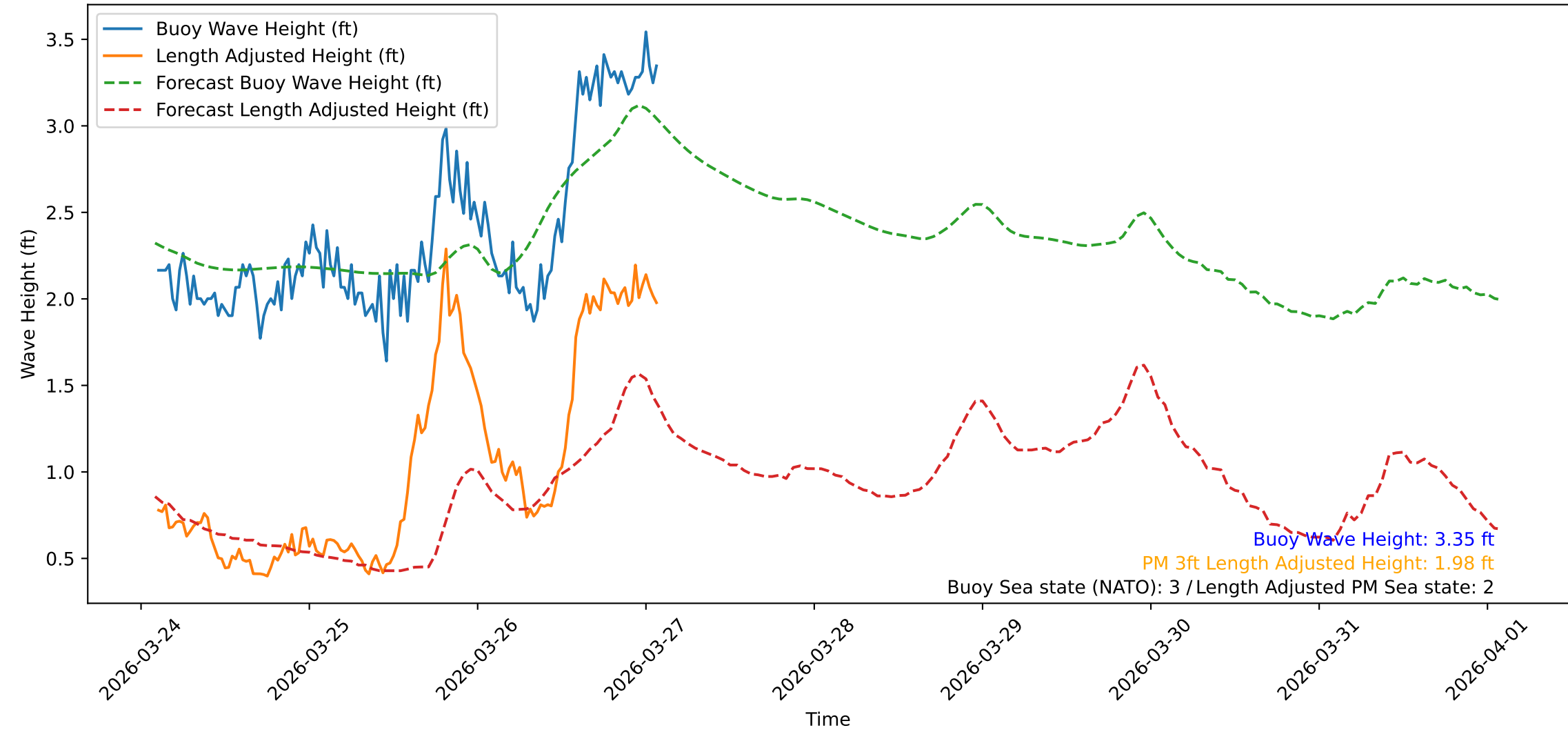
Wave Heights over Time for Green Beach at 2026-03-27 02:21:09
