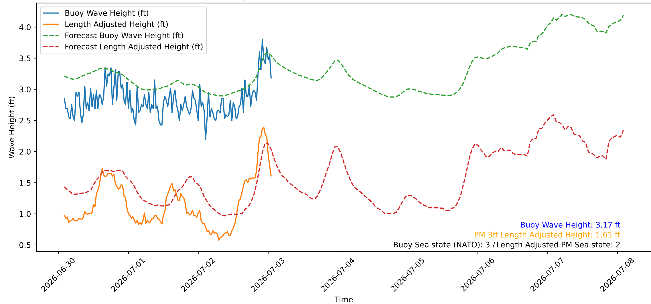
Wave Heights over Time for Red Beach at 2026-07-03 01:50:46
