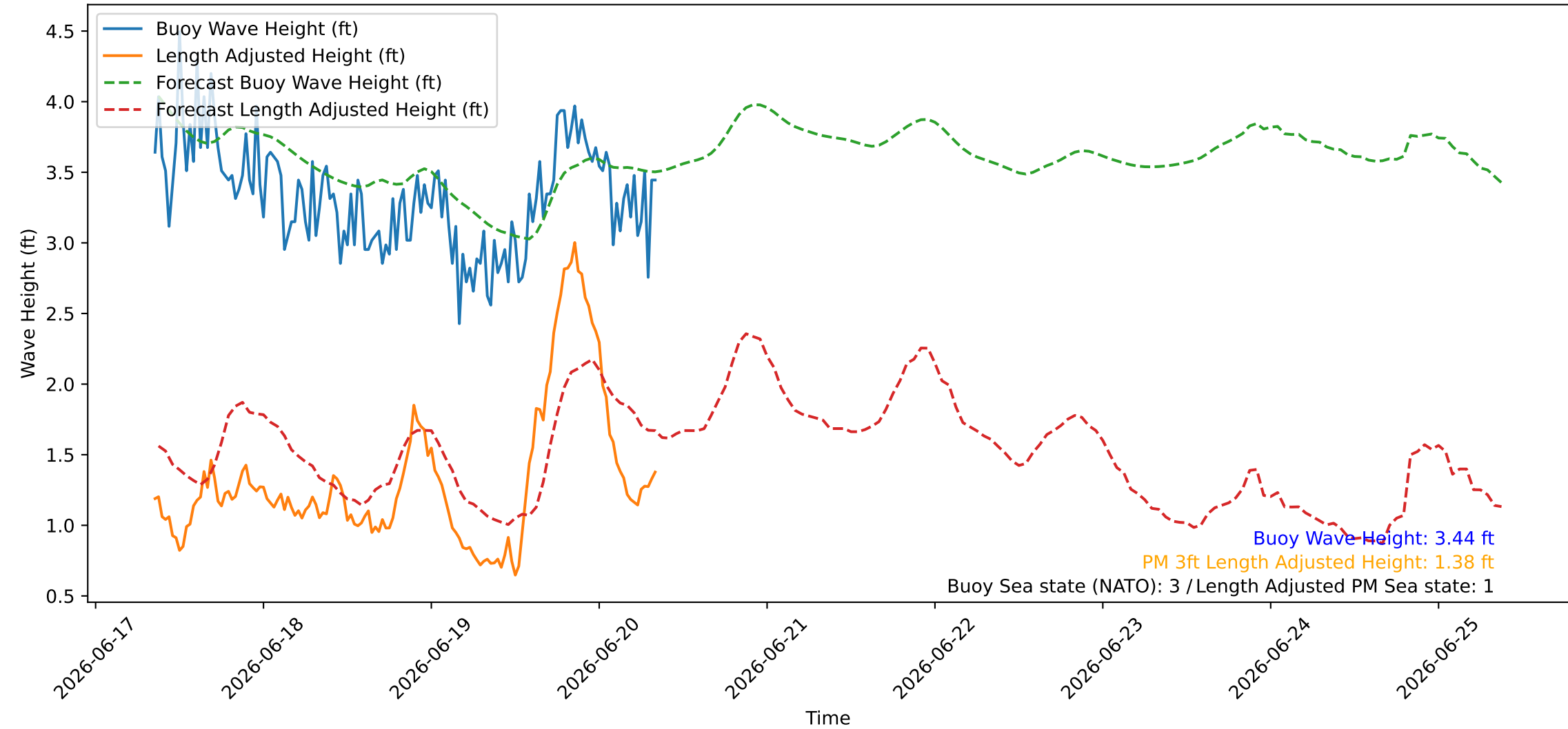
Wave Heights over Time for Green Beach at 2026-06-20 08:41:07
