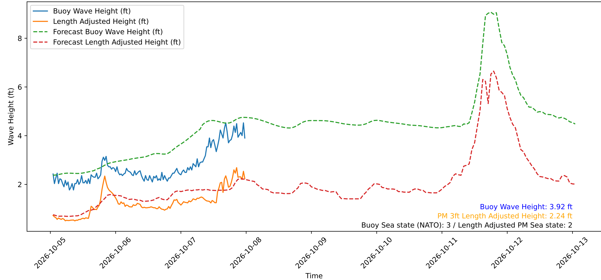
Wave Heights over Time for Green Beach at 2026-10-08 00:31:11
