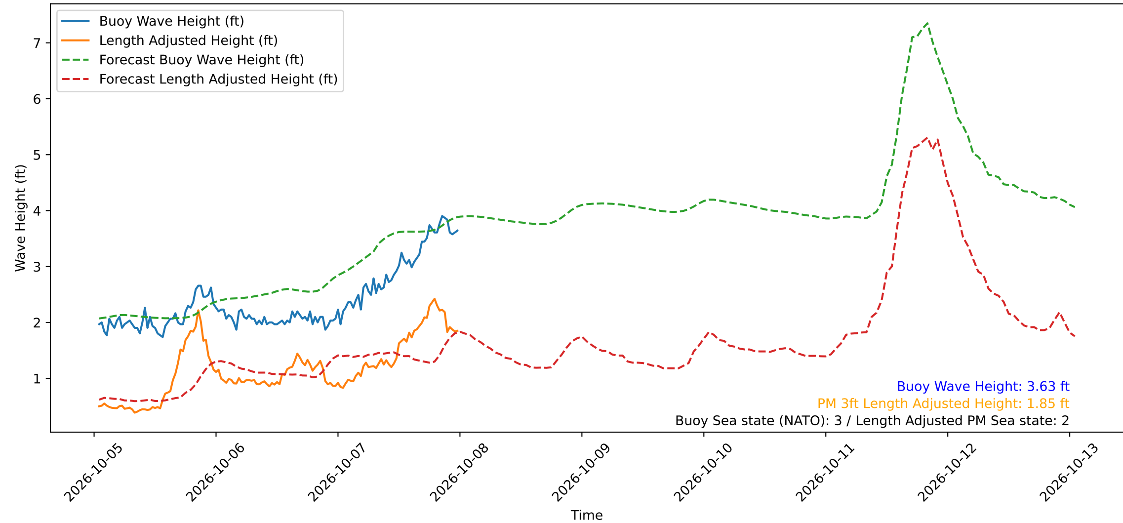
Wave Heights over Time for Red Beach at 2026-10-08 00:30:49
