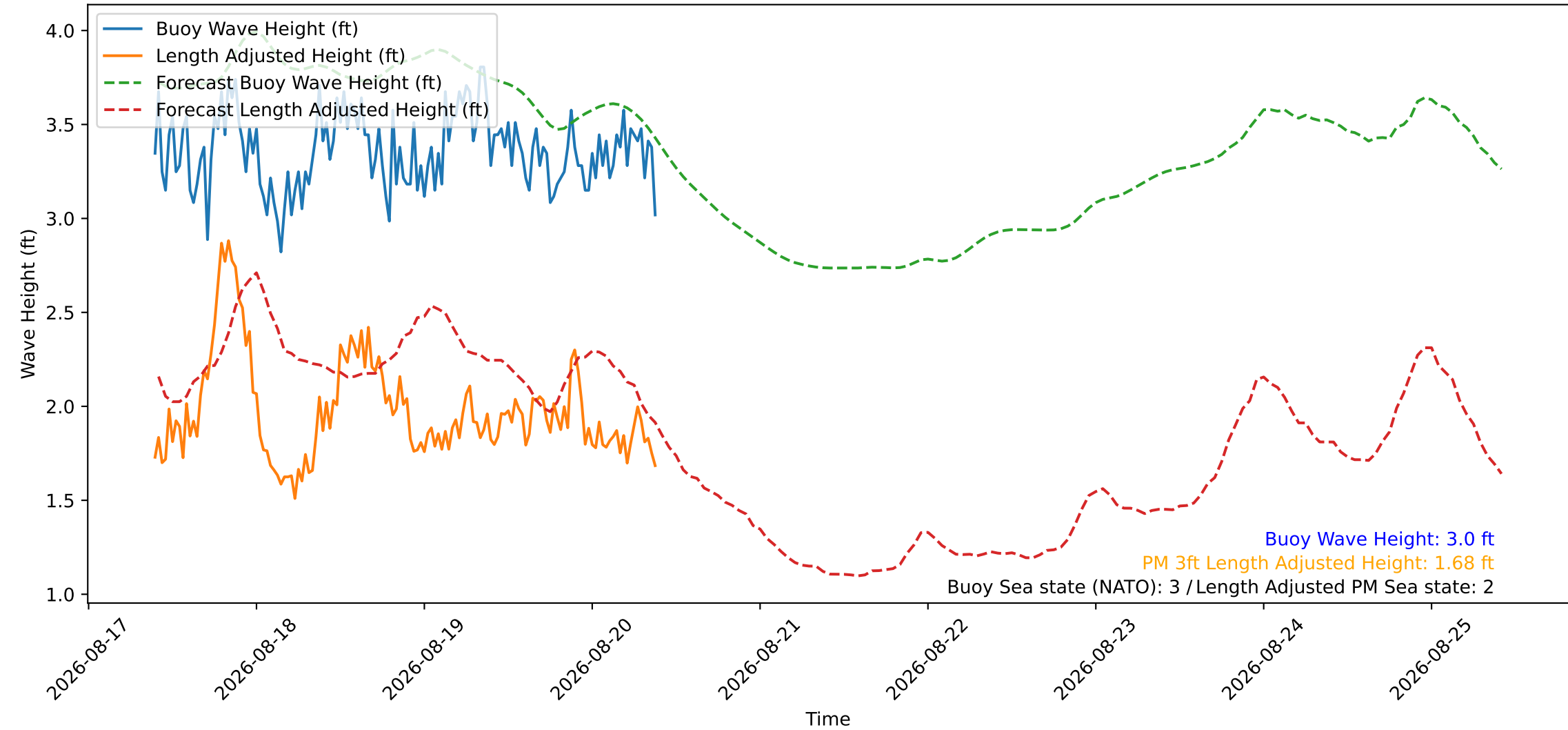
Wave Heights over Time for Oceanside Harbor at 2026-08-20 09:40:26
