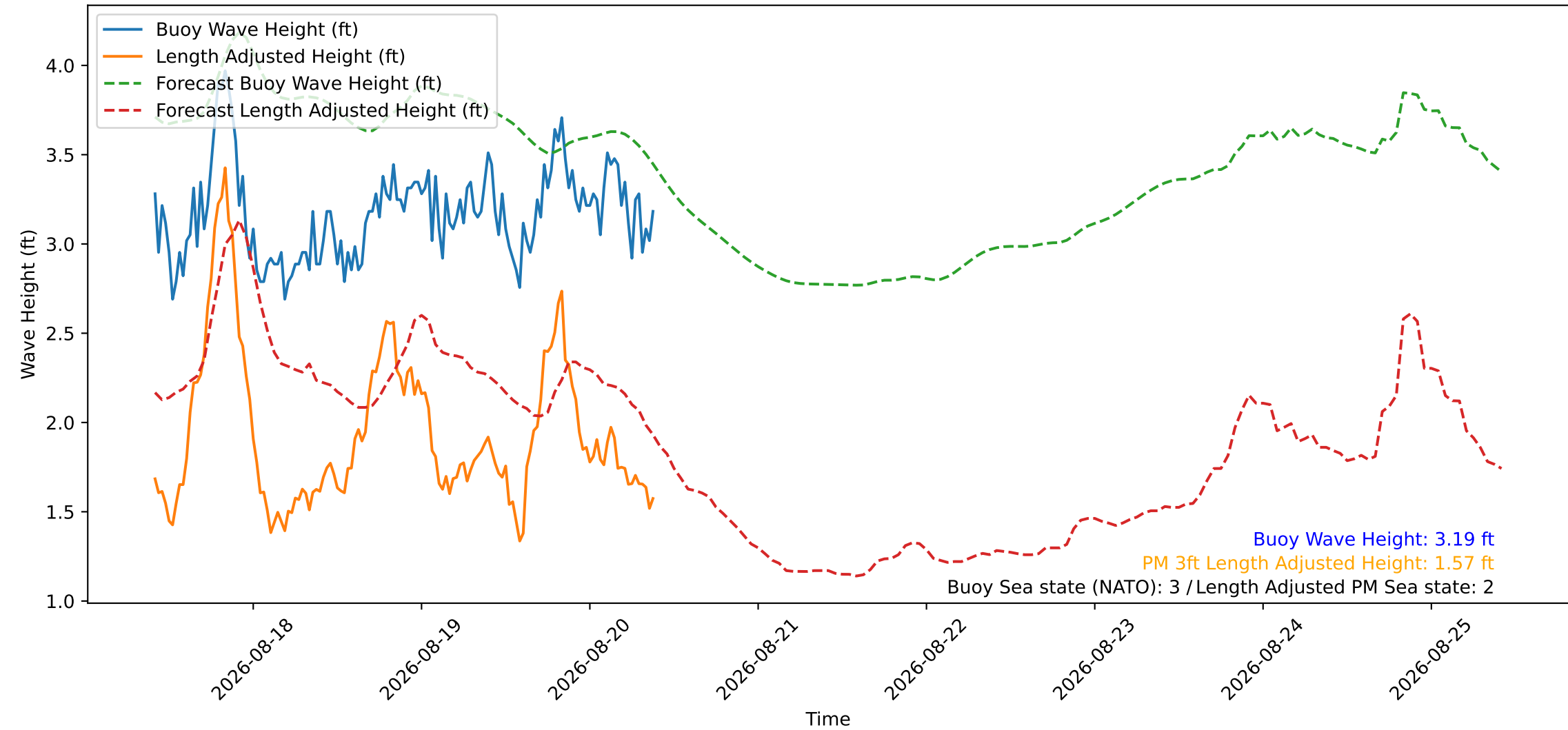
Wave Heights over Time for Green Beach at 2026-08-20 09:41:08
