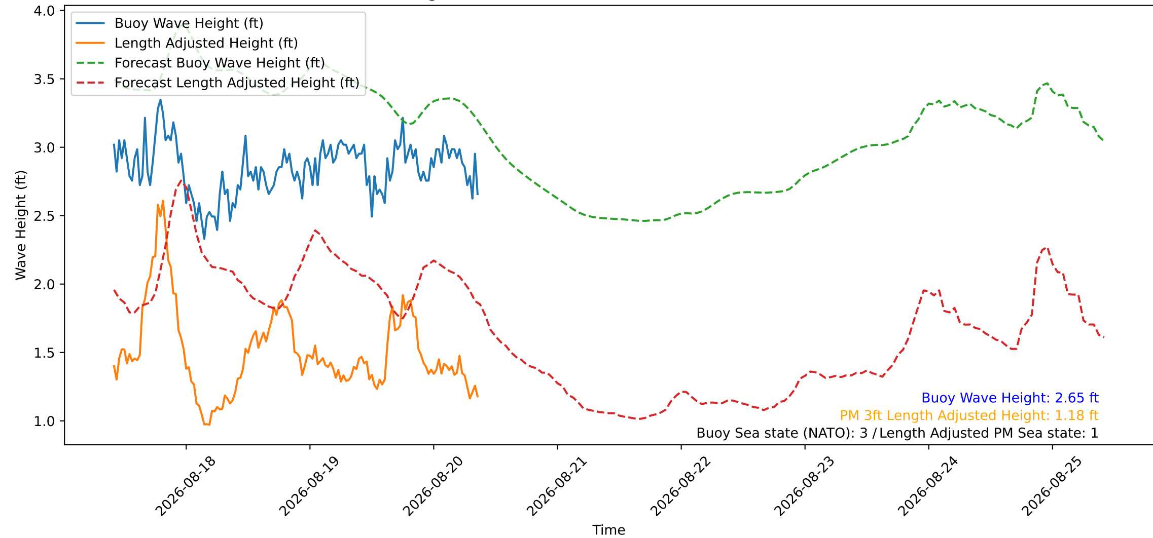
Wave Heights over Time for Red Beach at 2026-08-20 09:40:46
