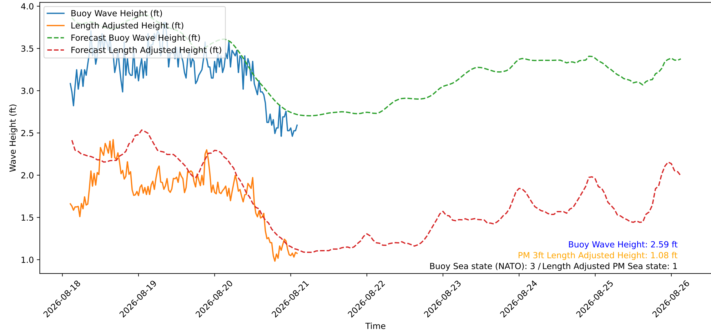
Wave Heights over Time for Oceanside Harbor at 2026-08-21 02:30:27
