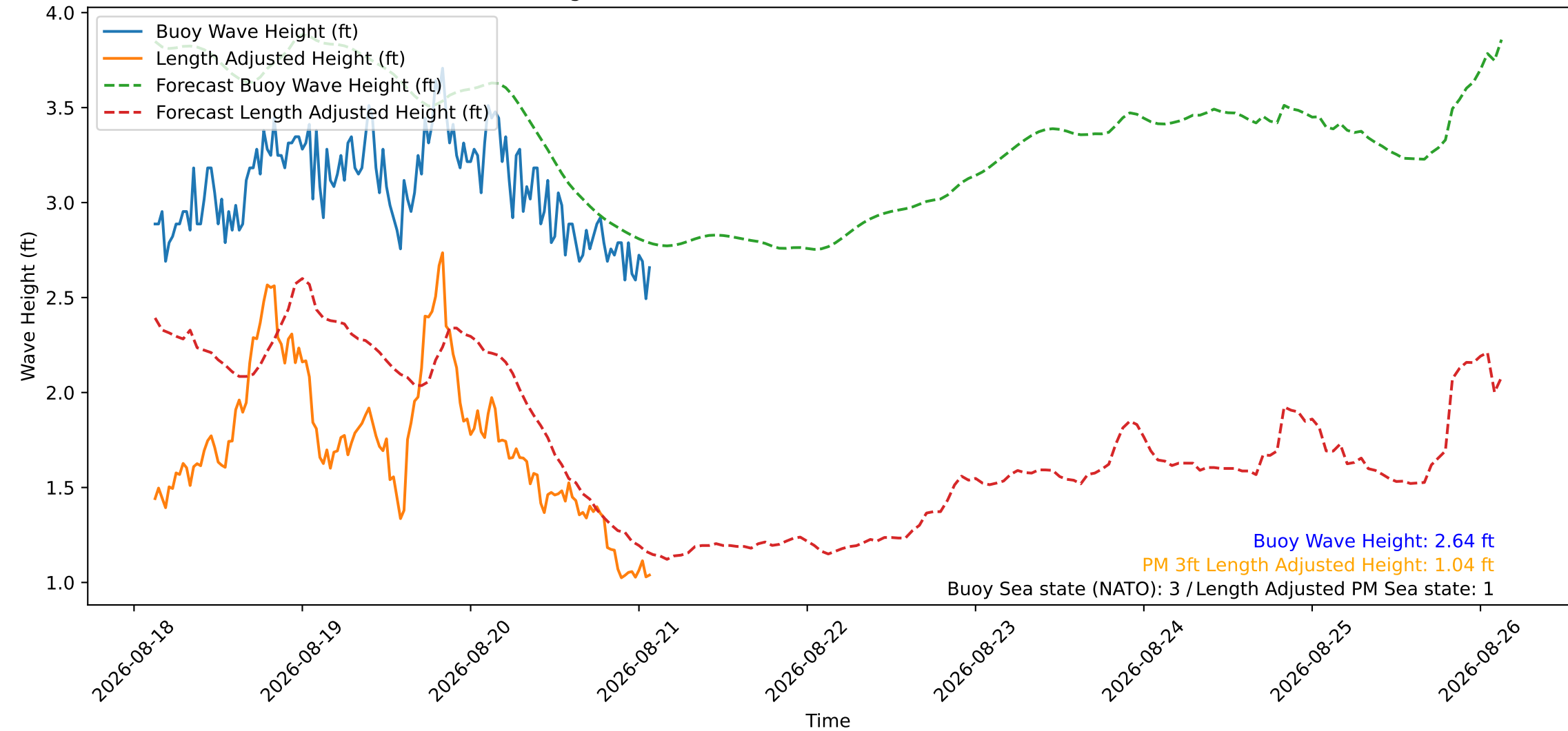
Wave Heights over Time for Green Beach at 2026-08-21 02:31:08
