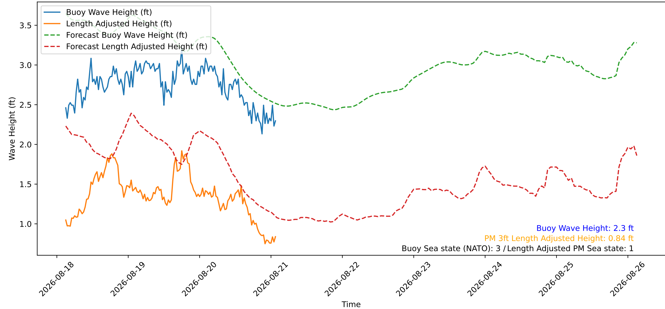
Wave Heights over Time for Red Beach at 2026-08-21 02:30:46
