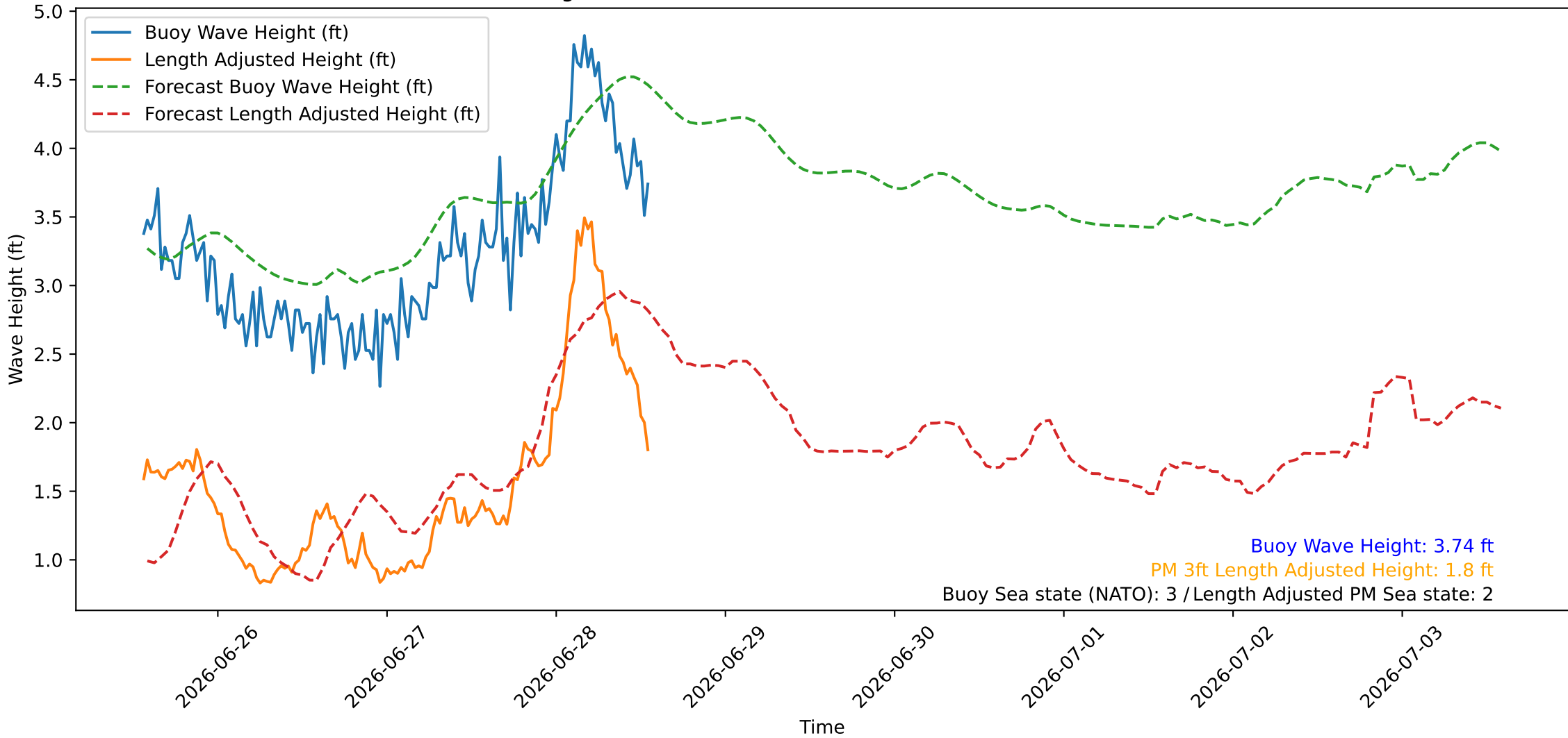
Wave Heights over Time for Green Beach at 2026-06-28 13:41:08
