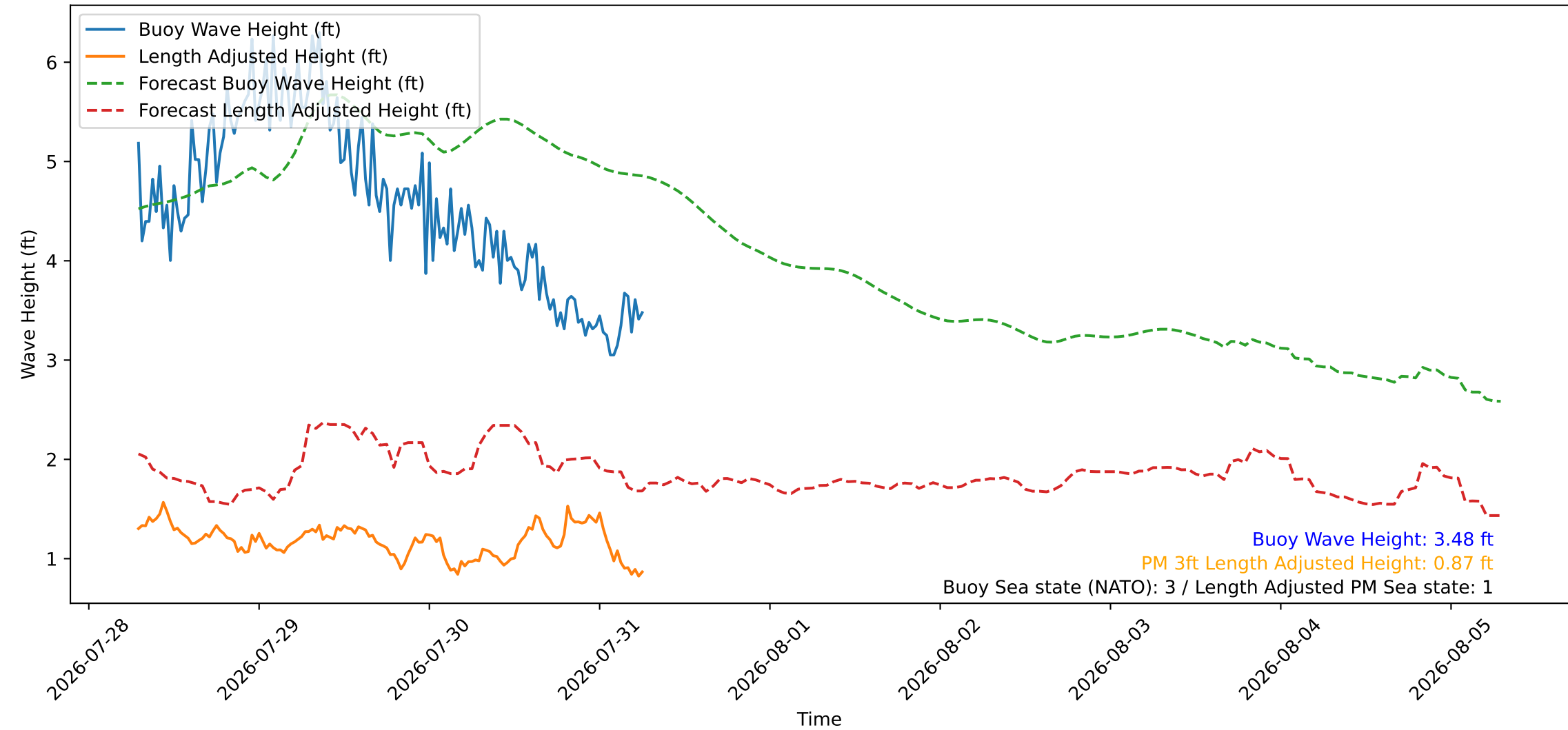
Wave Heights over Time for Green Beach at 2026-07-31 06:51:10
