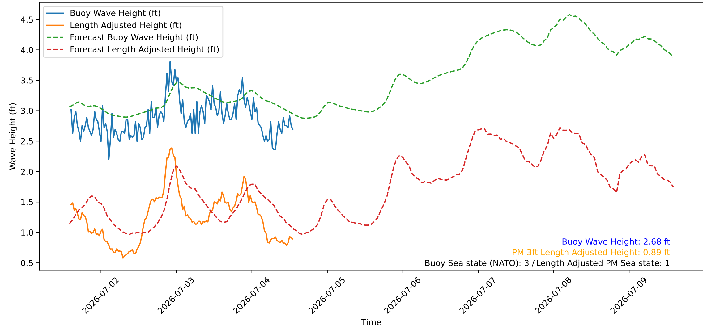
Wave Heights over Time for Red Beach at 2026-07-04 14:10:46
