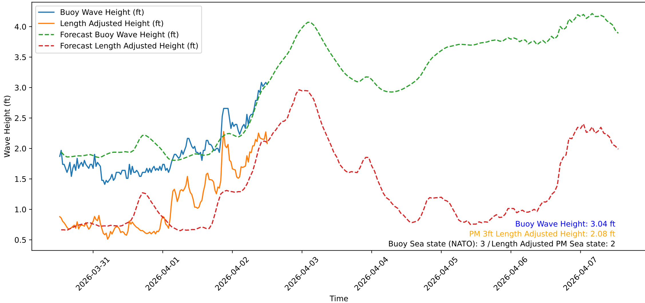
Wave Heights over Time for Green Beach at 2026-04-02 12:41:09
