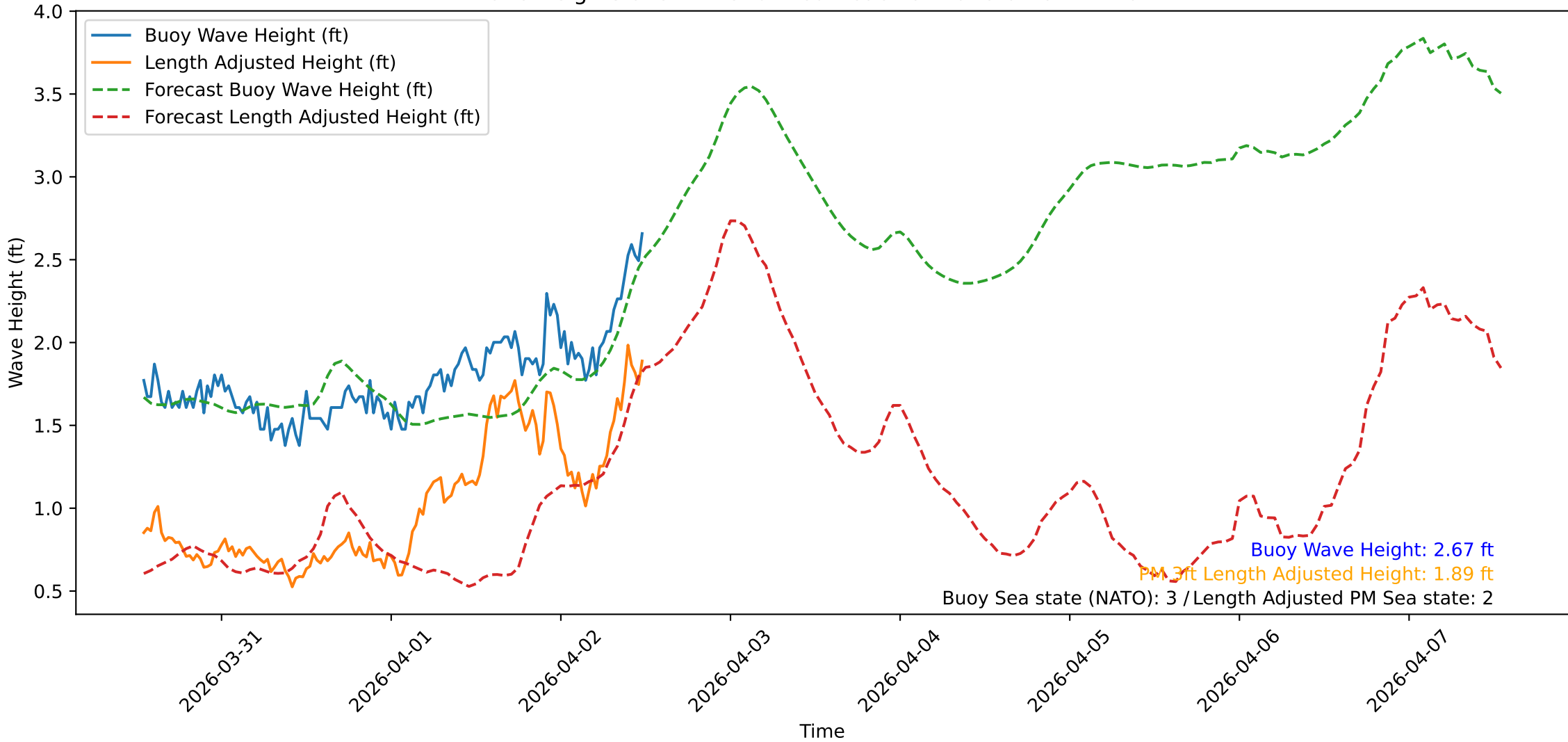
Wave Heights over Time for Red Beach at 2026-04-02 12:40:47
