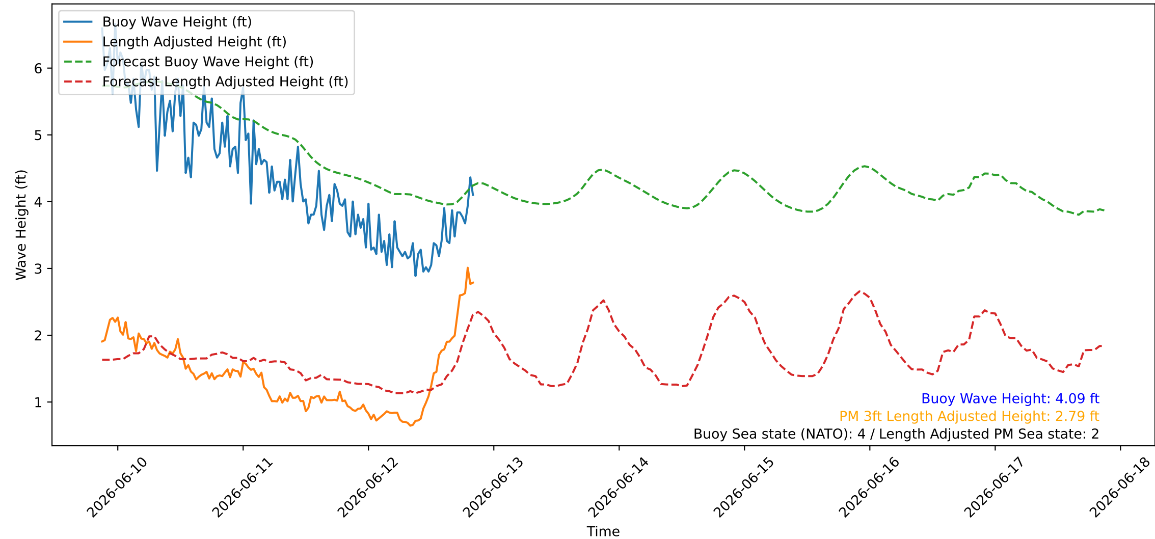
Wave Heights over Time for Green Beach at 2026-06-12 21:01:09
