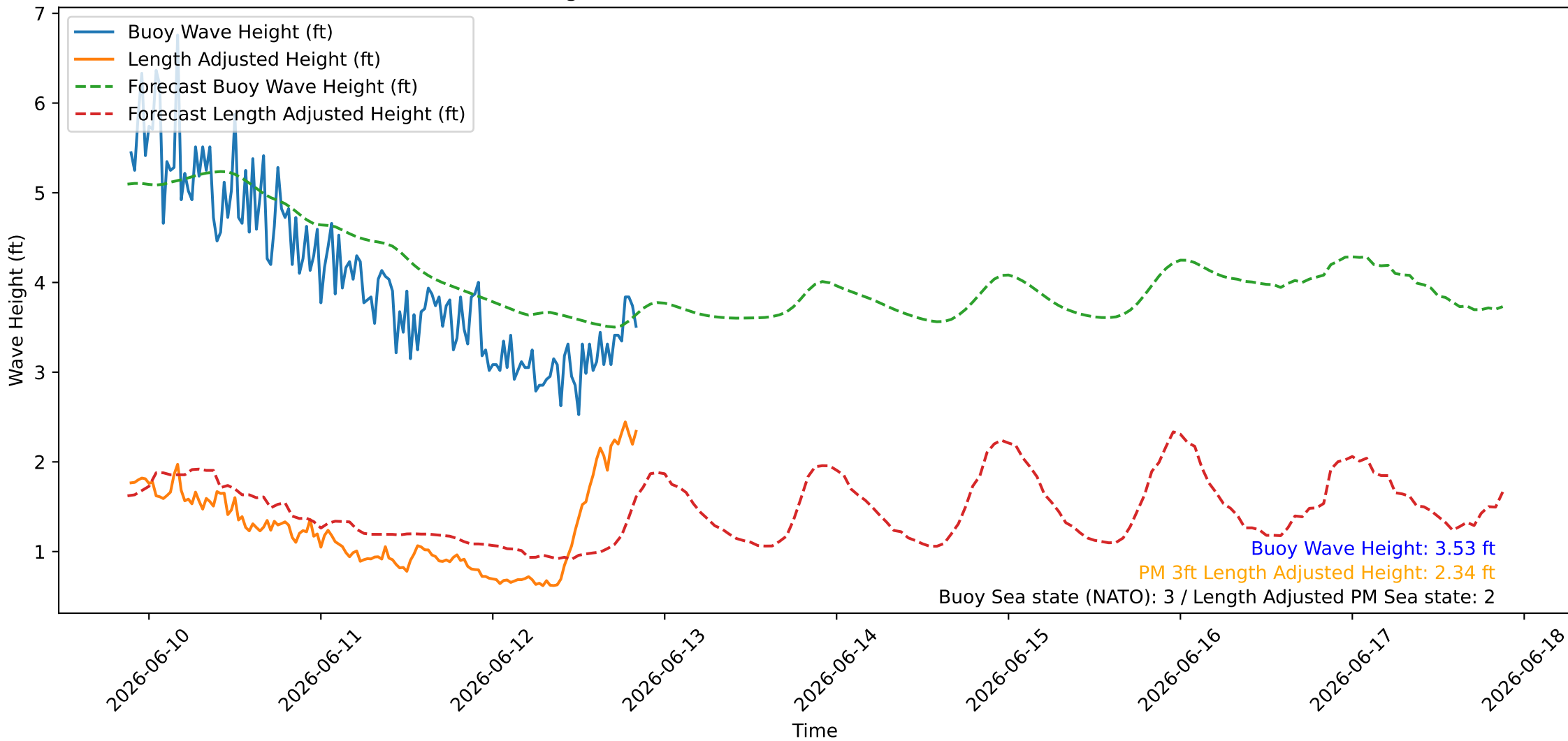
Wave Heights over Time for Red Beach at 2026-06-12 21:00:46
