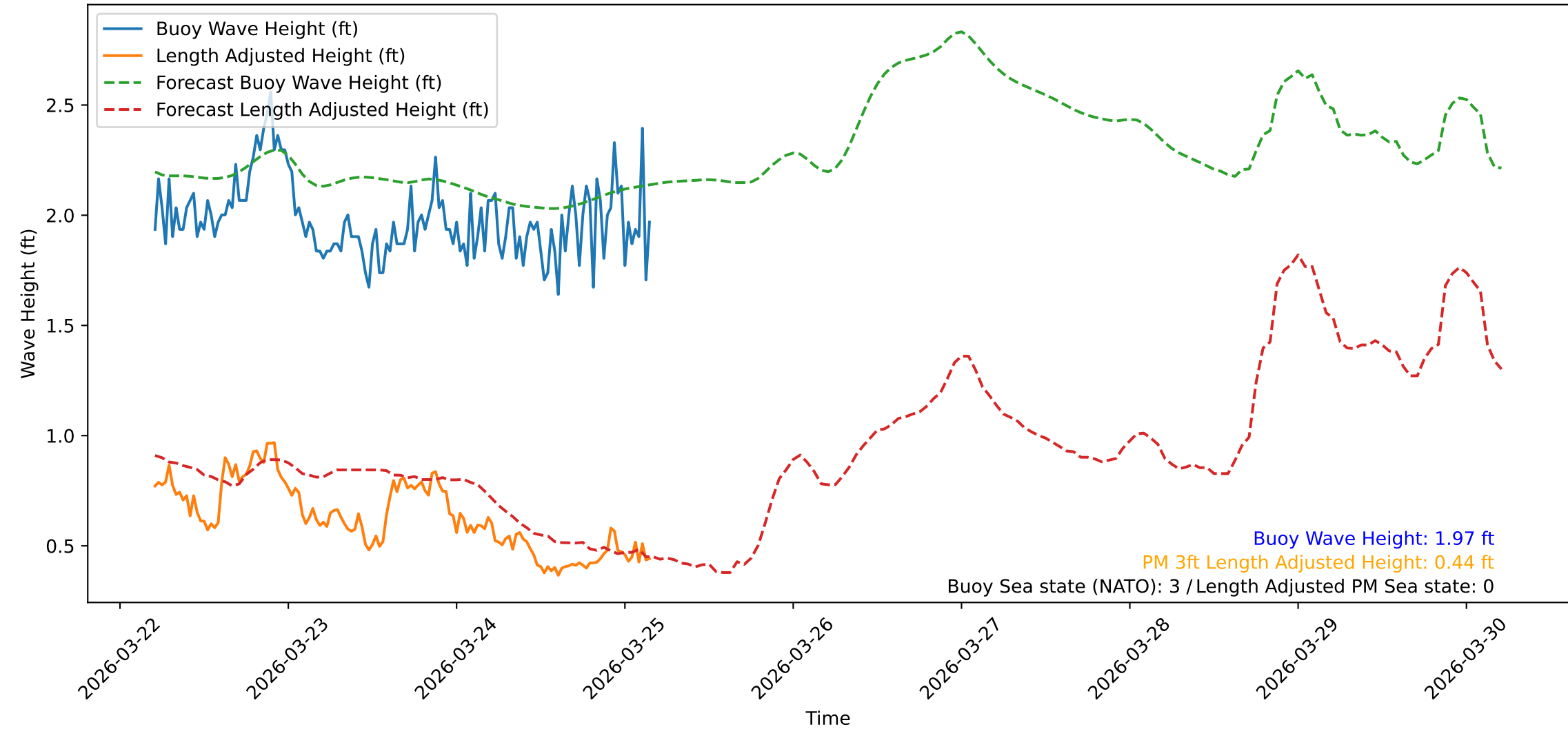
Wave Heights over Time for Red Beach at 2026-03-25 04:30:47
