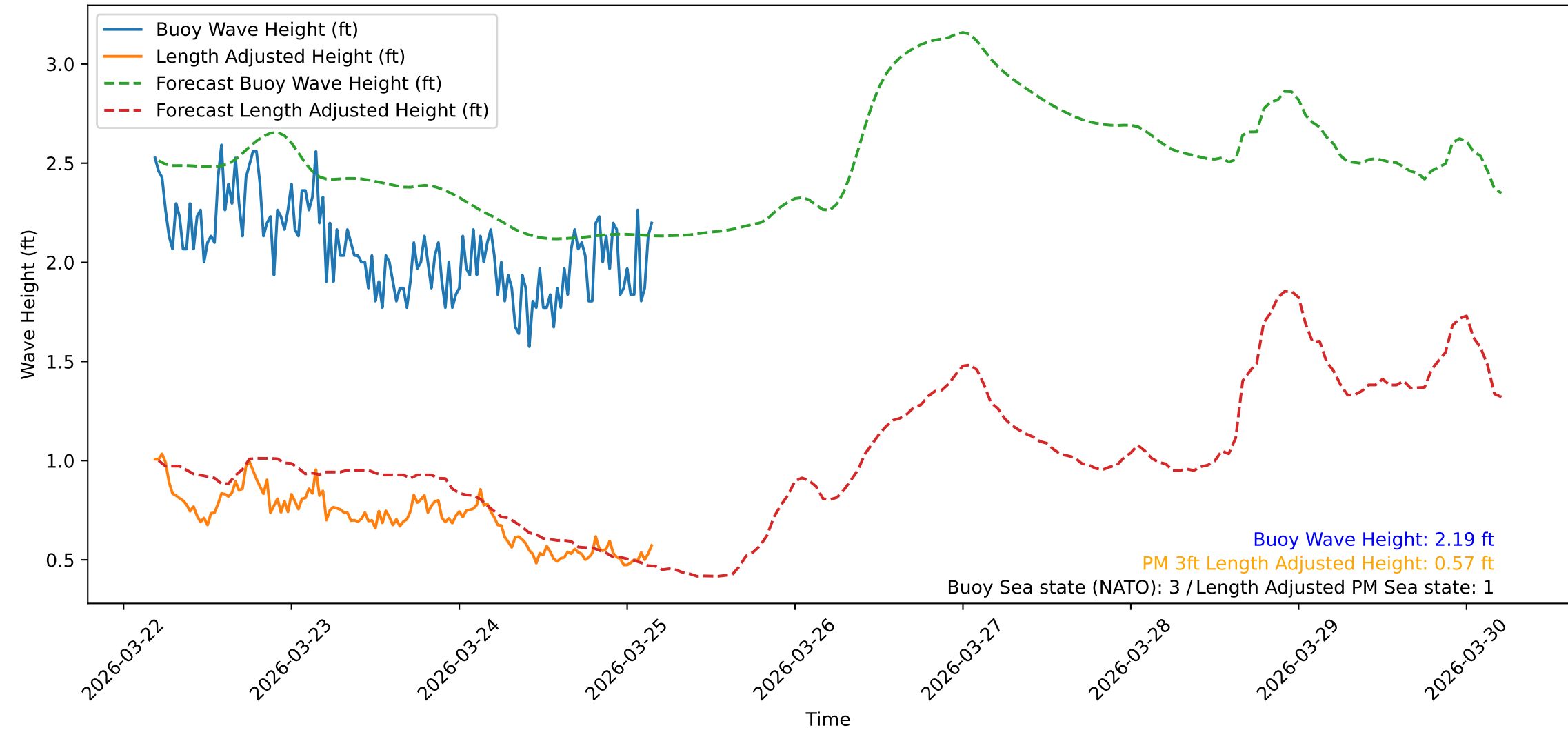
Wave Heights over Time for Oceanside Harbor at 2026-03-25 04:30:31
