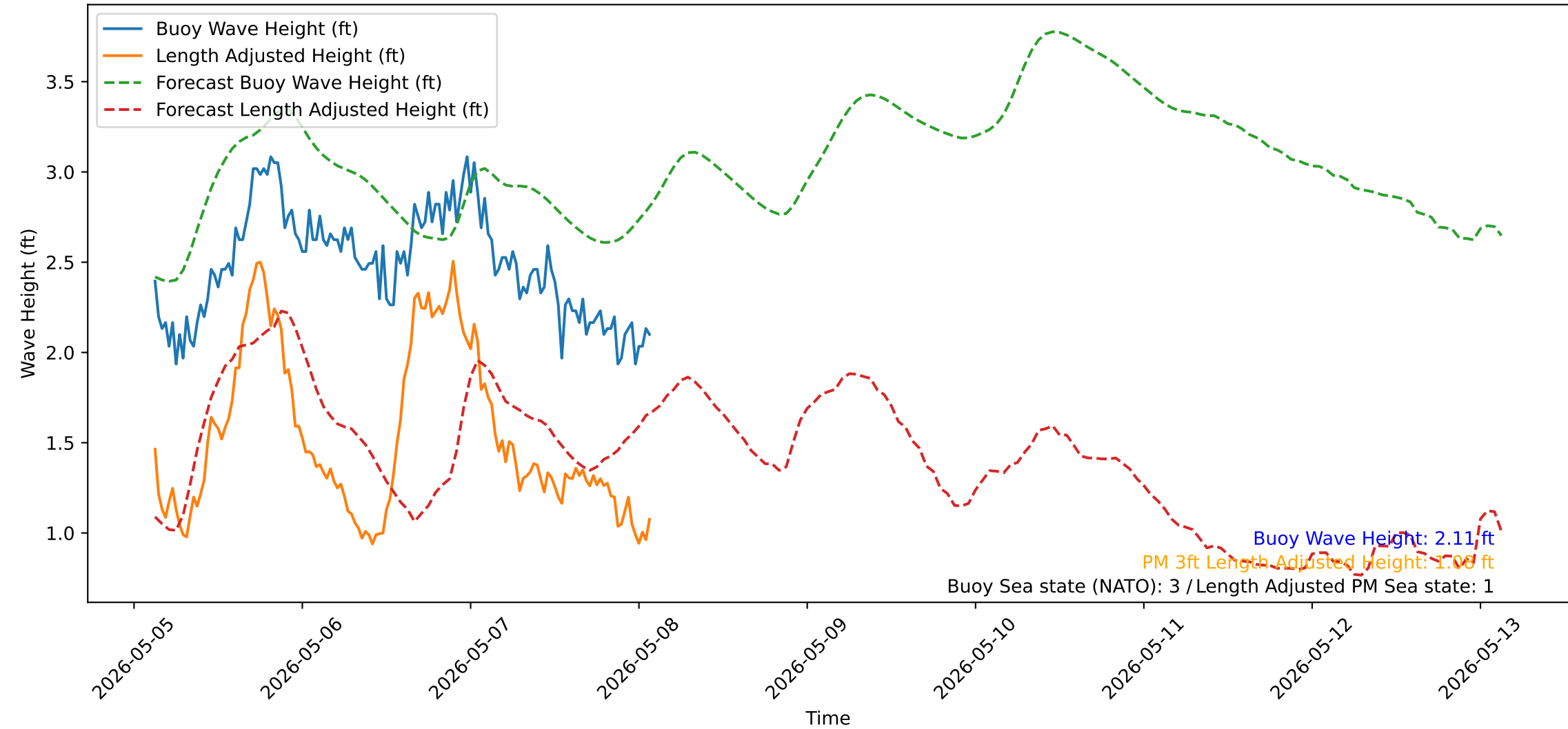
Wave Heights over Time for Red Beach at 2026-05-08 02:30:50
