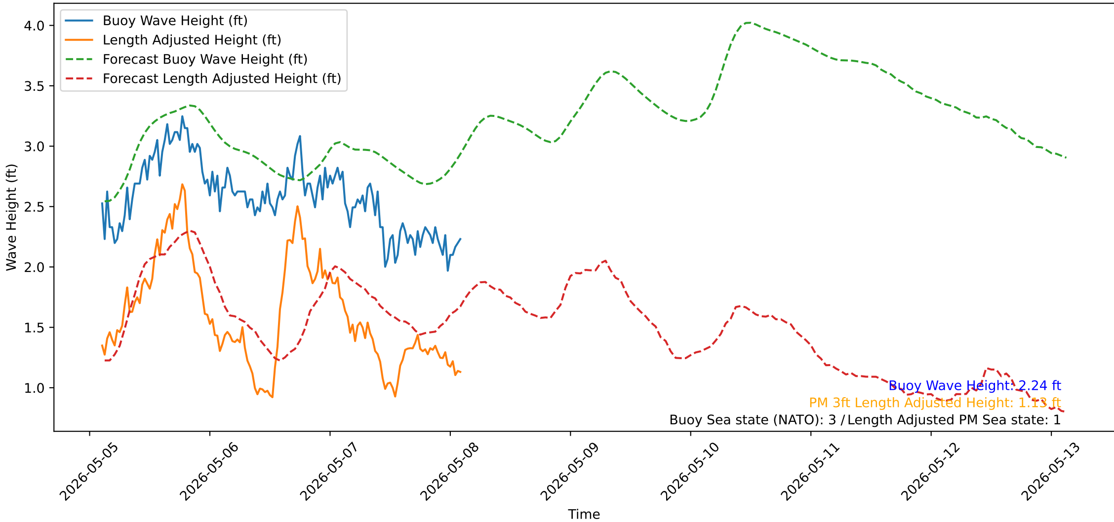
Wave Heights over Time for Oceanside Harbor at 2026-05-08 02:30:31
