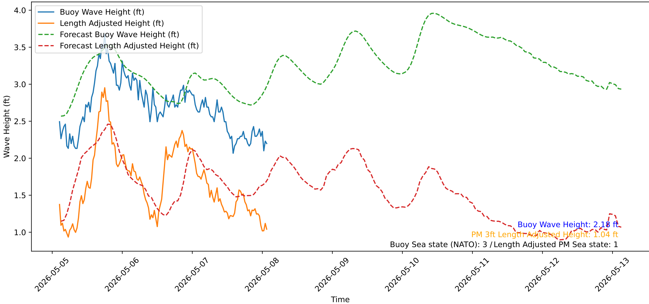
Wave Heights over Time for Green Beach at 2026-05-08 02:31:12
