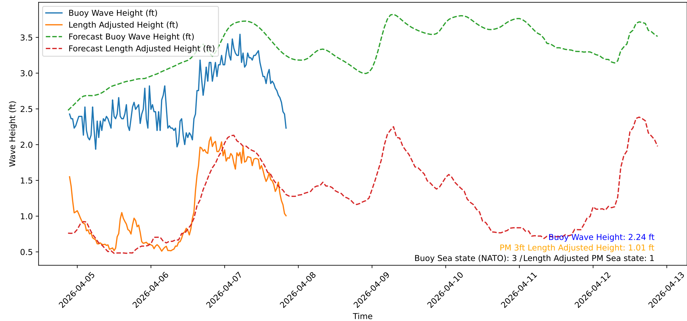
Wave Heights over Time for Red Beach at 2026-04-07 21:00:47
