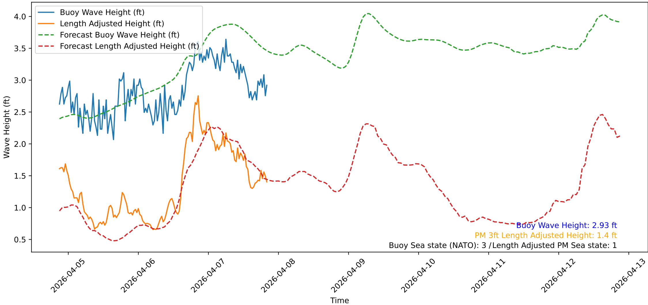
Wave Heights over Time for Oceanside Harbor at 2026-04-07 21:00:32
