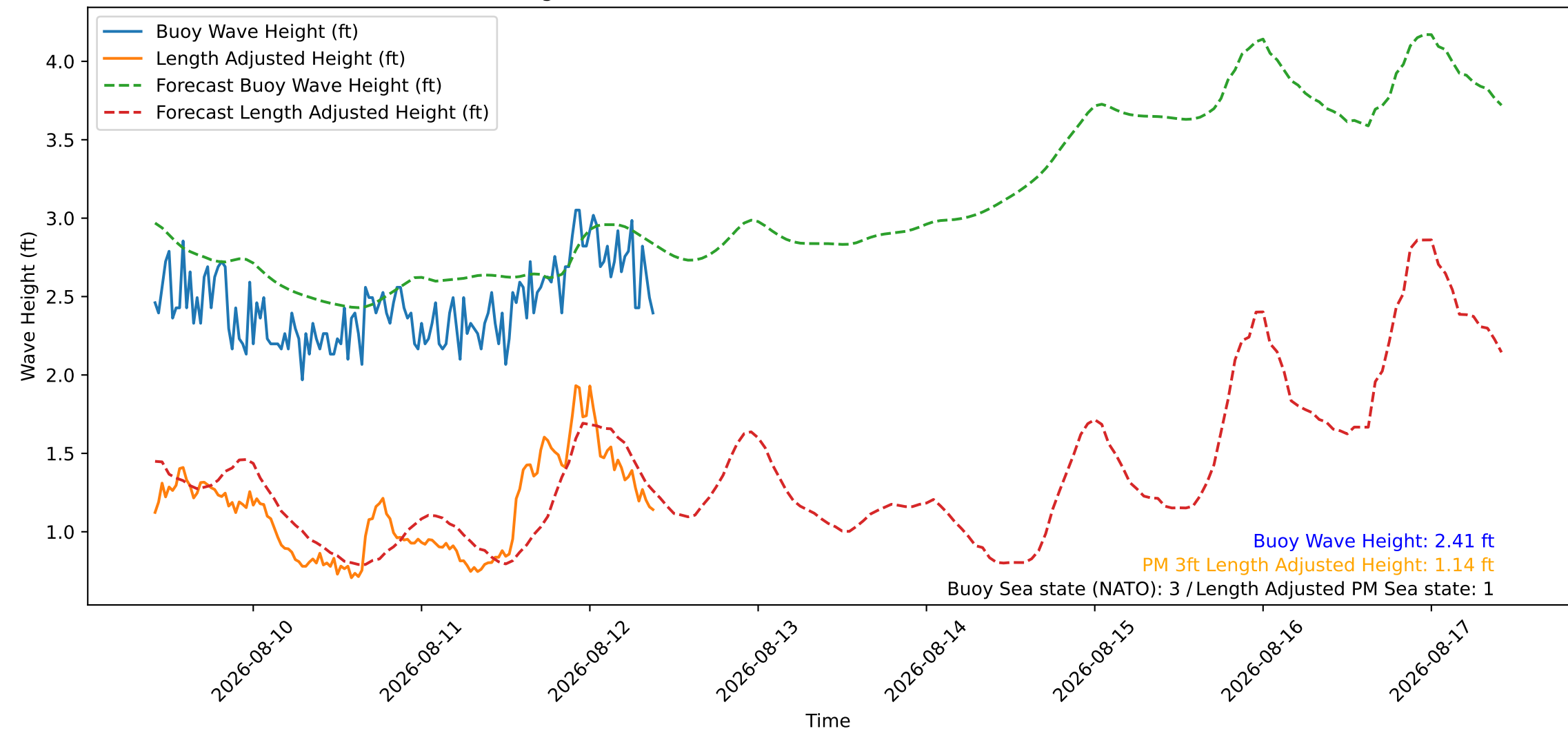
Wave Heights over Time for Oceanside Harbor at 2026-08-12 10:00:26
