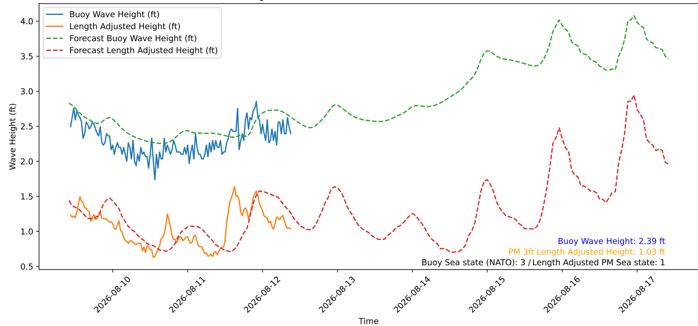
Wave Heights over Time for Red Beach at 2026-08-12 10:00:46
