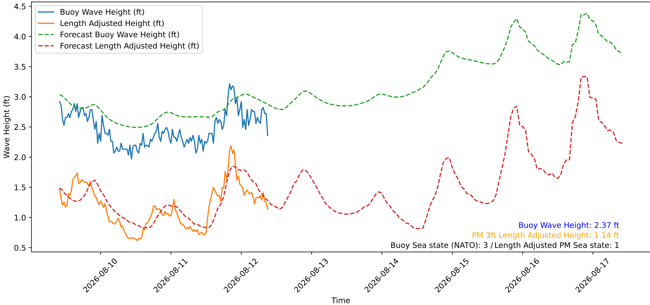
Wave Heights over Time for Green Beach at 2026-08-12 10:01:09
