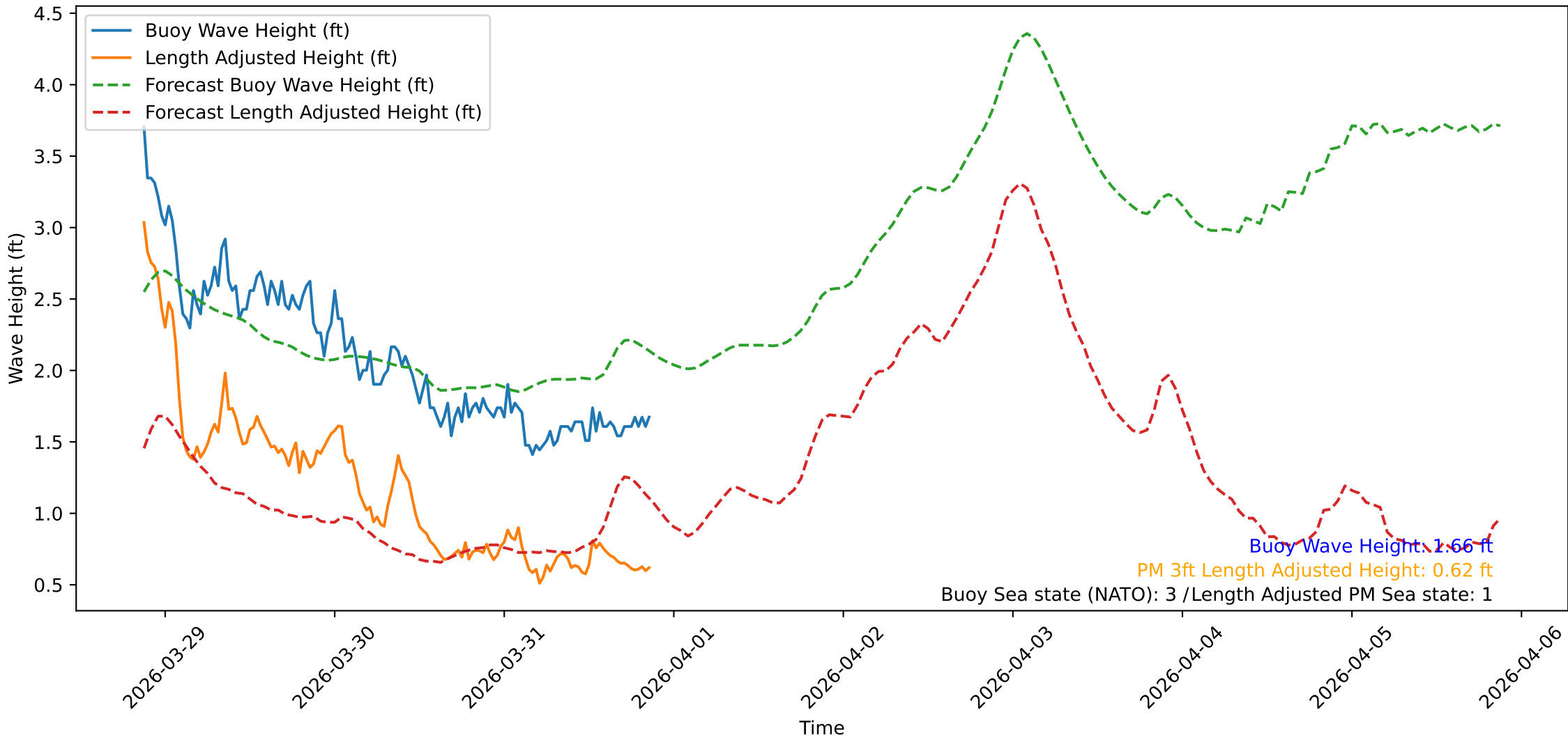
Wave Heights over Time for Green Beach at 2026-03-31 21:11:09
