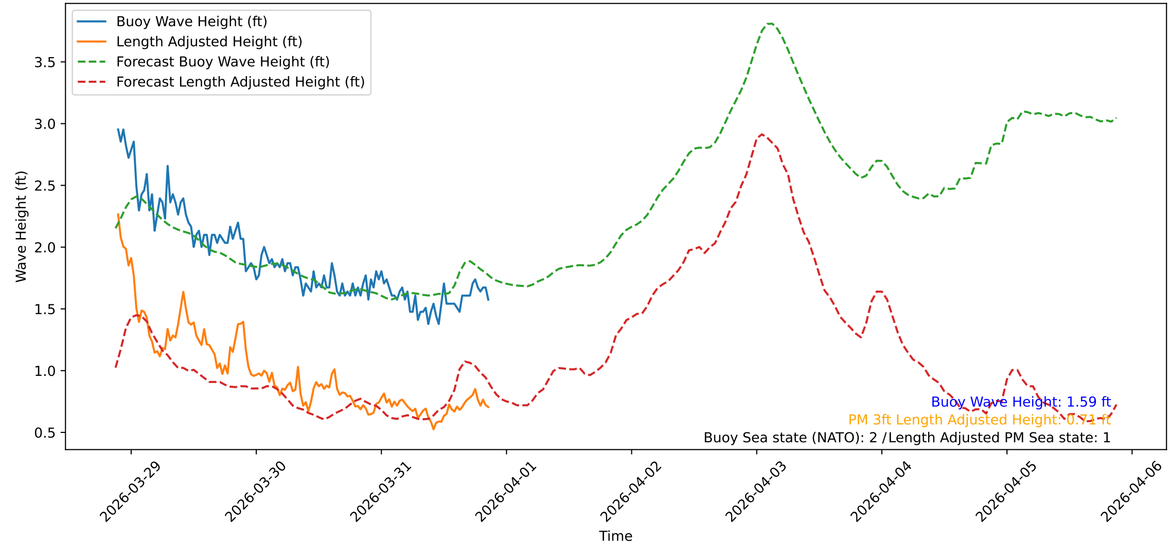
Wave Heights over Time for Red Beach at 2026-03-31 21:10:47
