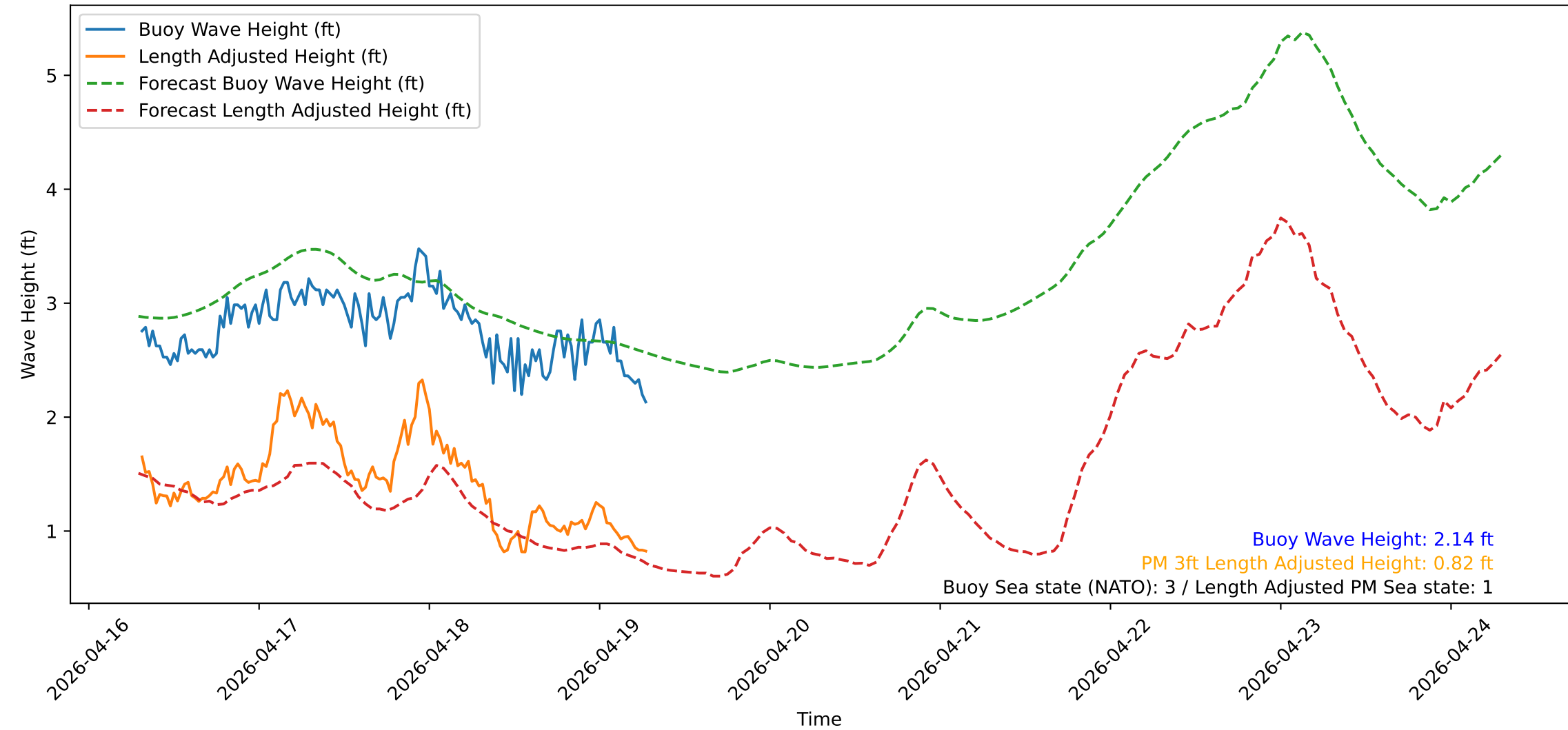
Wave Heights over Time for Green Beach at 2026-04-19 07:21:13
