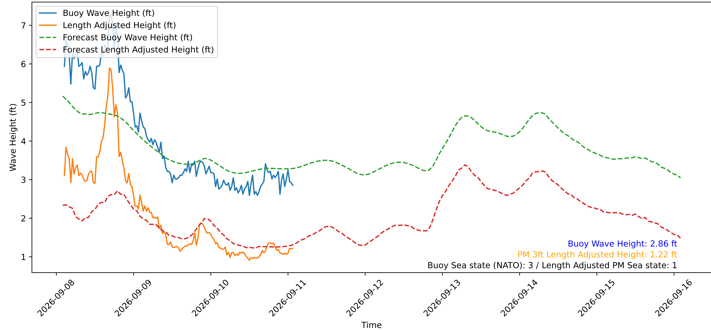
Wave Heights over Time for Green Beach at 2026-09-11 02:11:12
