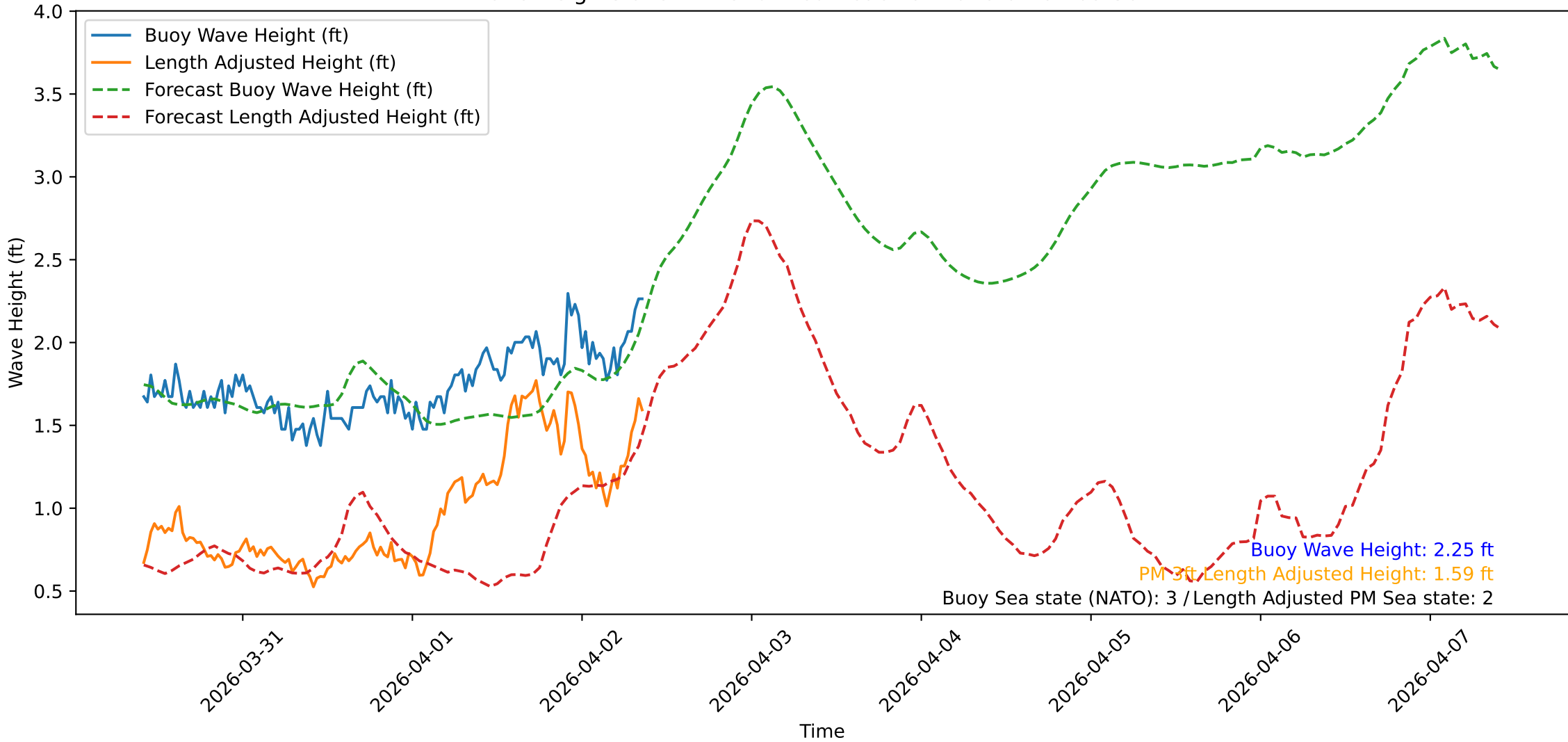
Wave Heights over Time for Red Beach at 2026-04-02 09:30:47
