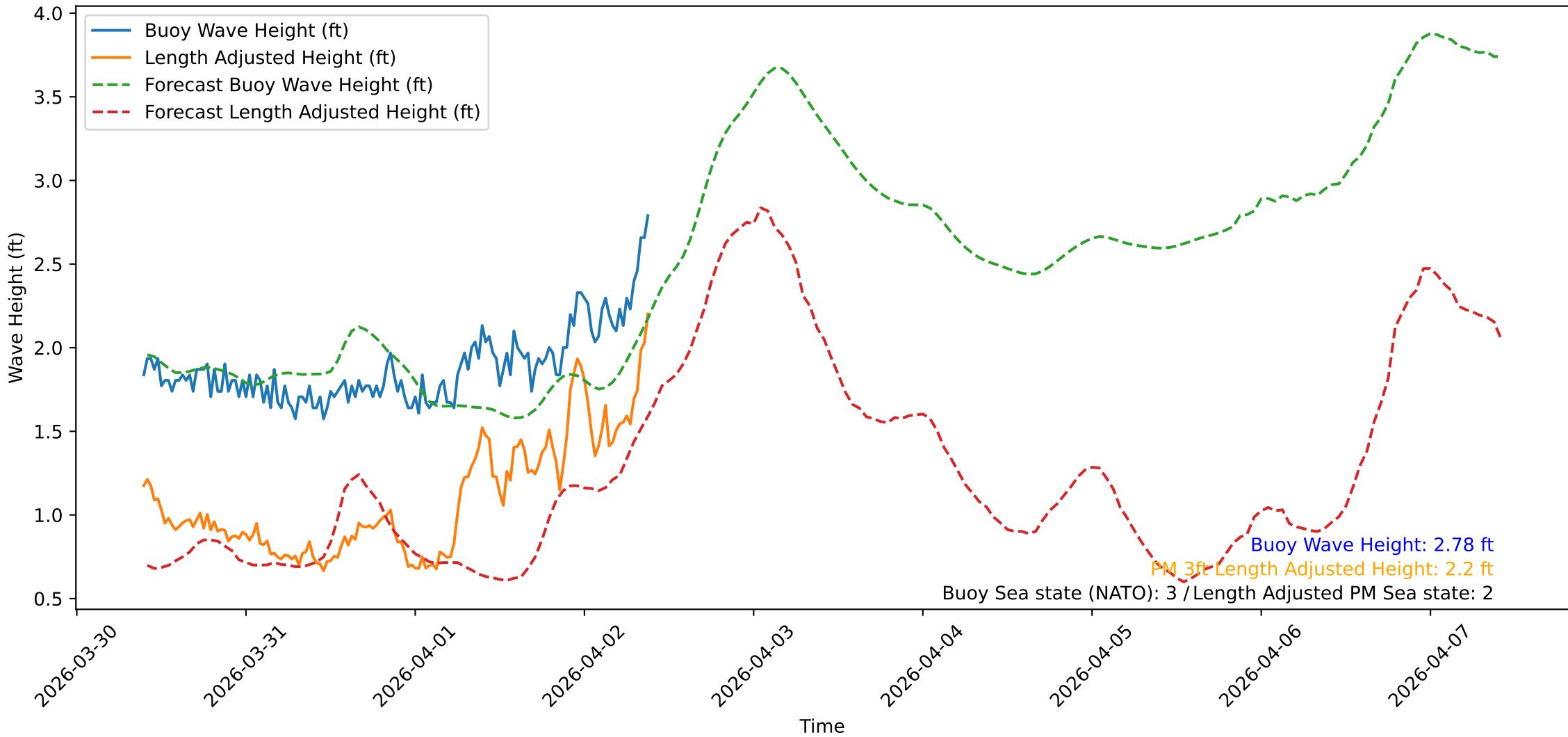
Wave Heights over Time for Oceanside Harbor at 2026-04-02 09:30:31
