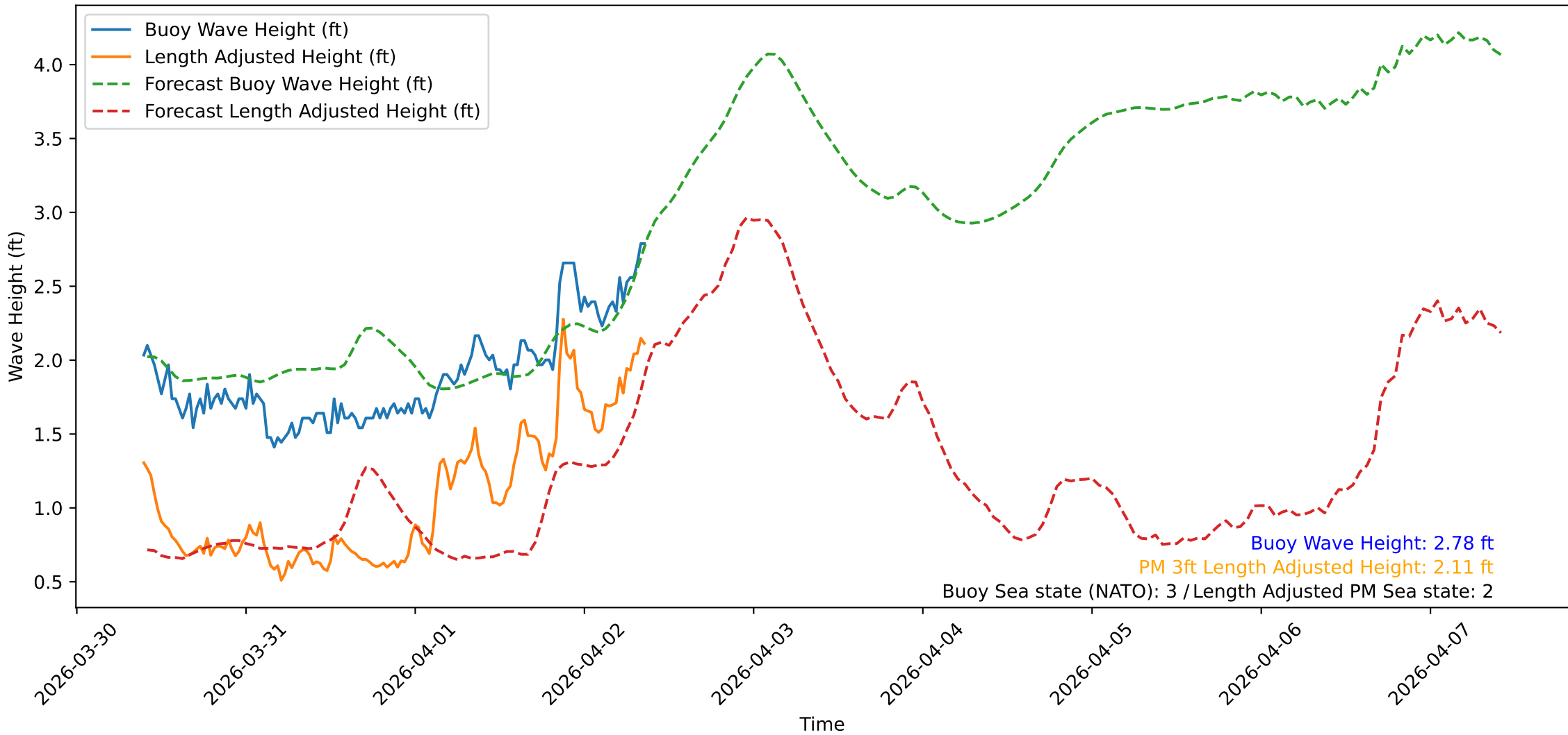
Wave Heights over Time for Green Beach at 2026-04-02 09:31:11
