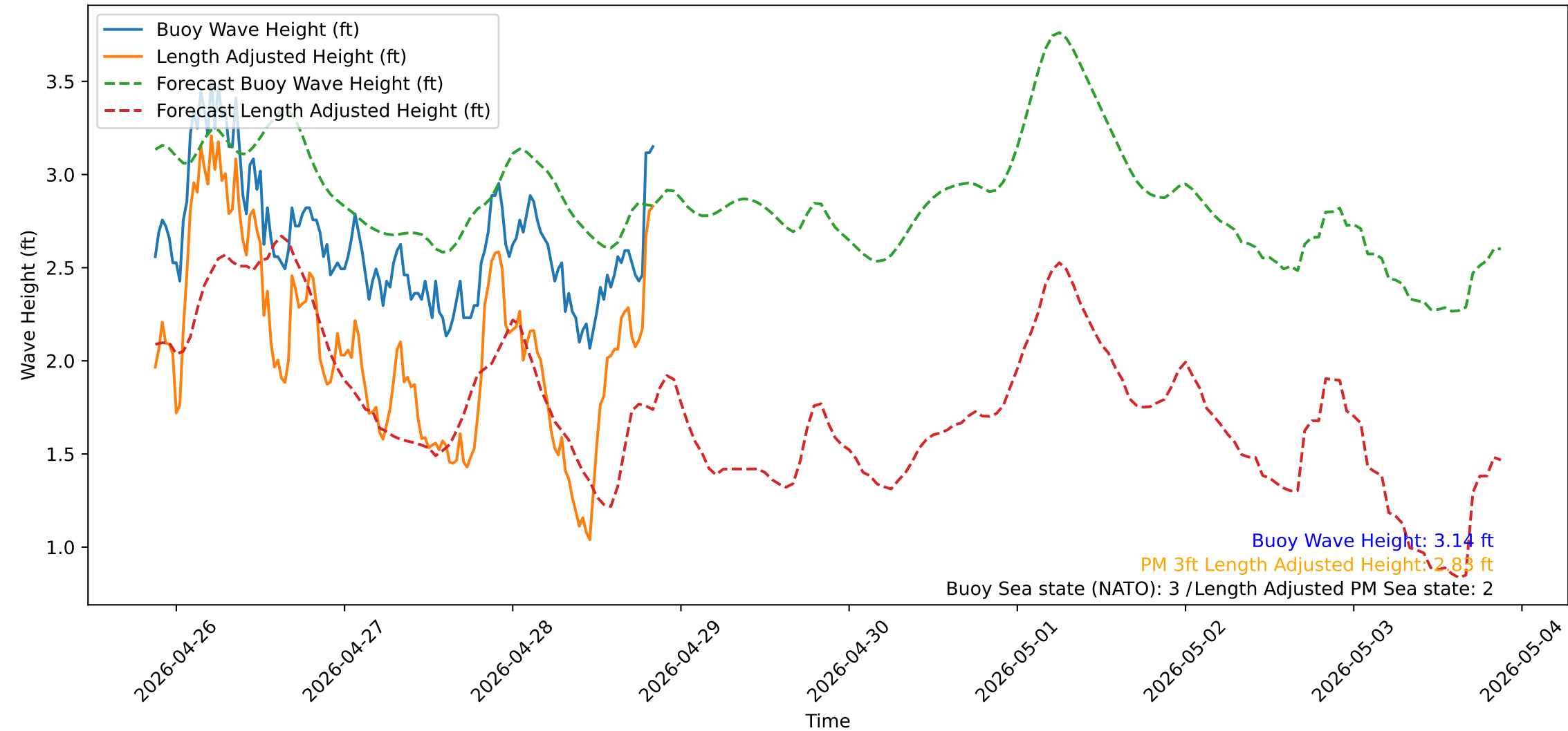
Wave Heights over Time for Green Beach at 2026-04-28 20:51:14
