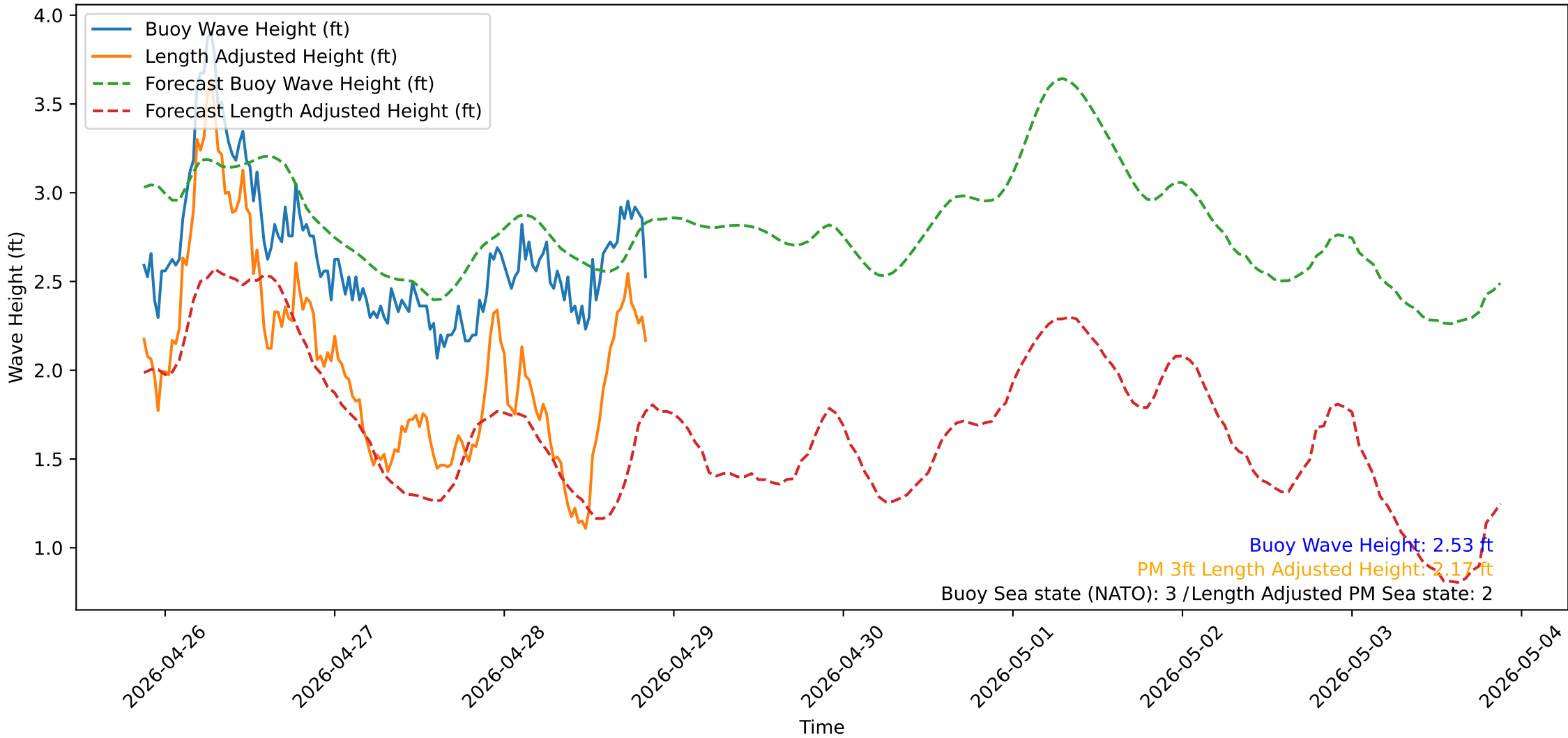
Wave Heights over Time for Oceanside Harbor at 2026-04-28 20:50:31
