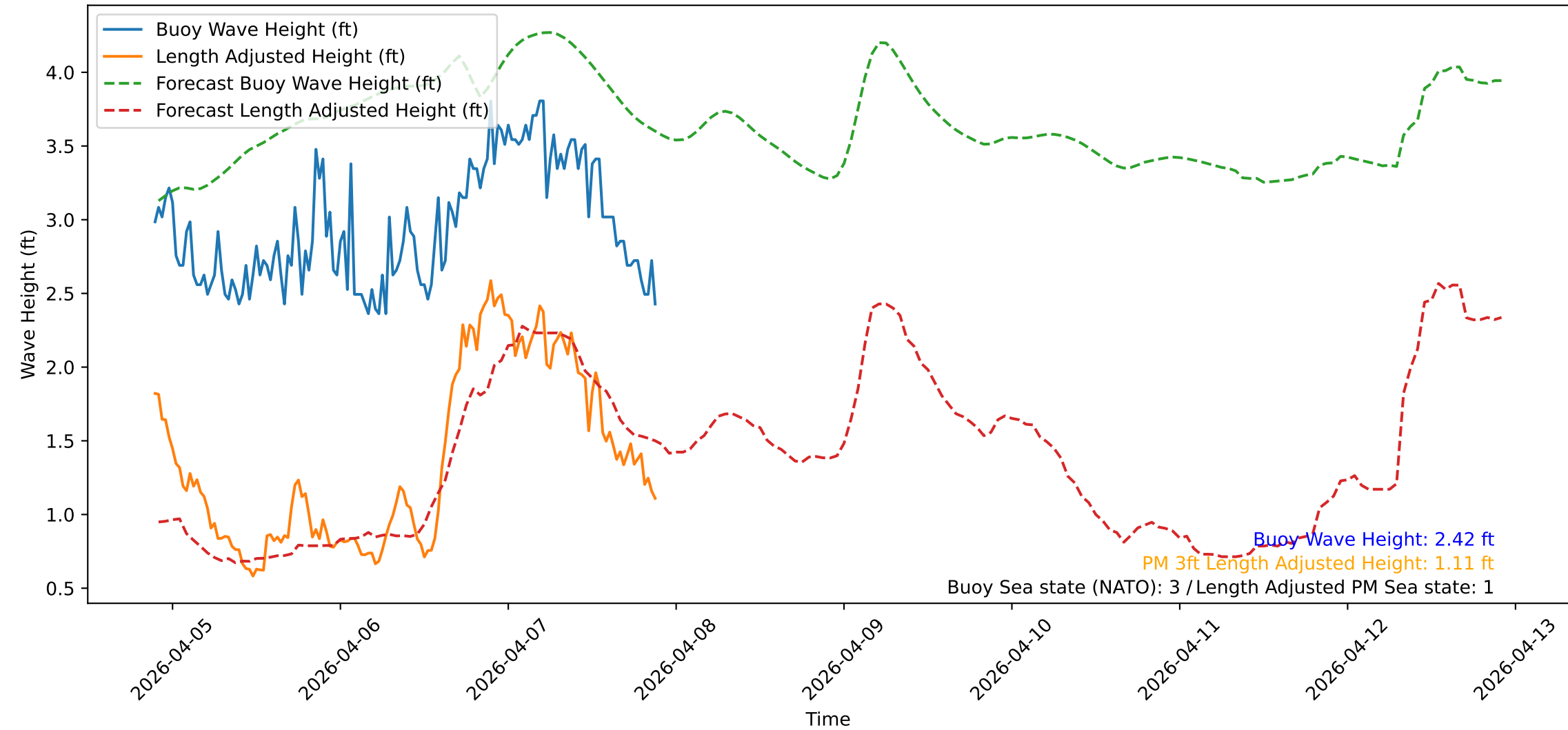
Wave Heights over Time for Green Beach at 2026-04-07 21:41:10
