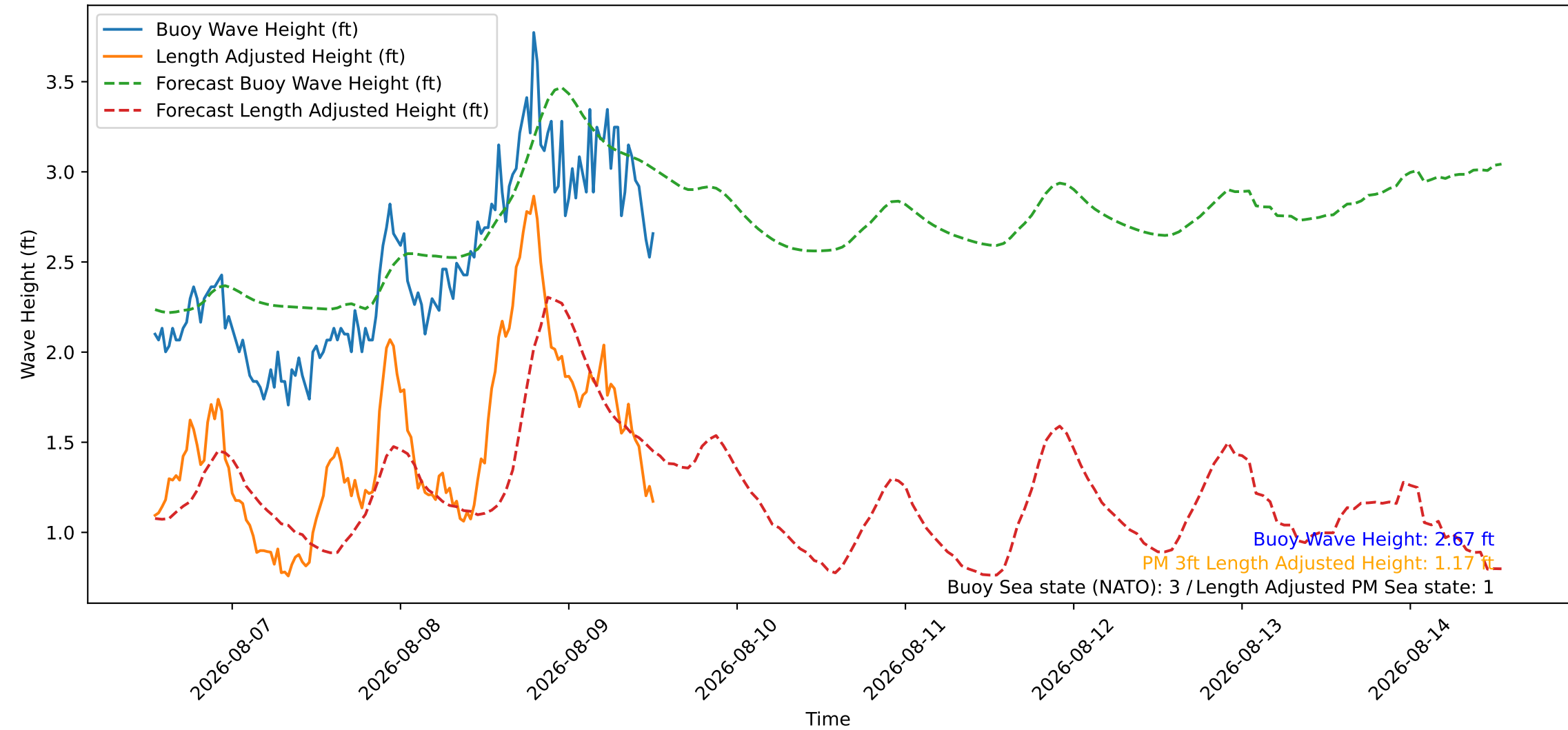
Wave Heights over Time for Green Beach at 2026-08-09 13:01:08
