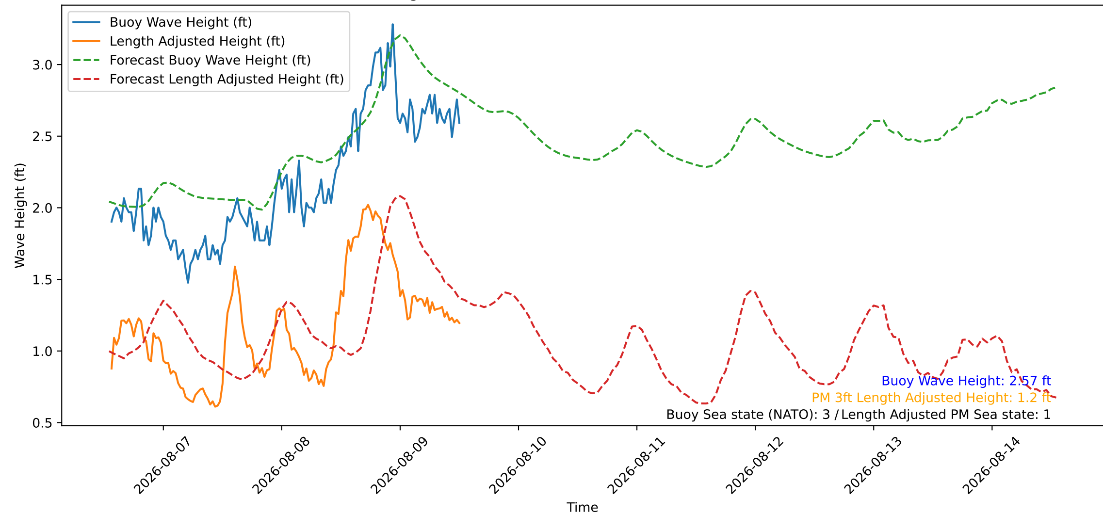
Wave Heights over Time for Red Beach at 2026-08-09 13:00:46
