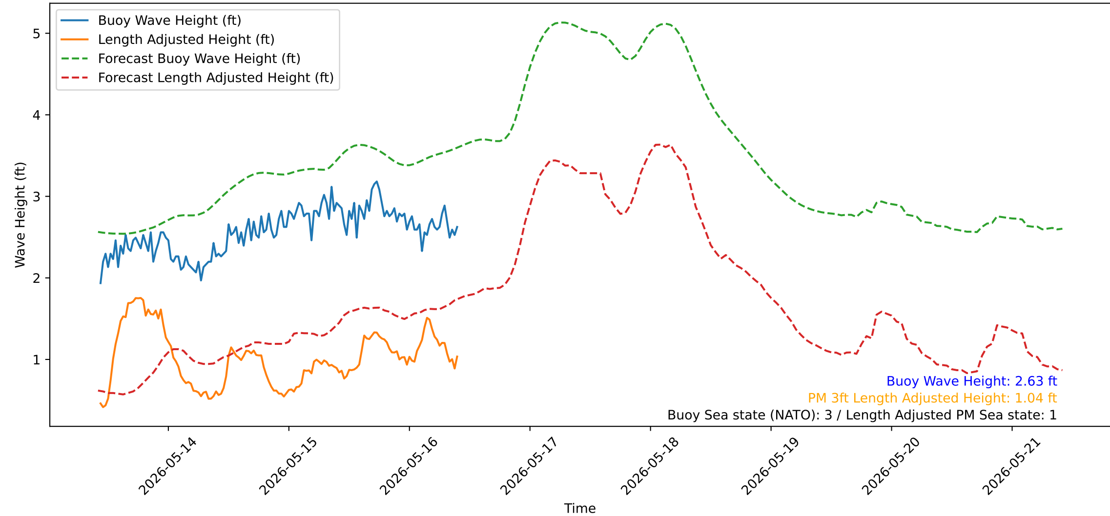
Wave Heights over Time for Red Beach at 2026-05-16 10:20:52
