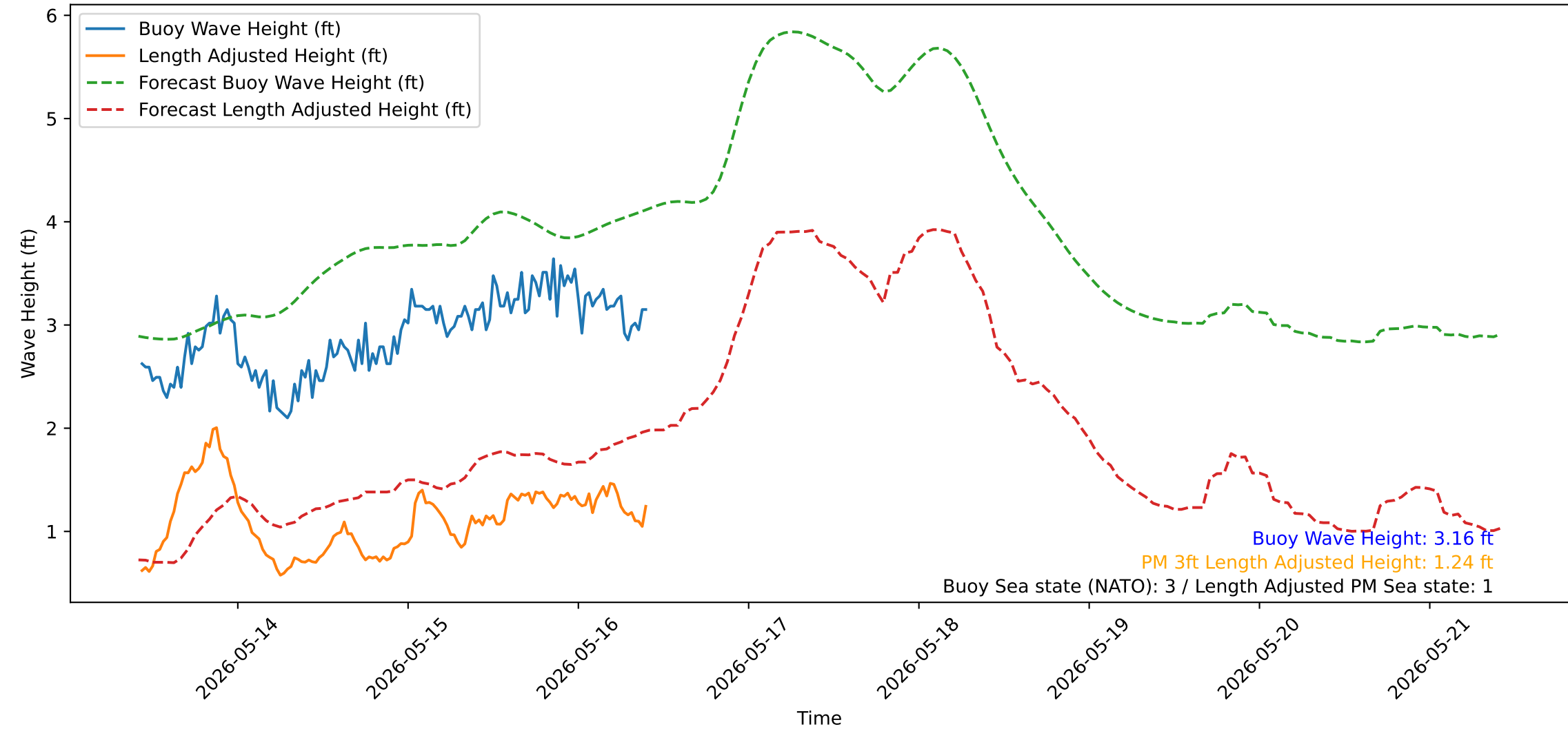
Wave Heights over Time for Green Beach at 2026-05-16 10:21:14
