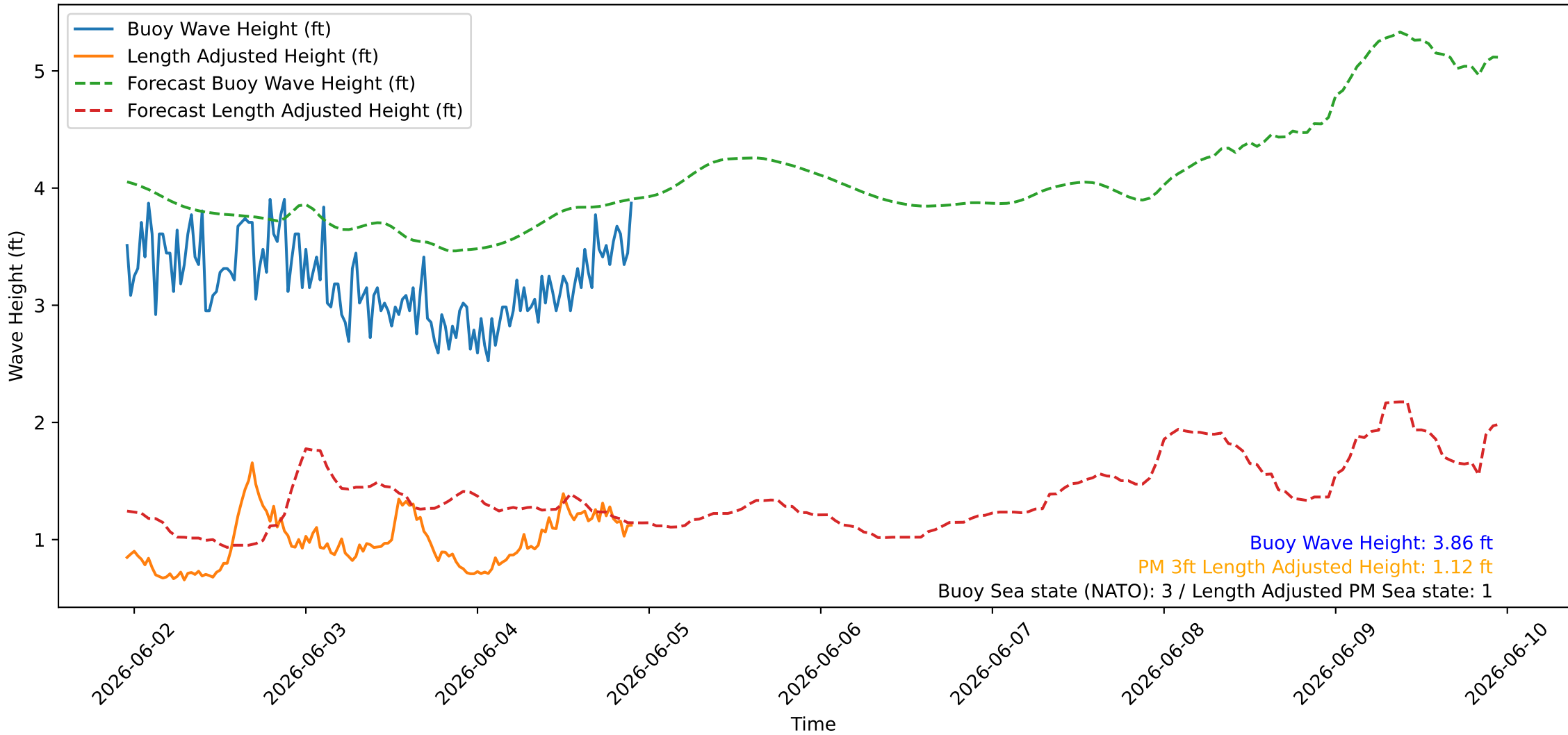
Wave Heights over Time for Red Beach at 2026-06-04 22:30:45
