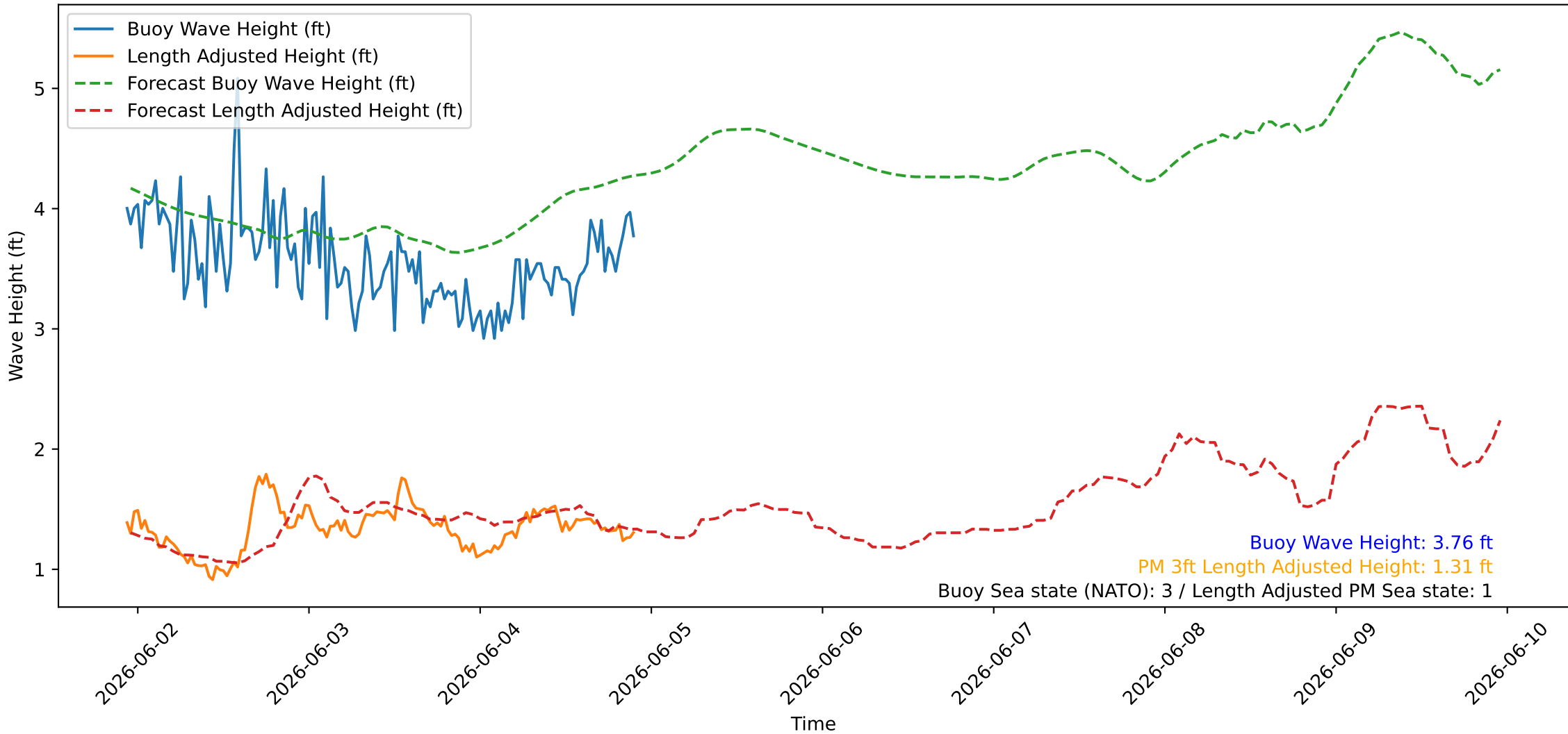
Wave Heights over Time for Oceanside Harbor at 2026-06-04 22:30:26
