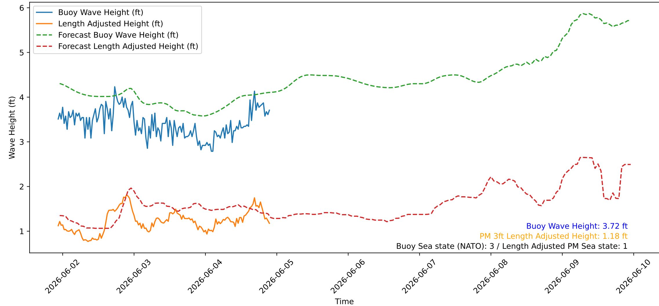
Wave Heights over Time for Green Beach at 2026-06-04 22:31:07
