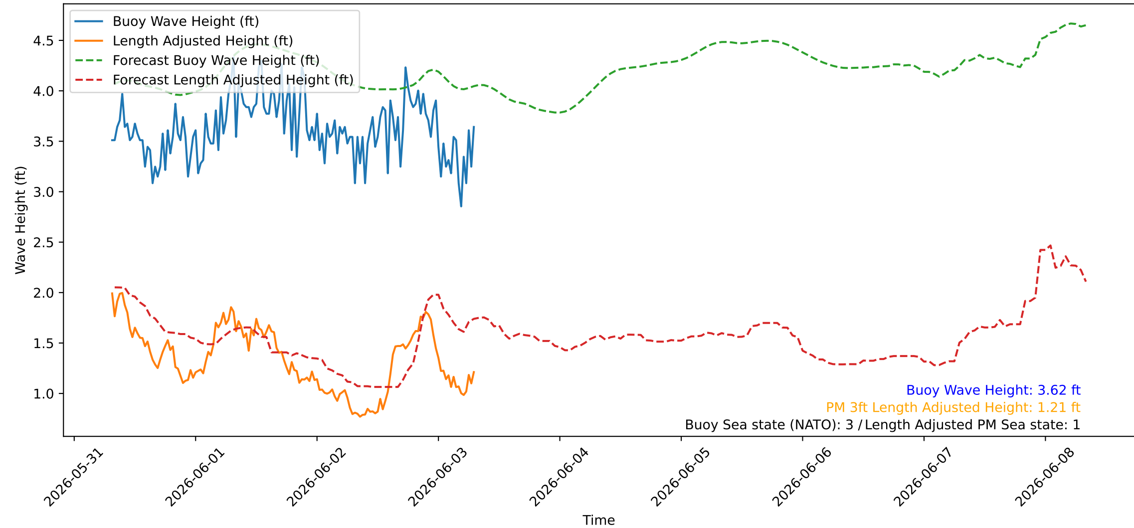
Wave Heights over Time for Green Beach at 2026-06-03 07:41:09
