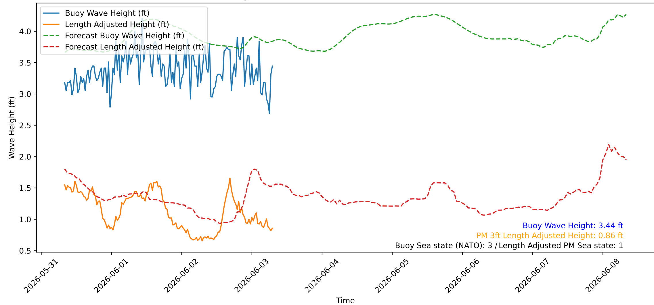
Wave Heights over Time for Red Beach at 2026-06-03 07:40:46
