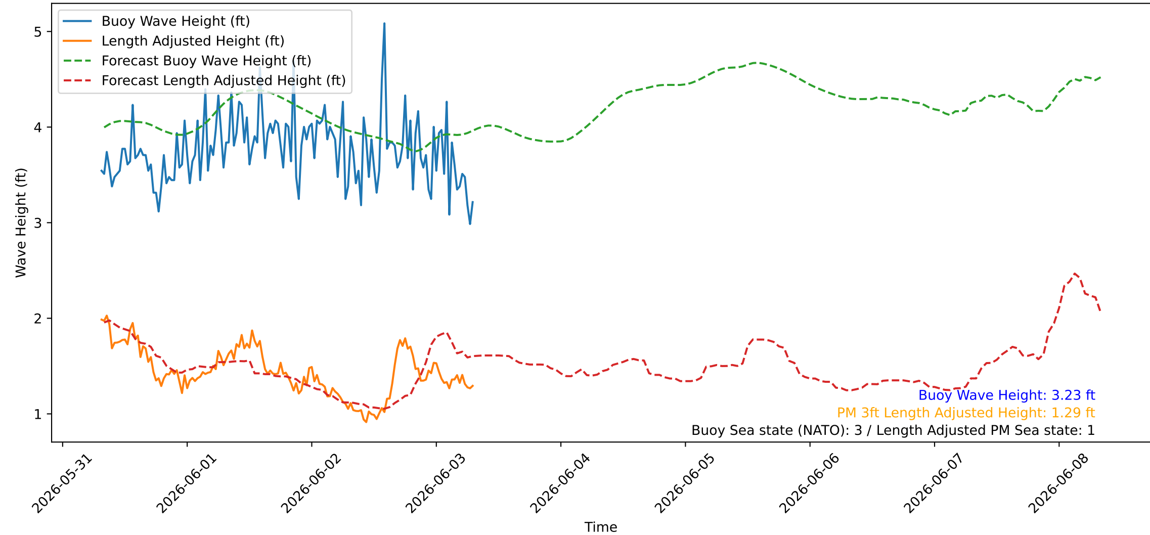
Wave Heights over Time for Oceanside Harbor at 2026-06-03 07:40:26
