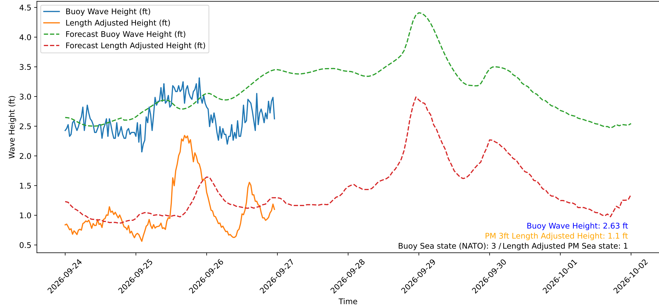
Wave Heights over Time for Red Beach at 2026-09-26 23:50:50
