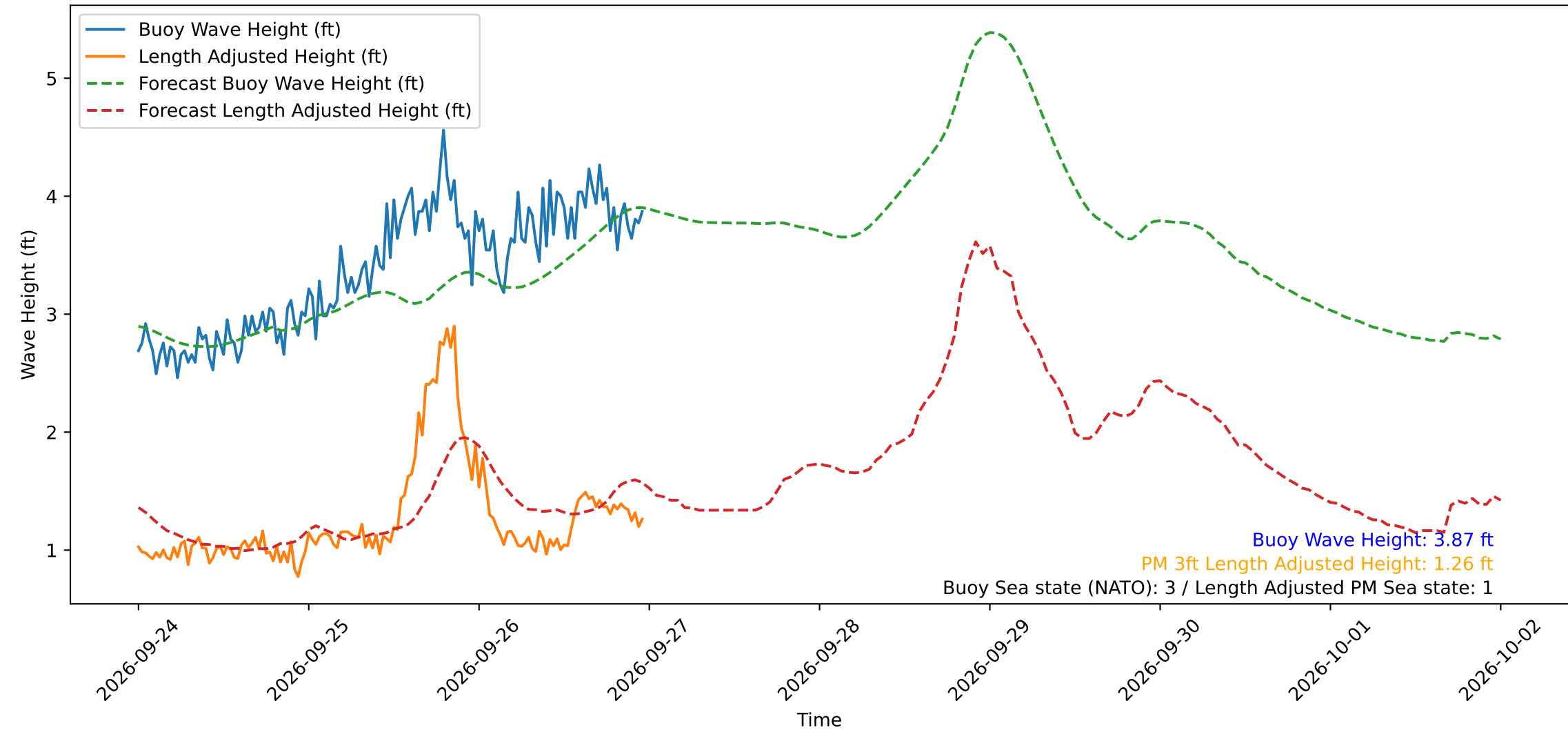
Wave Heights over Time for Green Beach at 2026-09-26 23:51:15
