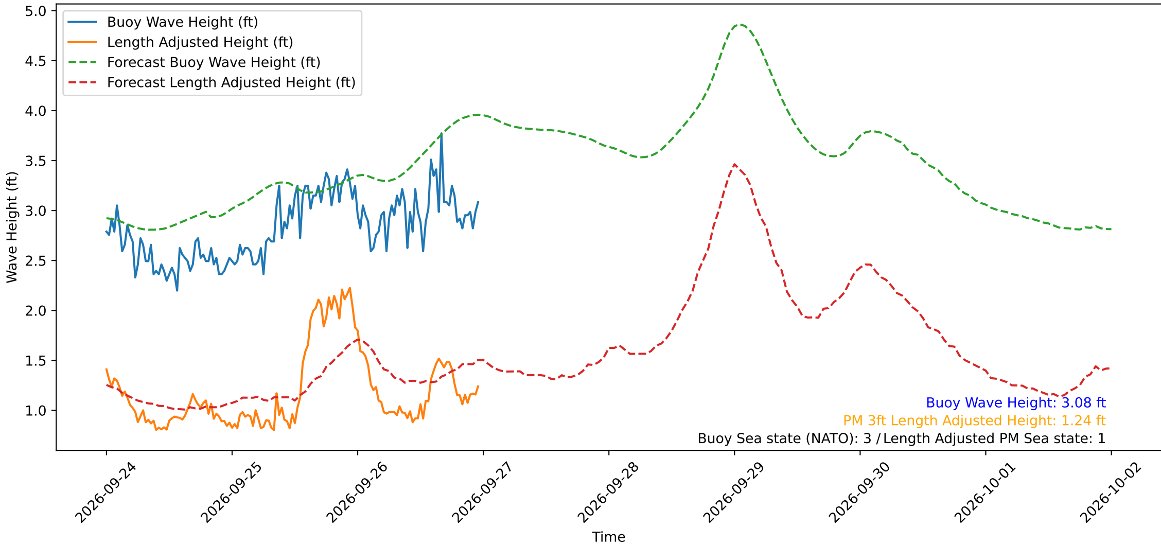
Wave Heights over Time for Oceanside Harbor at 2026-09-26 23:50:29
