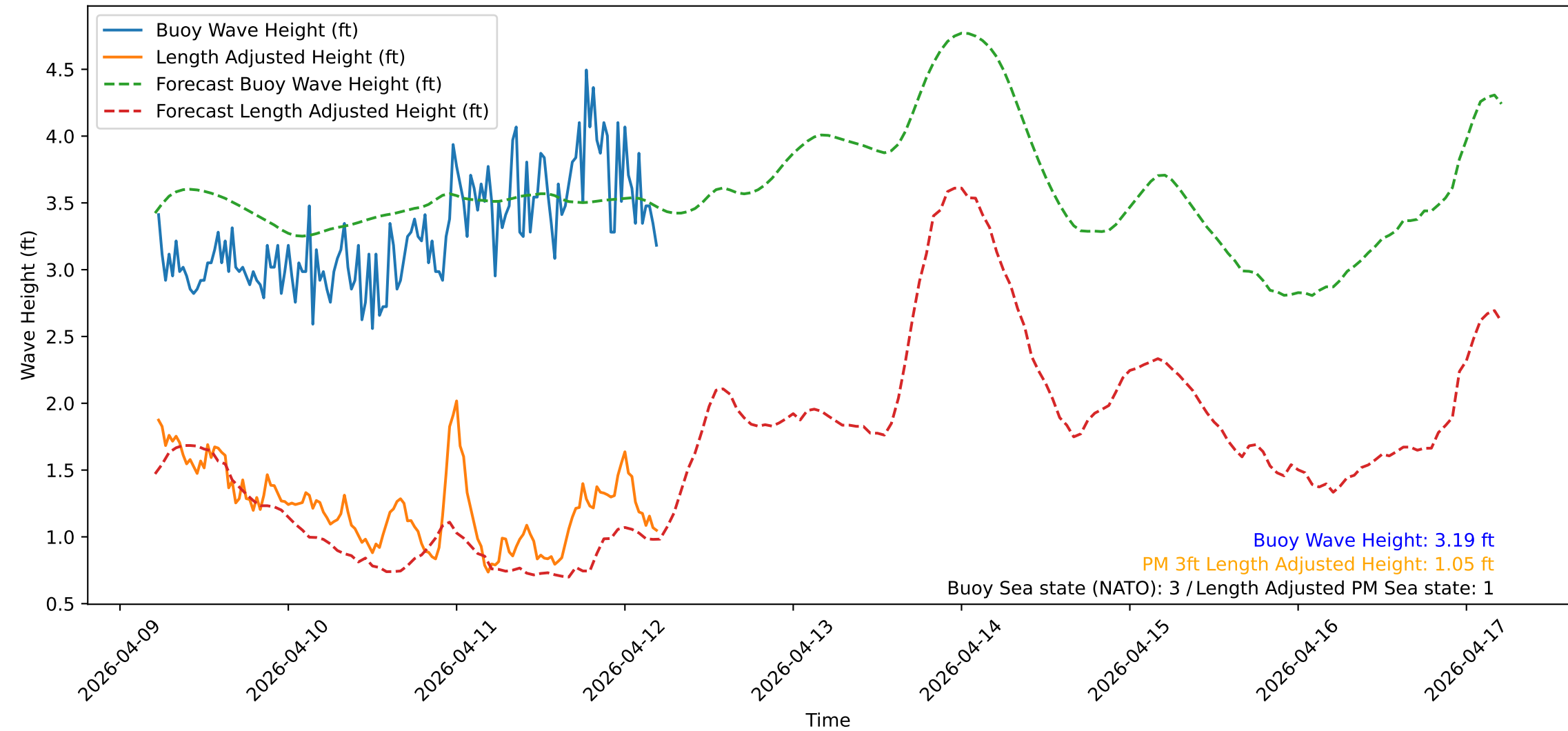
Wave Heights over Time for Green Beach at 2026-04-12 05:21:14
