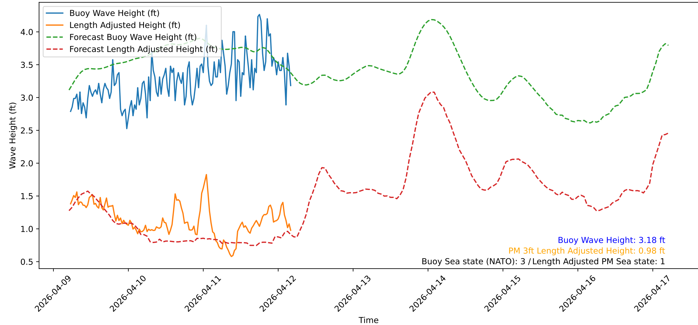
Wave Heights over Time for Red Beach at 2026-04-12 05:20:51
