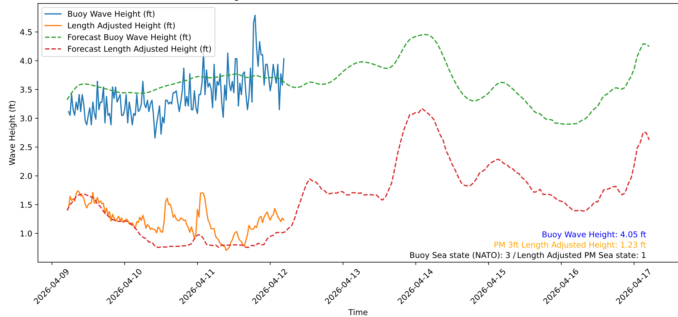
Wave Heights over Time for Oceanside Harbor at 2026-04-12 05:20:31
