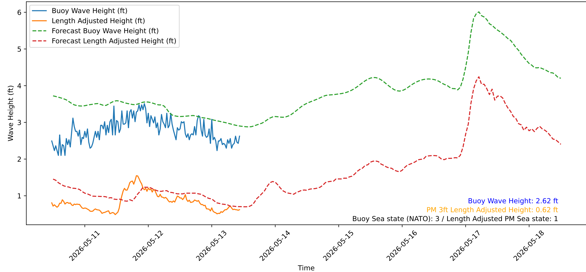
Wave Heights over Time for Green Beach at 2026-05-13 11:31:15
