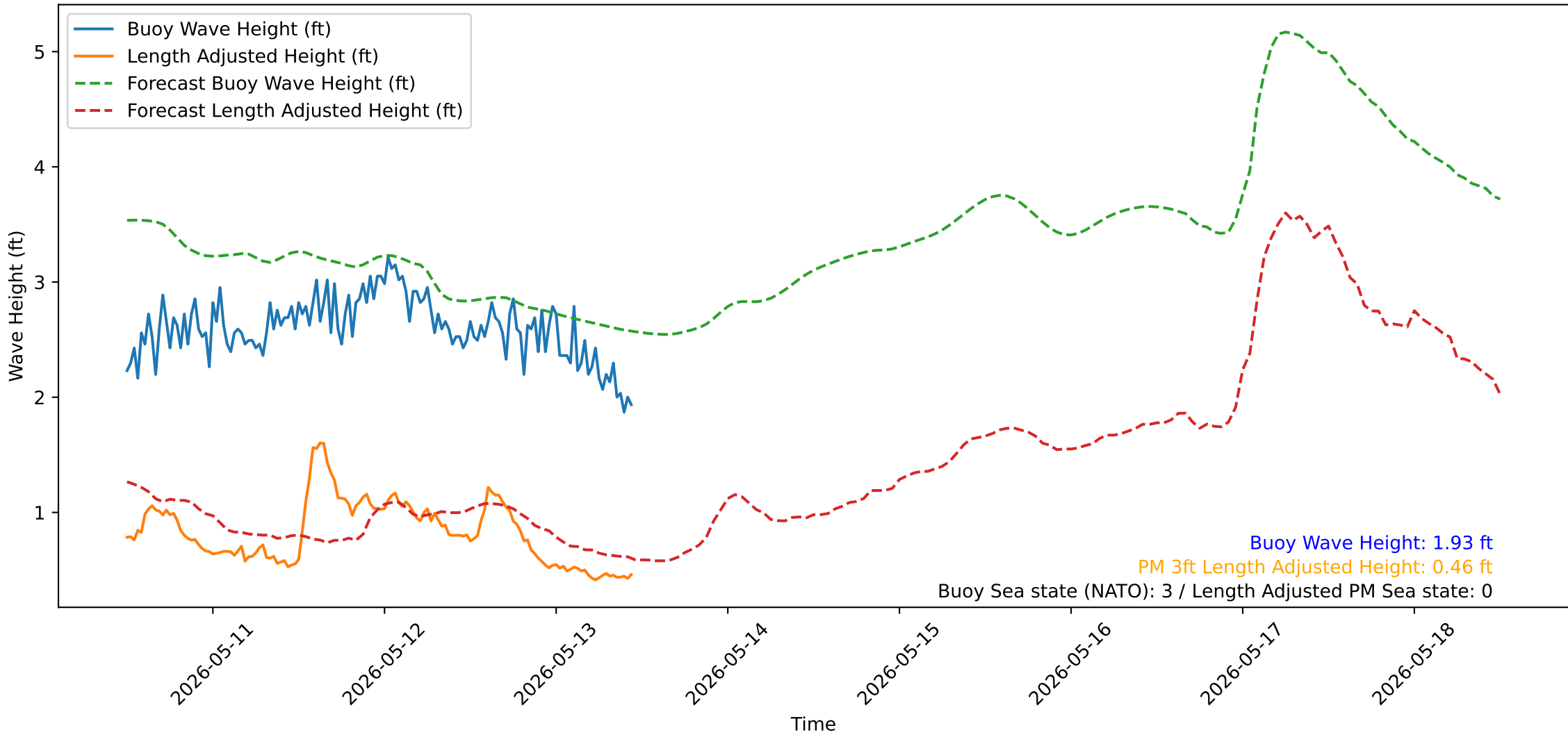
Wave Heights over Time for Red Beach at 2026-05-13 11:30:52
