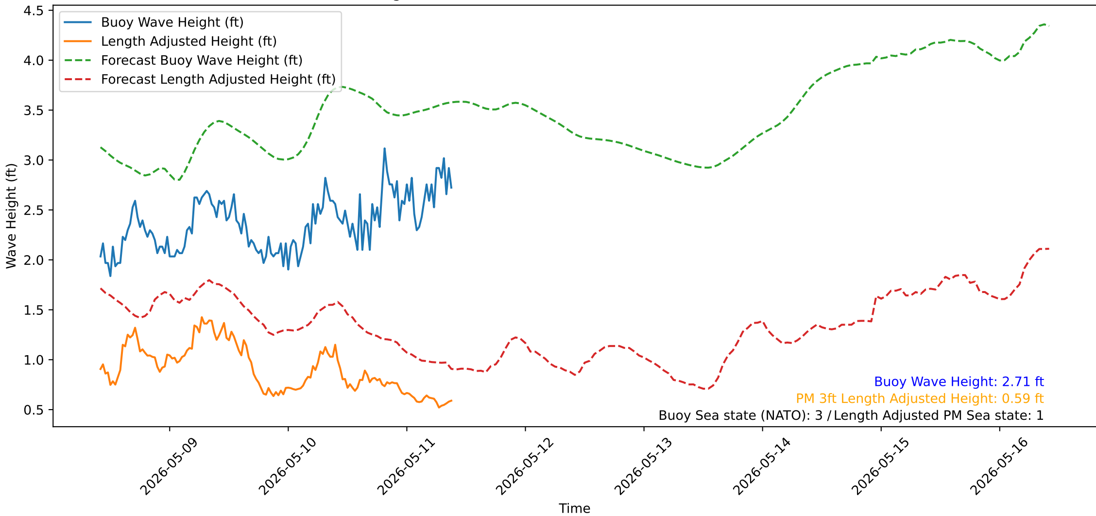
Wave Heights over Time for Green Beach at 2026-05-11 09:51:14
