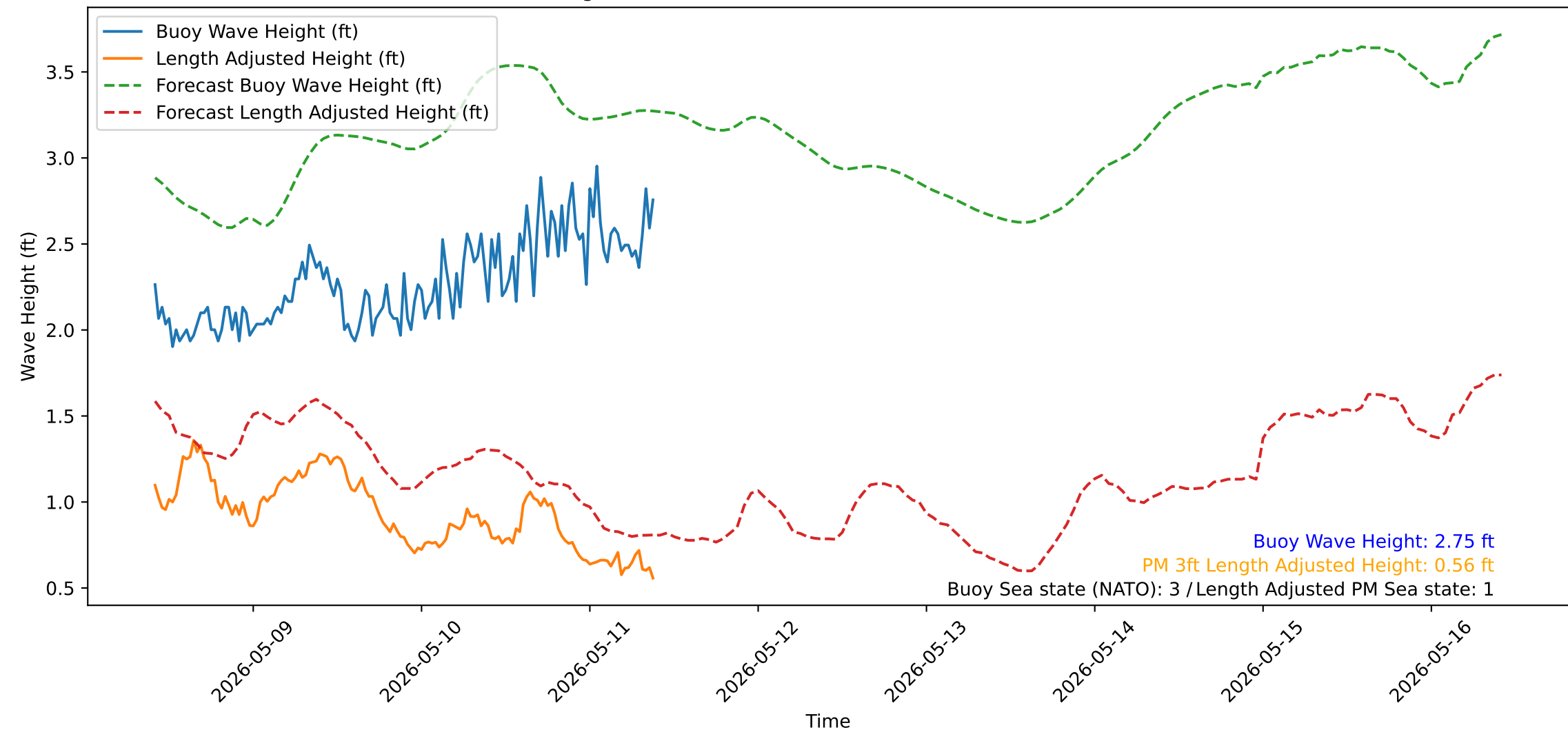
Wave Heights over Time for Red Beach at 2026-05-11 09:50:52
