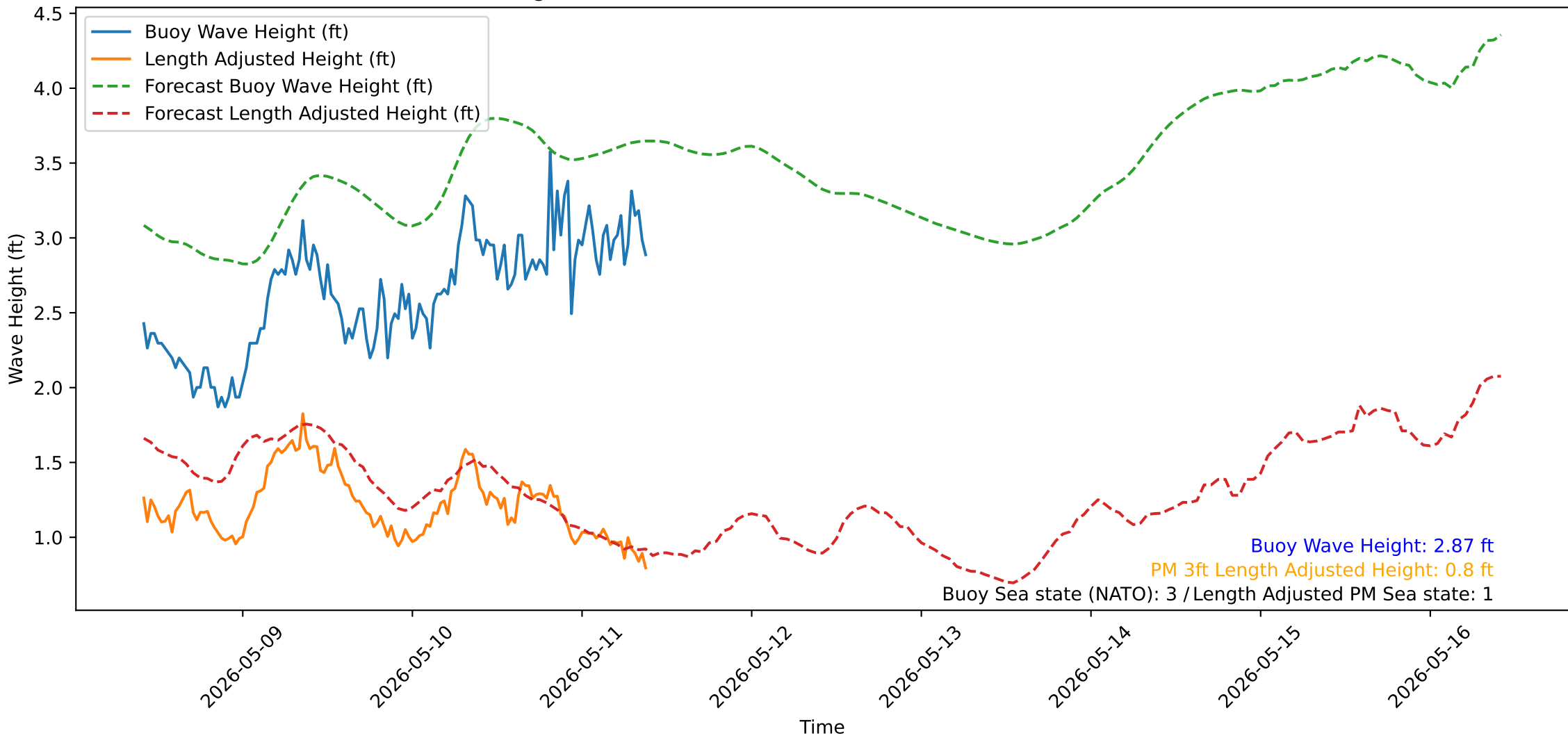
Wave Heights over Time for Oceanside Harbor at 2026-05-11 09:50:32
