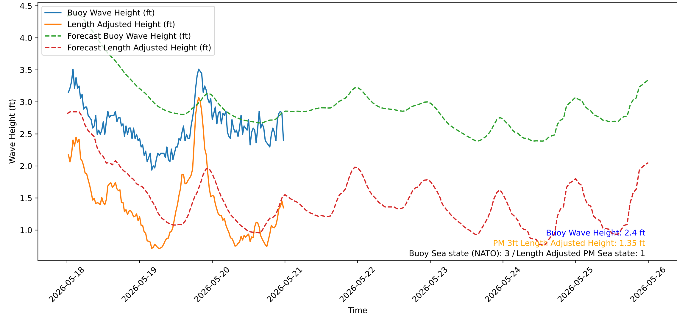
Wave Heights over Time for Red Beach at 2026-05-21 00:10:51
