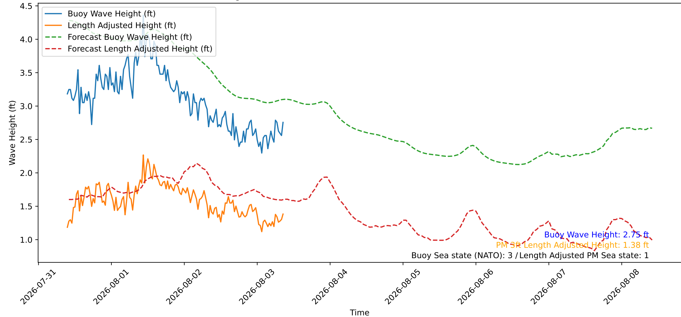
Wave Heights over Time for Oceanside Harbor at 2026-08-03 09:30:26
