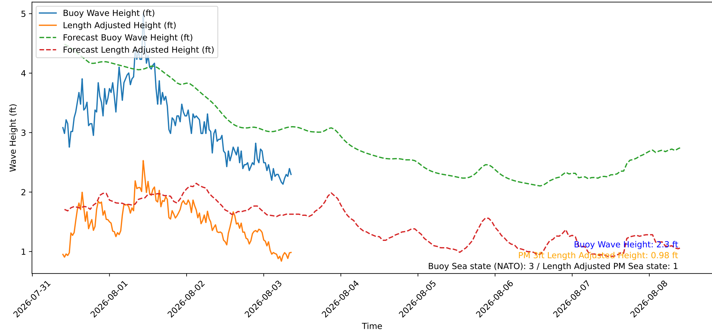
Wave Heights over Time for Green Beach at 2026-08-03 09:31:08
