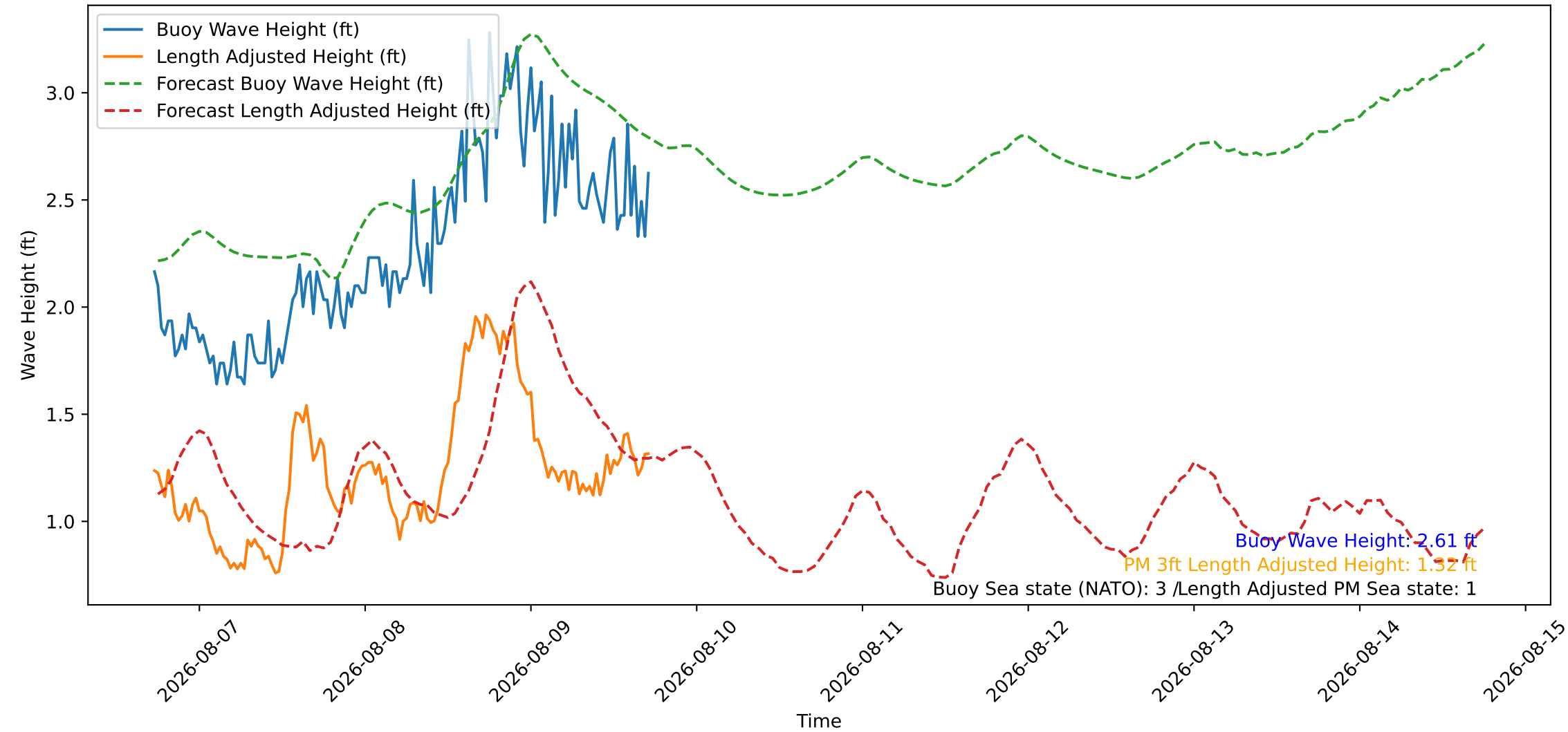
Wave Heights over Time for Oceanside Harbor at 2026-08-09 17:40:26
