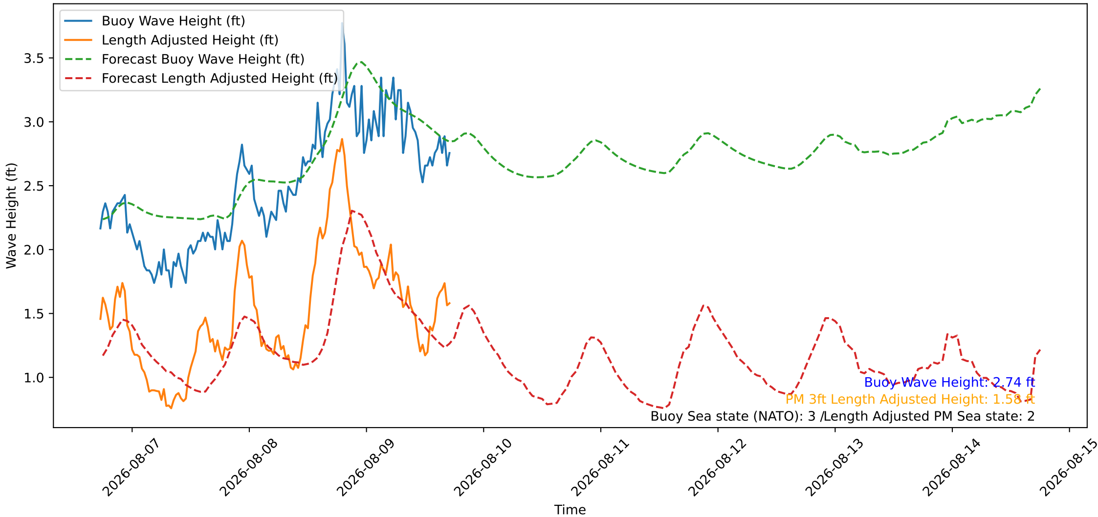
Wave Heights over Time for Green Beach at 2026-08-09 17:41:07
