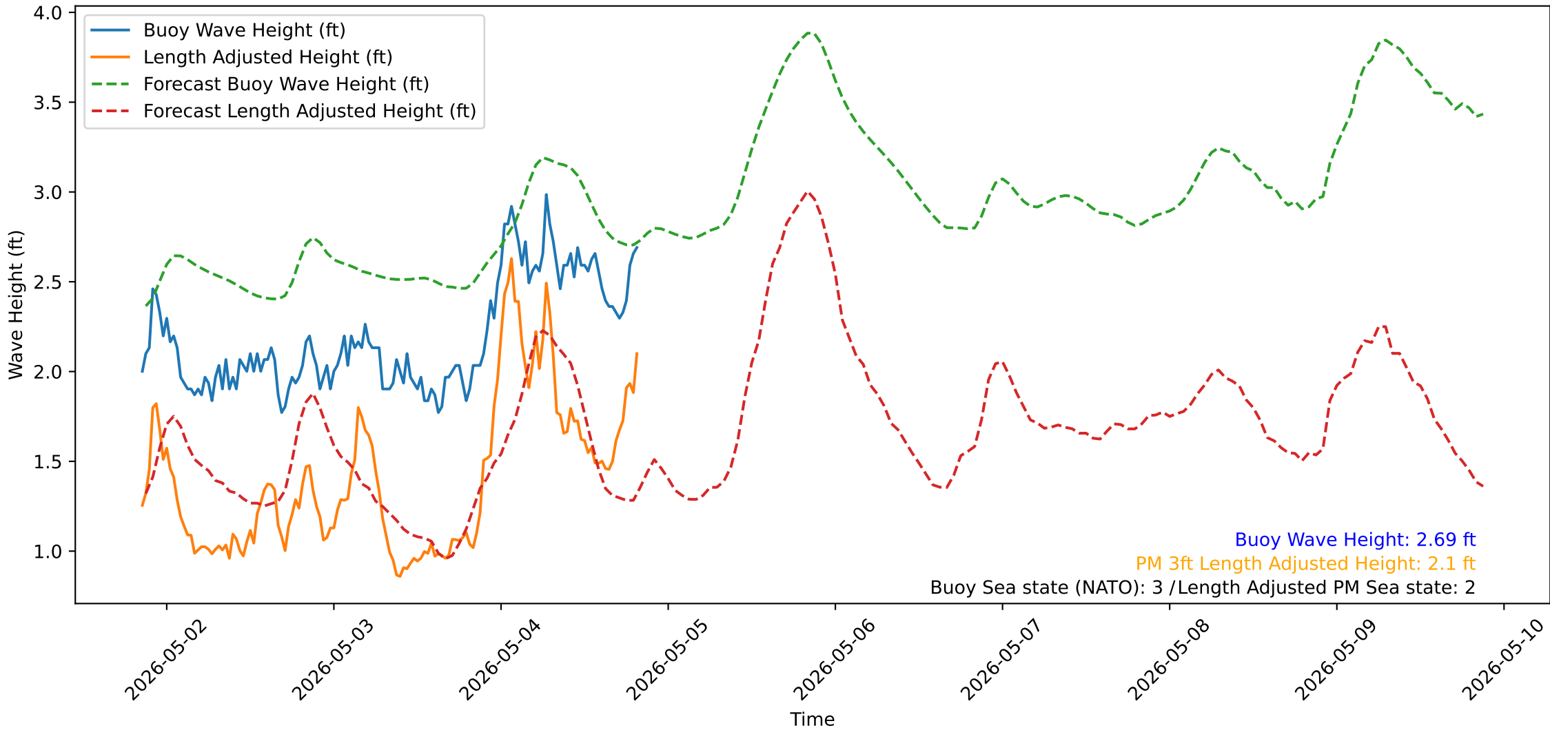
Wave Heights over Time for Green Beach at 2026-05-04 20:31:12
