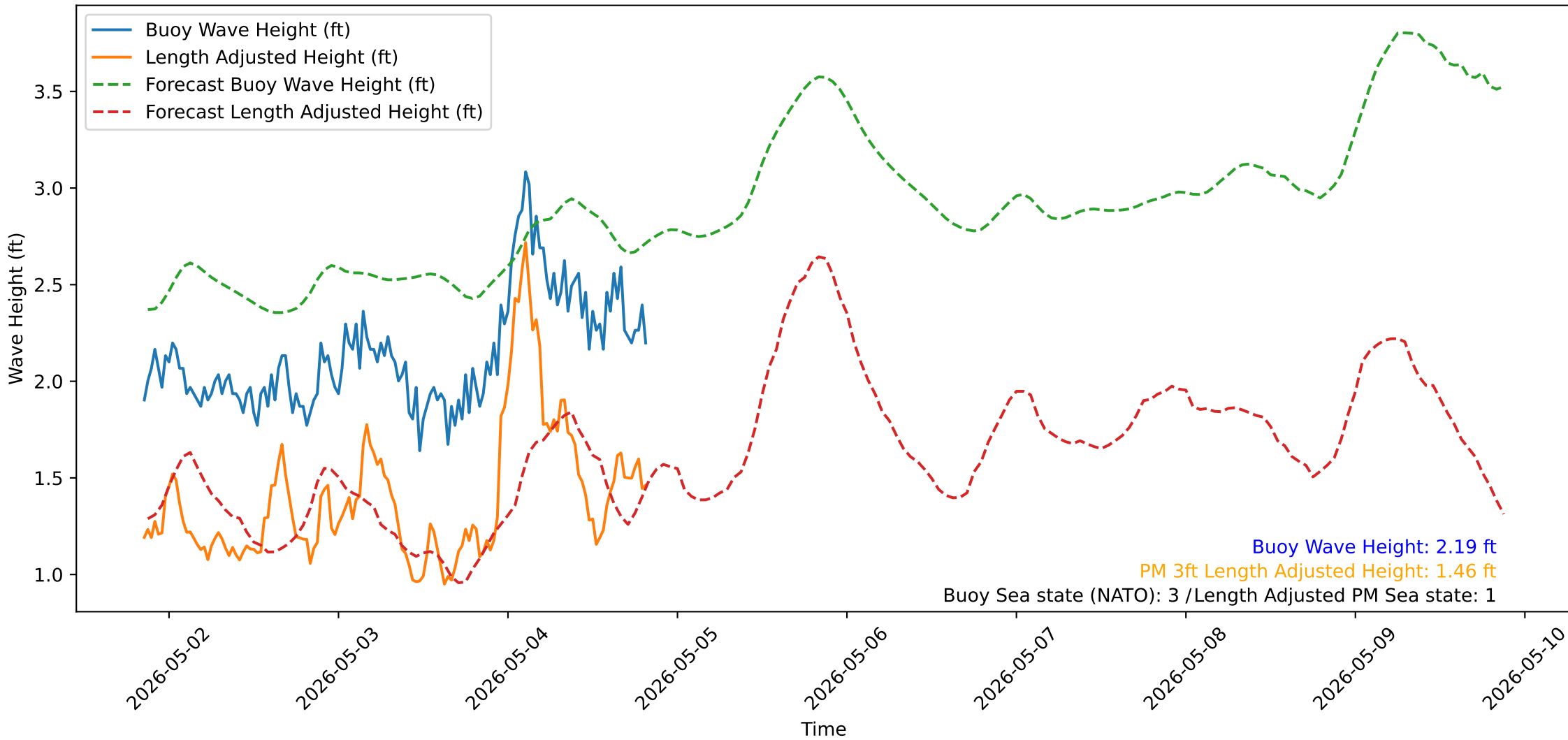
Wave Heights over Time for Oceanside Harbor at 2026-05-04 20:30:31
