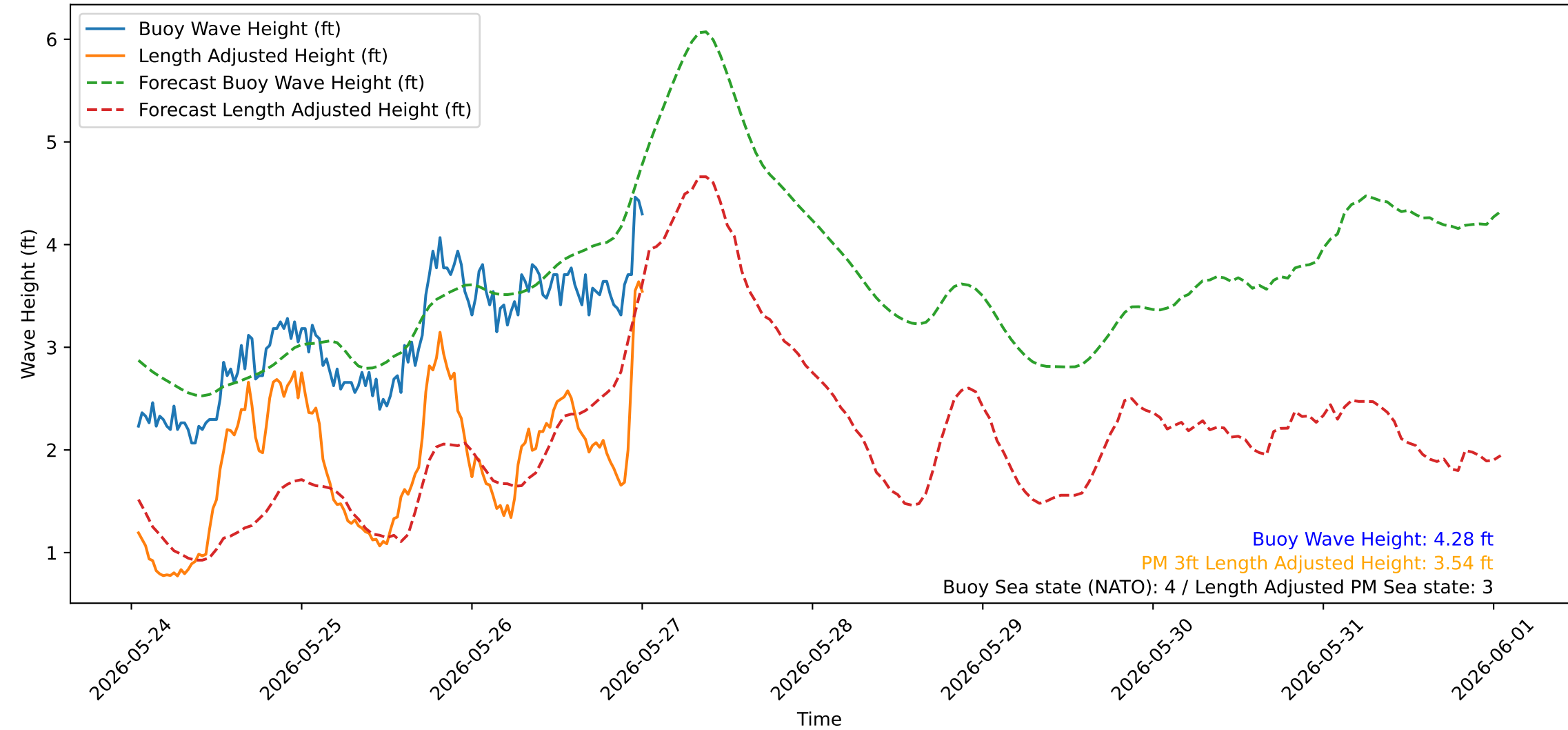
Wave Heights over Time for Green Beach at 2026-05-27 01:01:13
