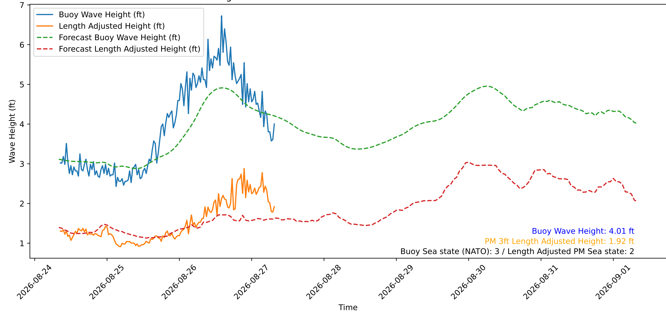
Wave Heights over Time for Oceanside Harbor at 2026-08-27 08:20:30
