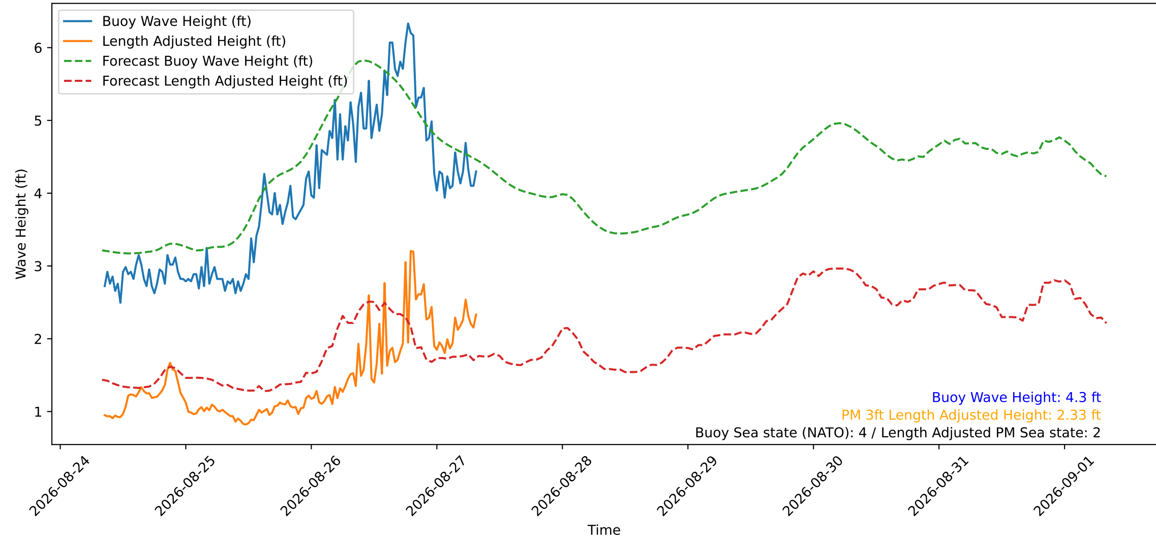
Wave Heights over Time for Green Beach at 2026-08-27 08:21:15
