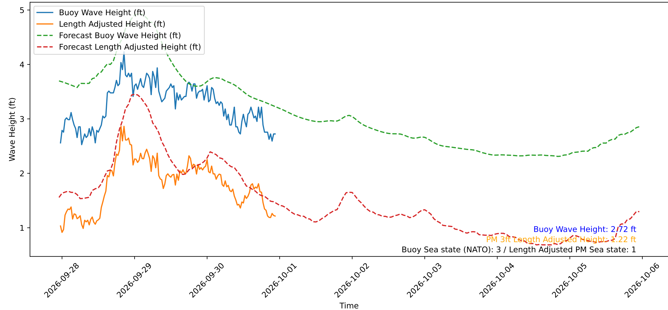
Wave Heights over Time for Oceanside Harbor at 2026-09-30 23:20:30
