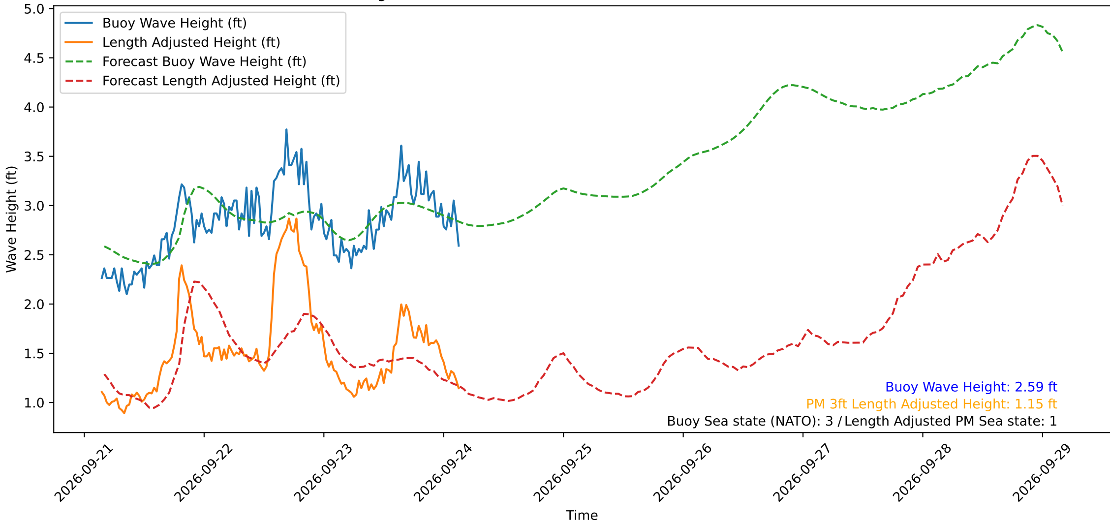
Wave Heights over Time for Oceanside Harbor at 2026-09-24 03:40:29
