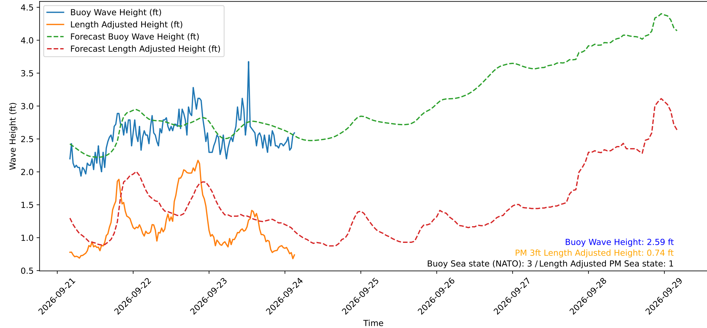
Wave Heights over Time for Red Beach at 2026-09-24 03:40:49
