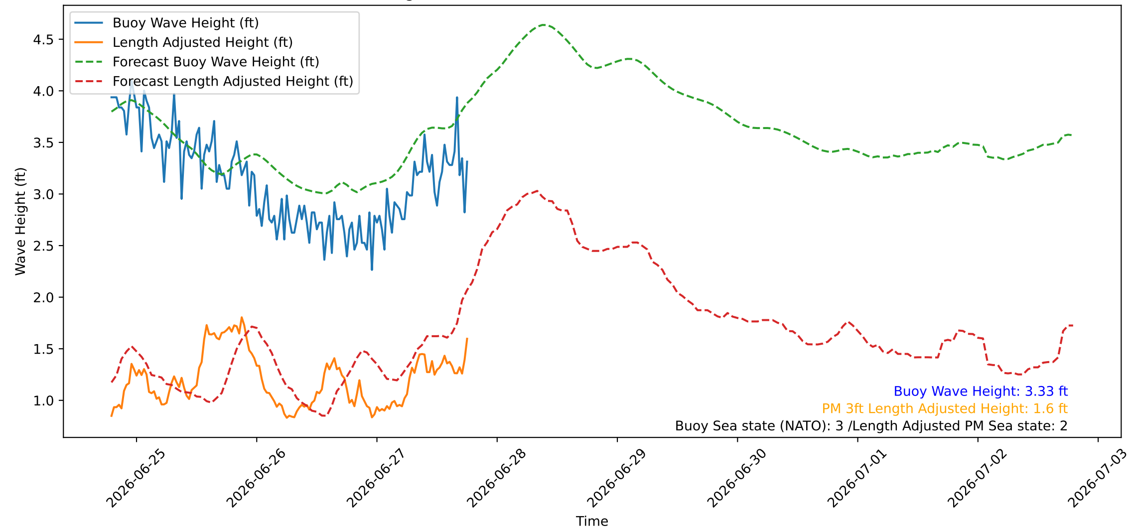
Wave Heights over Time for Green Beach at 2026-06-27 18:51:08
