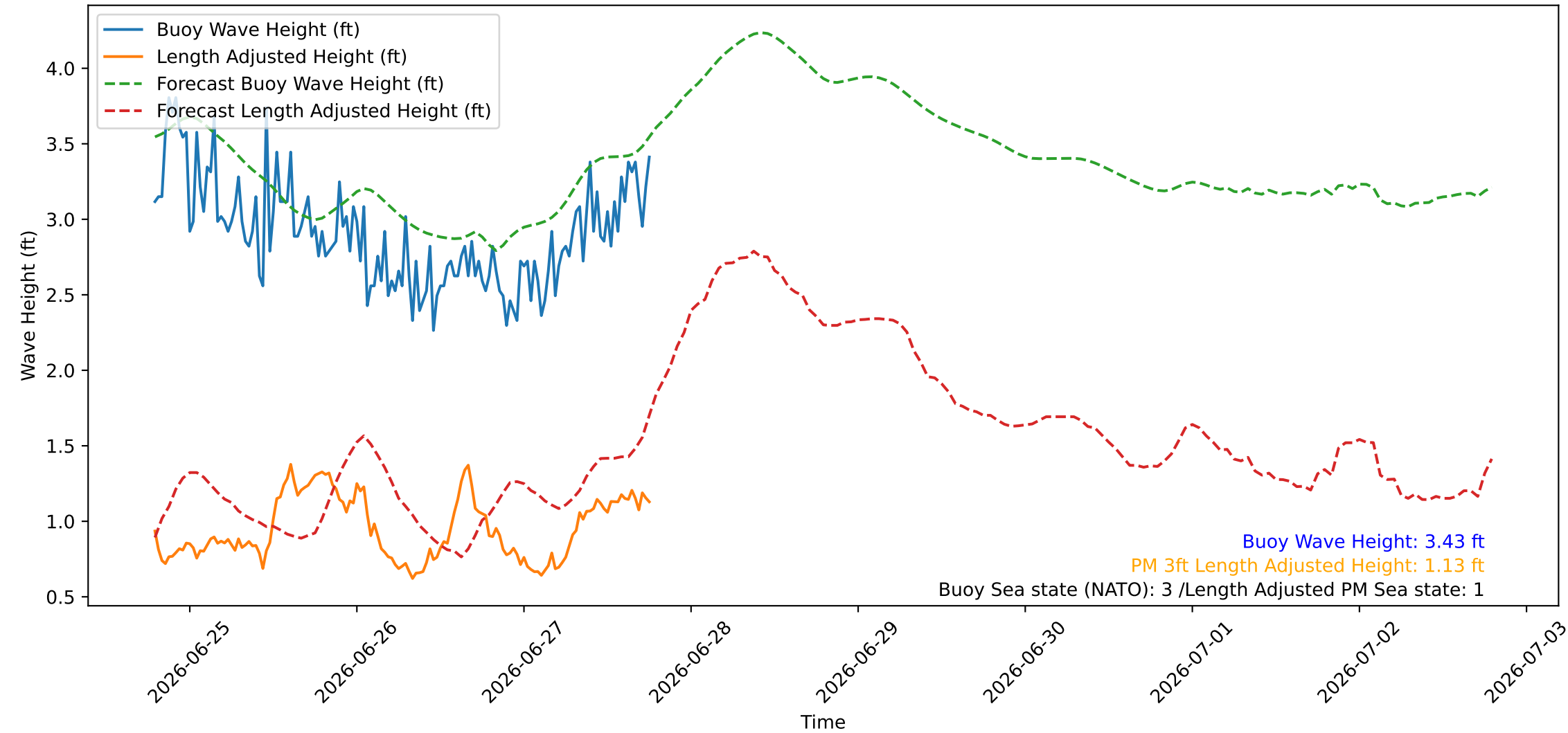
Wave Heights over Time for Red Beach at 2026-06-27 18:50:46
