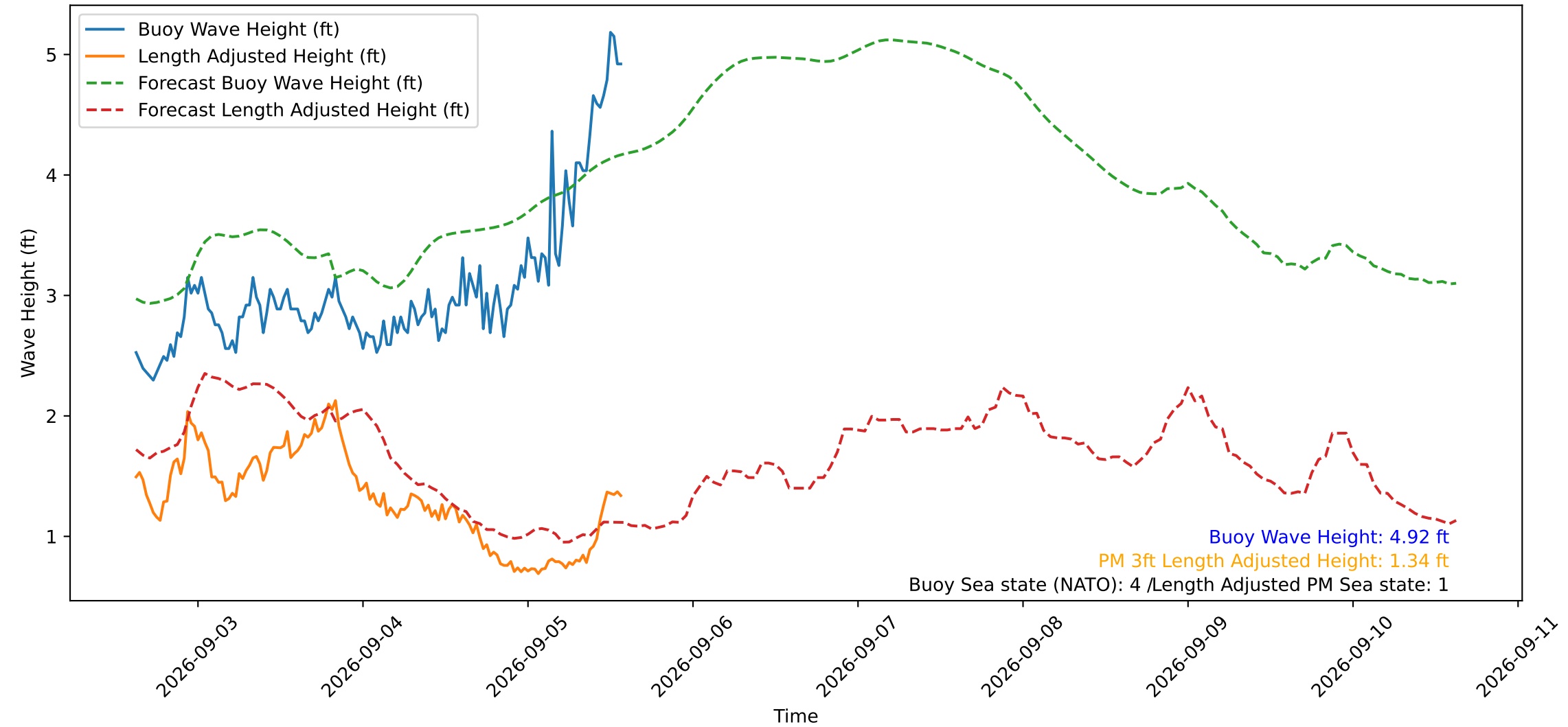
Wave Heights over Time for Red Beach at 2026-09-05 14:30:50
