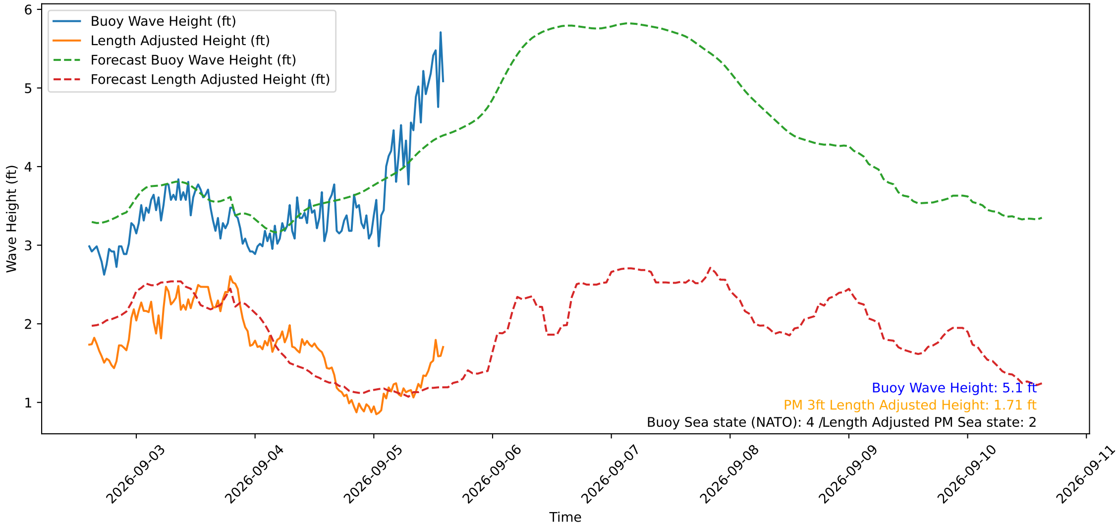
Wave Heights over Time for Oceanside Harbor at 2026-09-05 14:30:30
