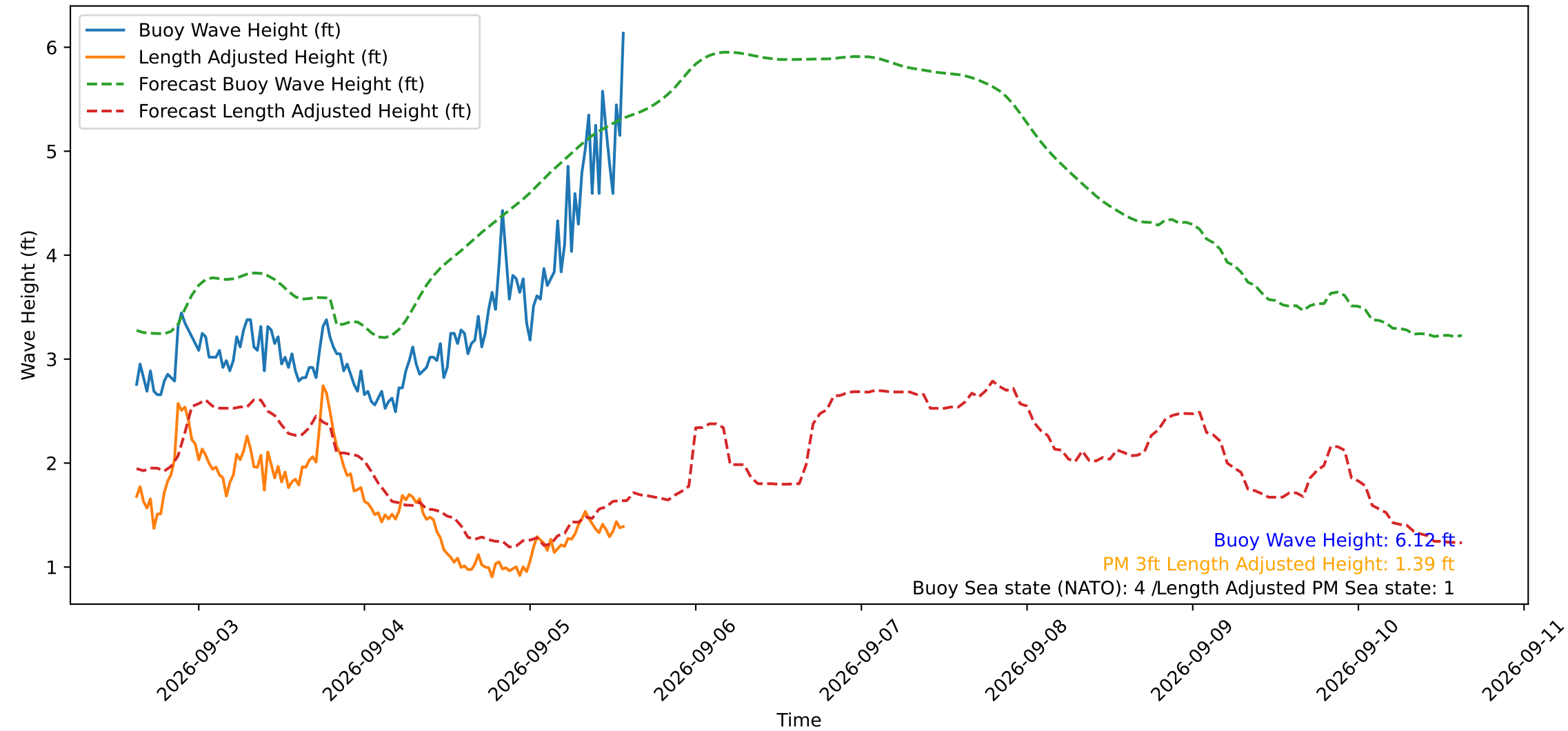
Wave Heights over Time for Green Beach at 2026-09-05 14:31:13
