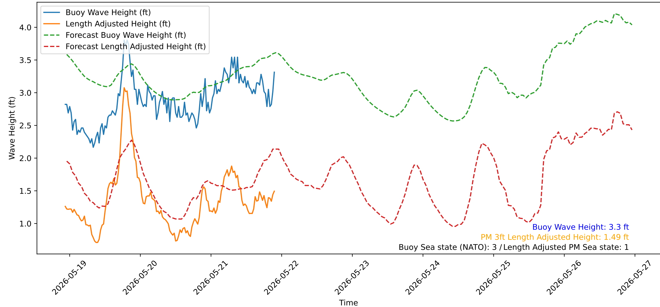
Wave Heights over Time for Green Beach at 2026-05-21 22:31:14
