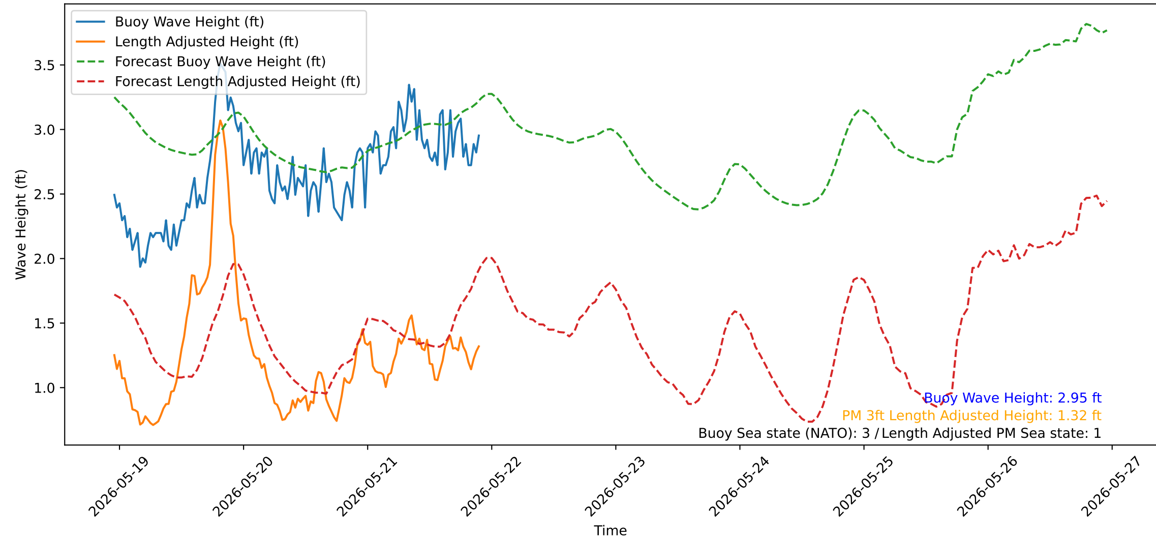
Wave Heights over Time for Red Beach at 2026-05-21 22:30:51
