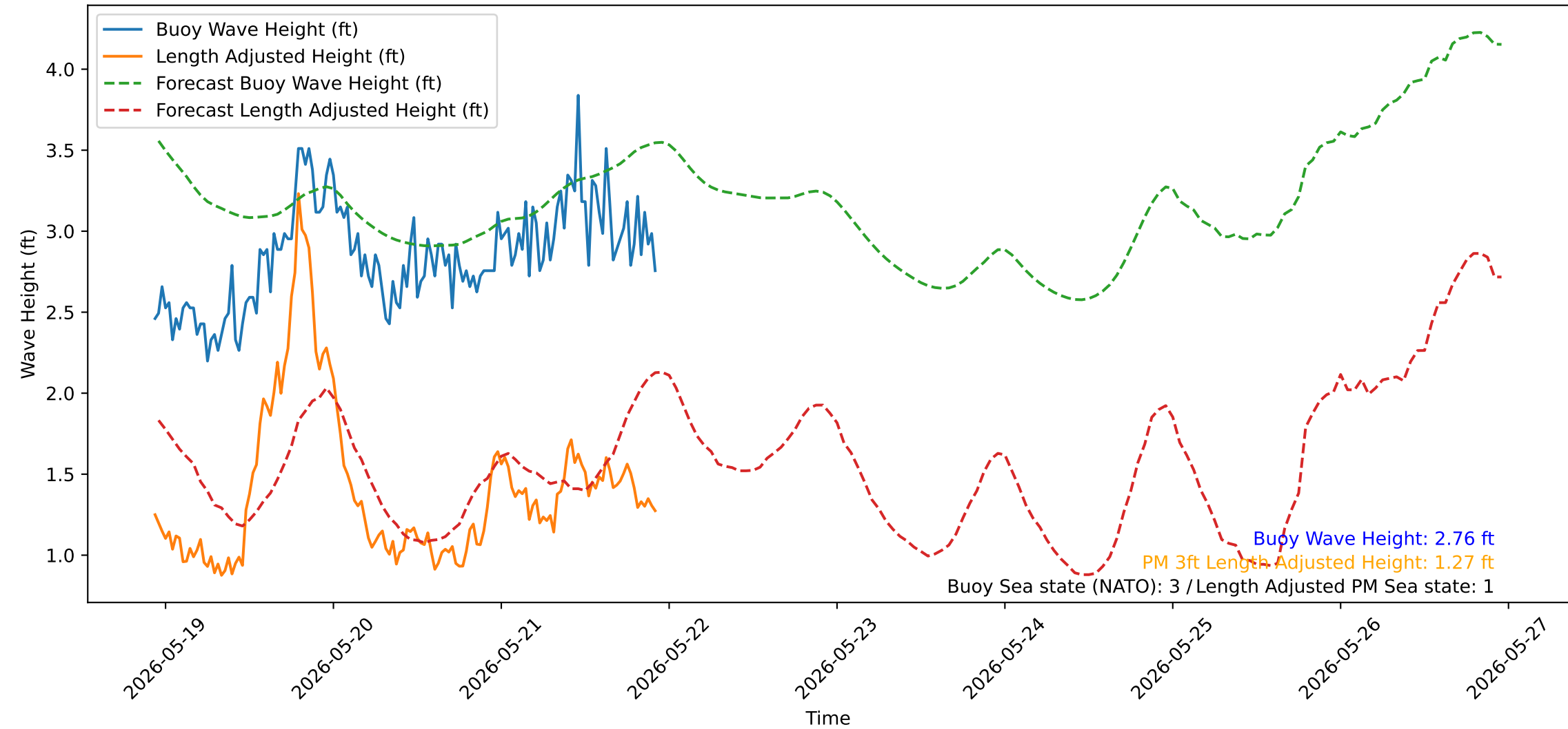
Wave Heights over Time for Oceanside Harbor at 2026-05-21 22:30:32
