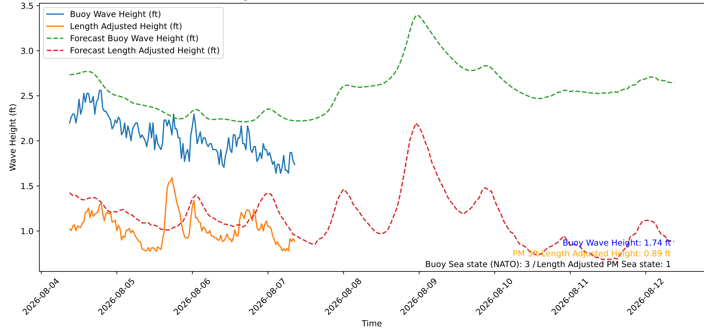
Wave Heights over Time for Oceanside Harbor at 2026-08-07 09:10:26
