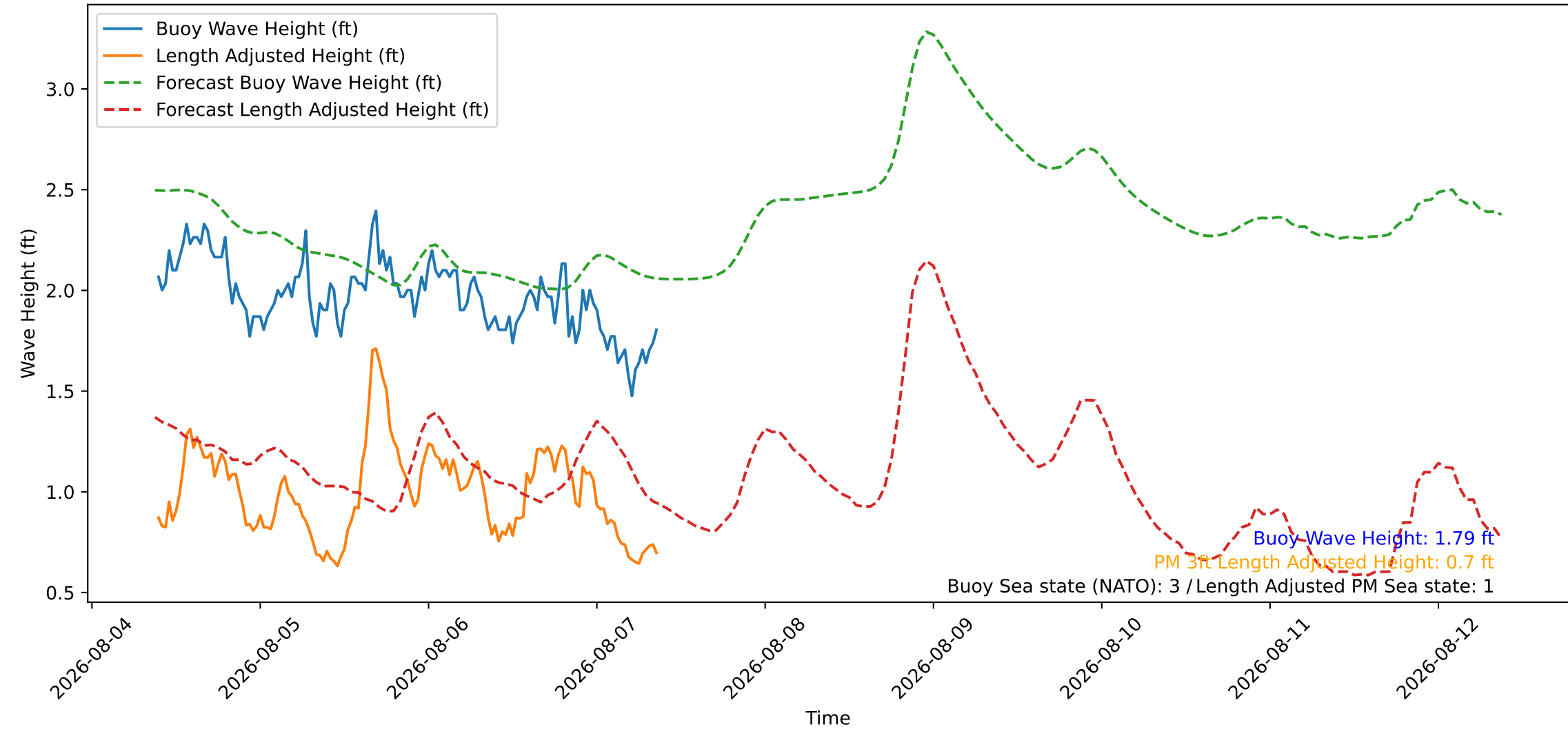
Wave Heights over Time for Red Beach at 2026-08-07 09:10:45
