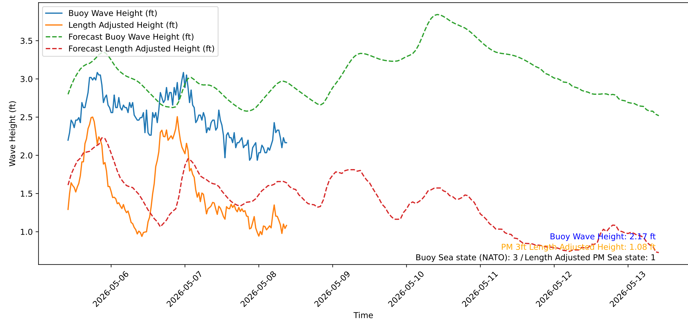
Wave Heights over Time for Red Beach at 2026-05-08 09:50:52
