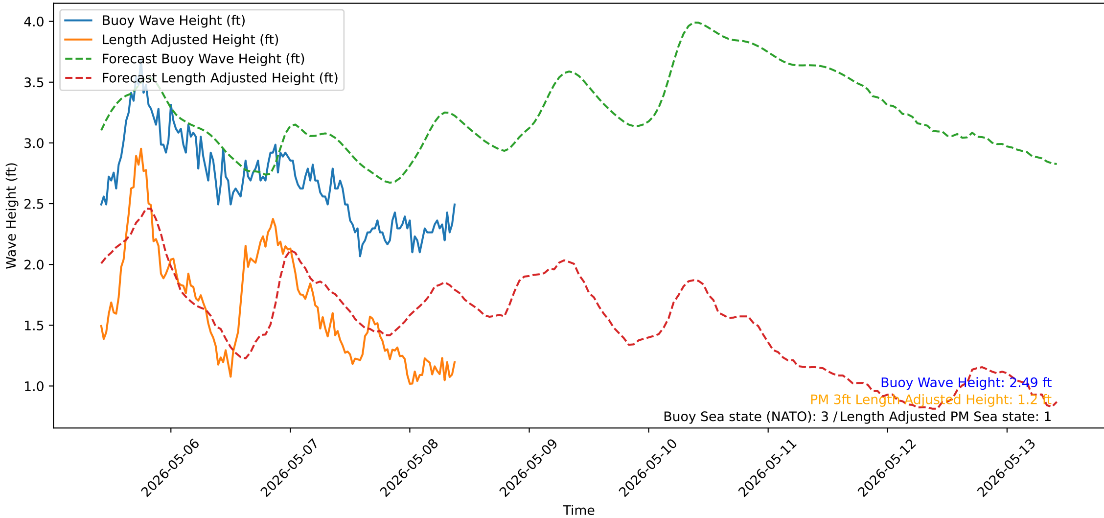
Wave Heights over Time for Green Beach at 2026-05-08 09:51:15
