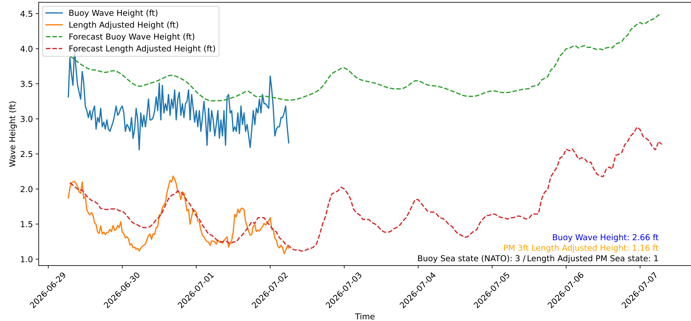
Wave Heights over Time for Oceanside Harbor at 2026-07-02 06:40:27
