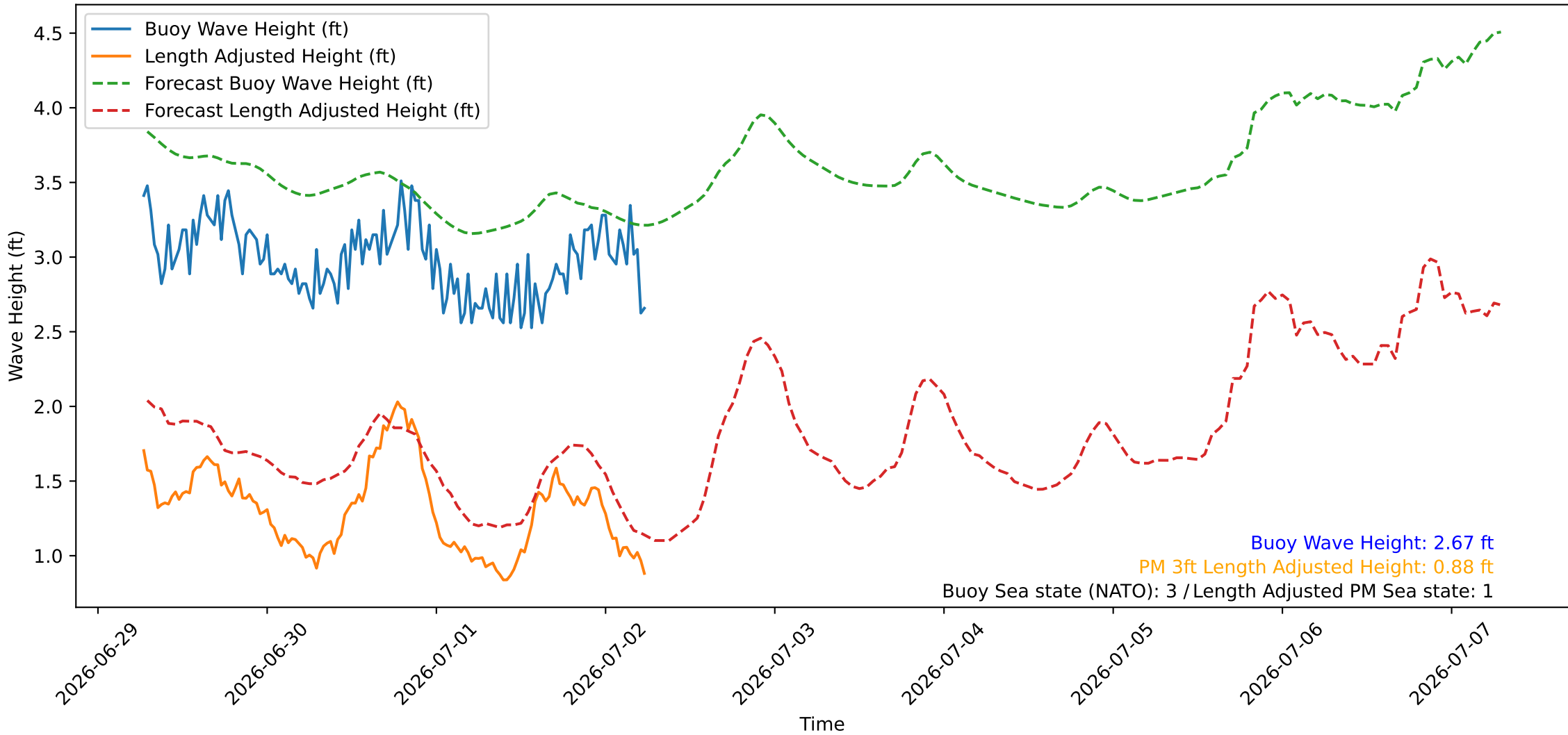
Wave Heights over Time for Green Beach at 2026-07-02 06:41:09
