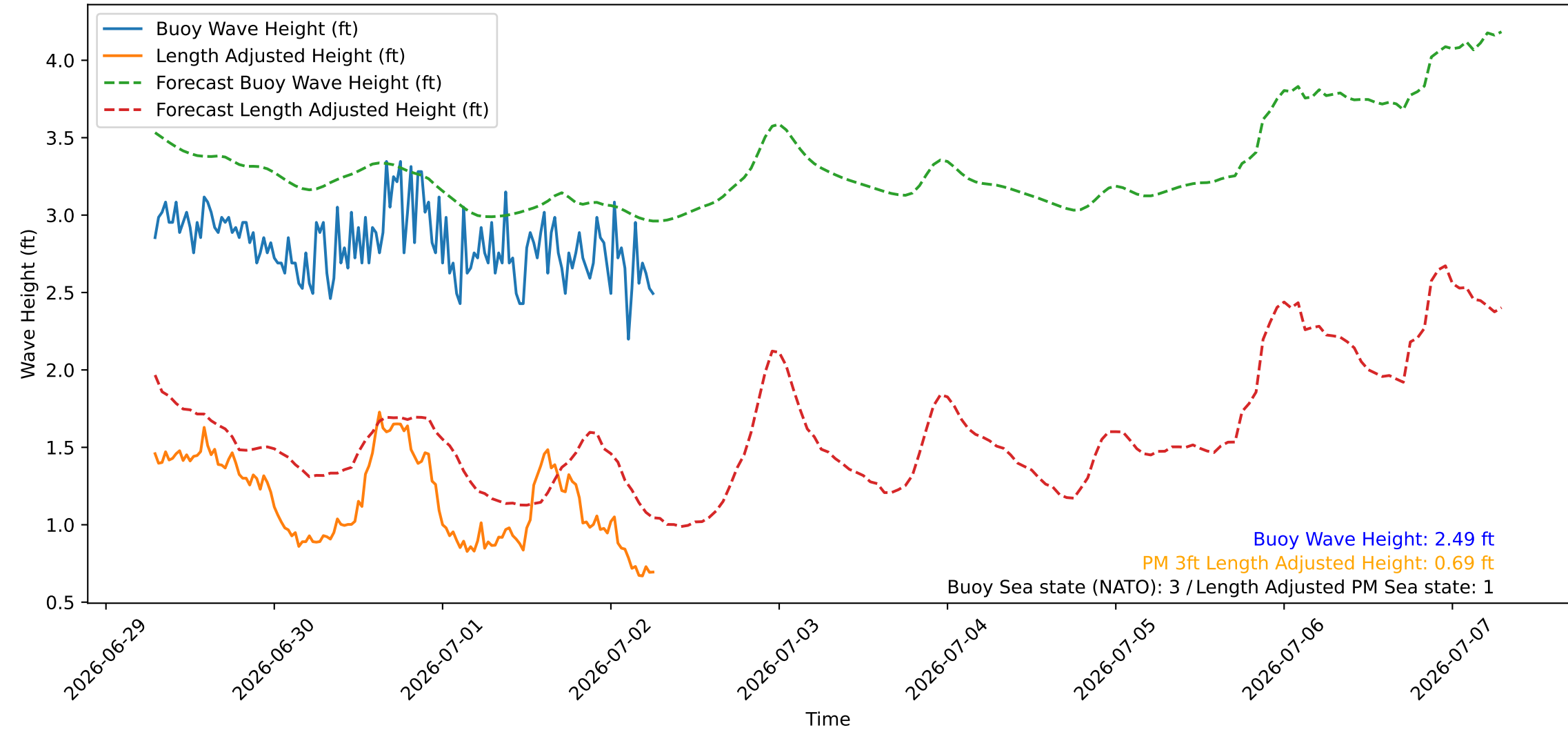
Wave Heights over Time for Red Beach at 2026-07-02 06:40:46
