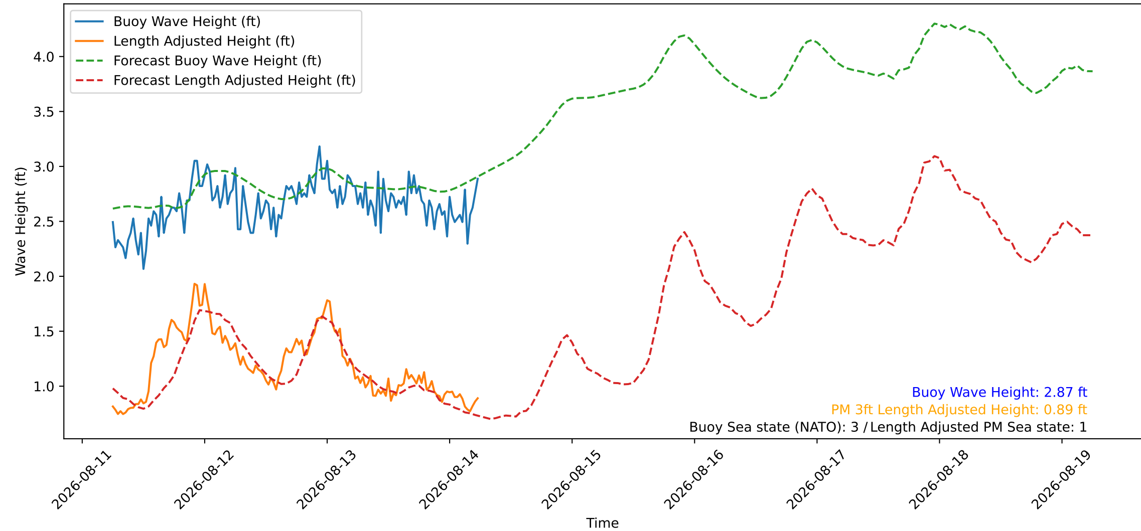
Wave Heights over Time for Oceanside Harbor at 2026-08-14 06:10:27
