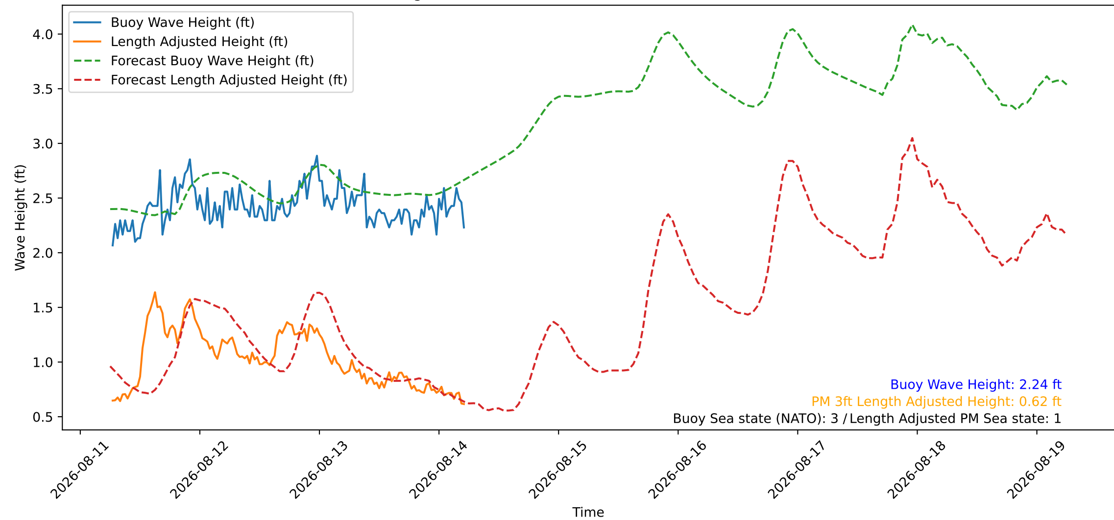
Wave Heights over Time for Red Beach at 2026-08-14 06:10:46
