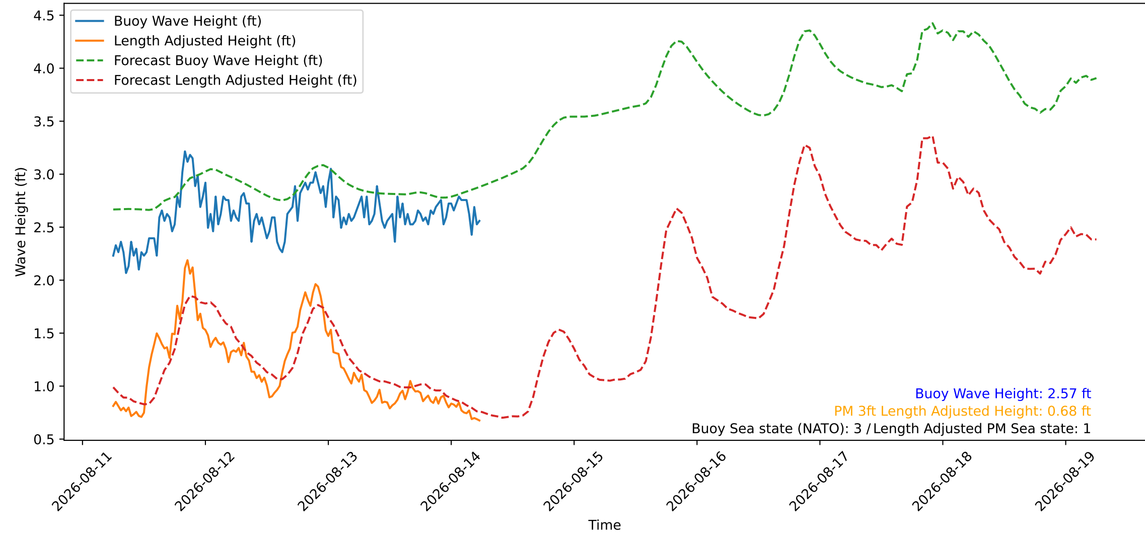
Wave Heights over Time for Green Beach at 2026-08-14 06:11:08
