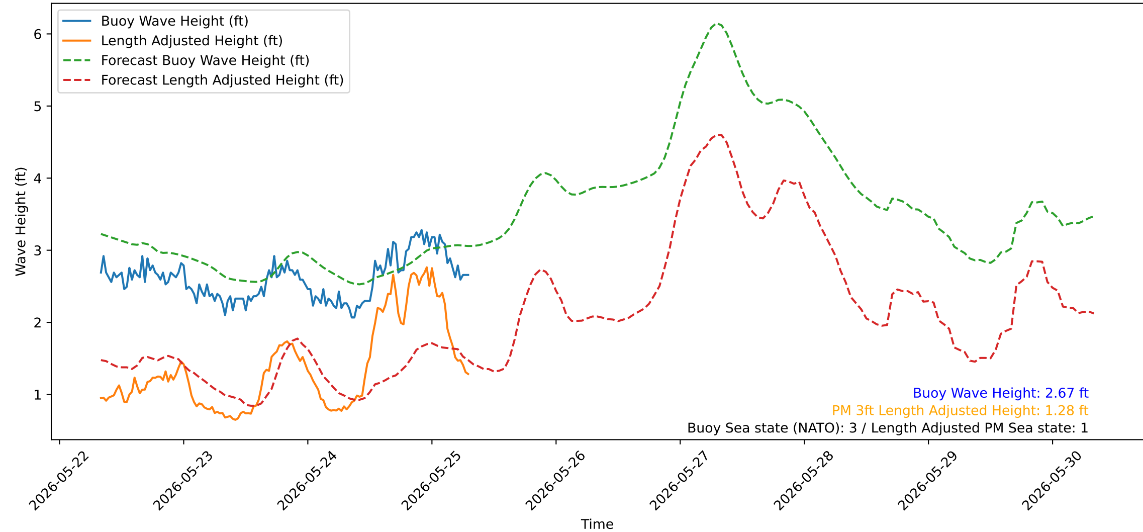
Wave Heights over Time for Green Beach at 2026-05-25 08:01:13
