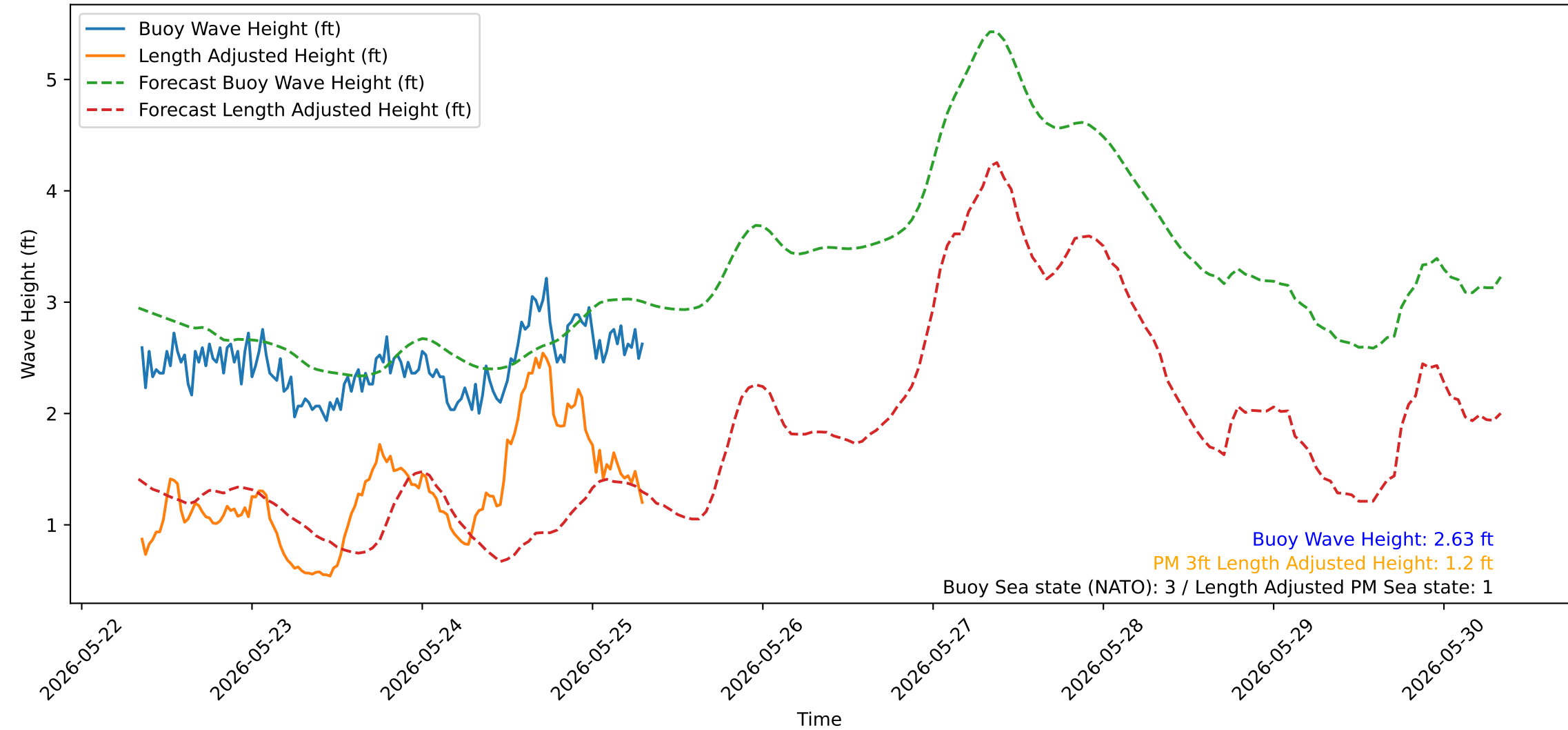
Wave Heights over Time for Red Beach at 2026-05-25 08:00:51
