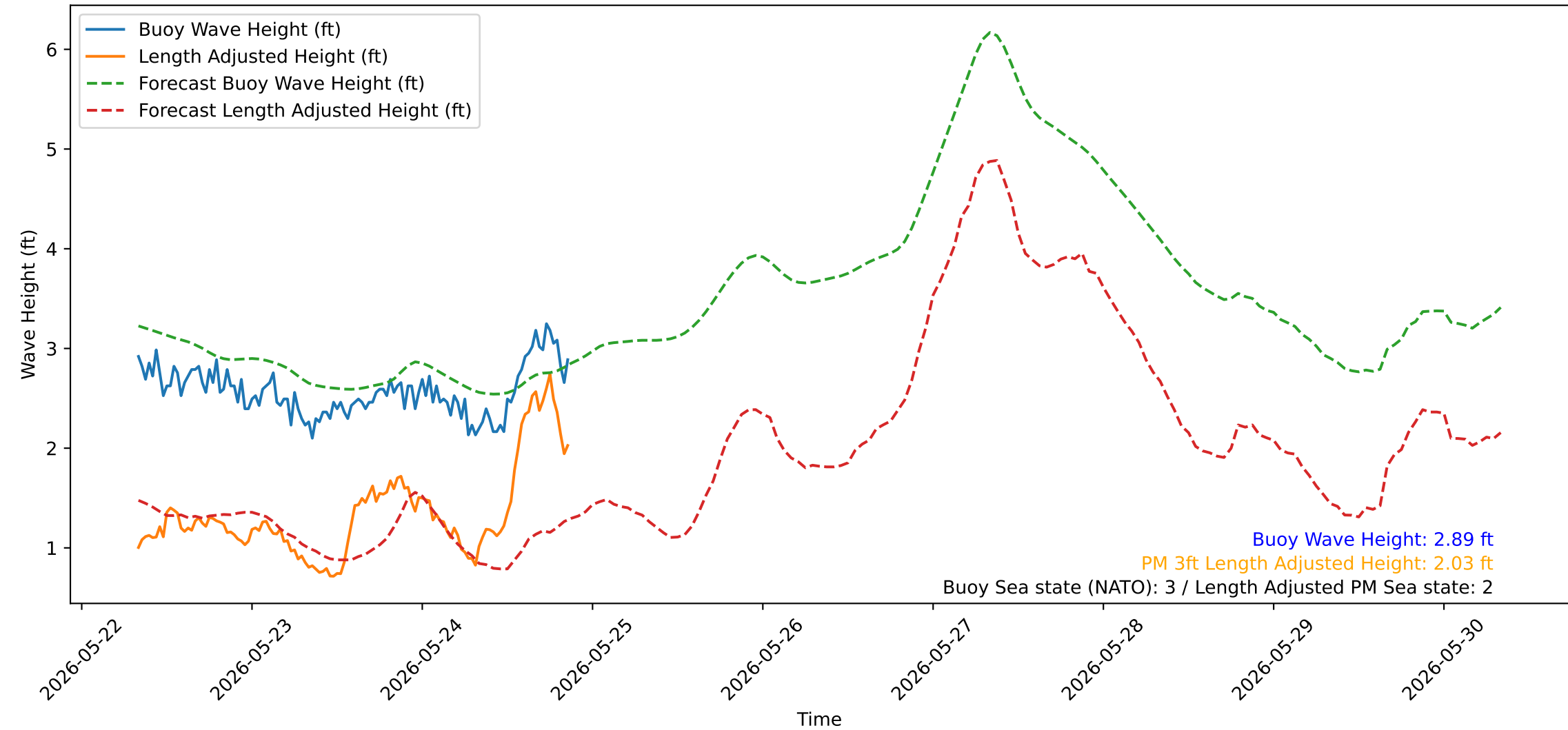
Wave Heights over Time for Oceanside Harbor at 2026-05-25 08:00:31
