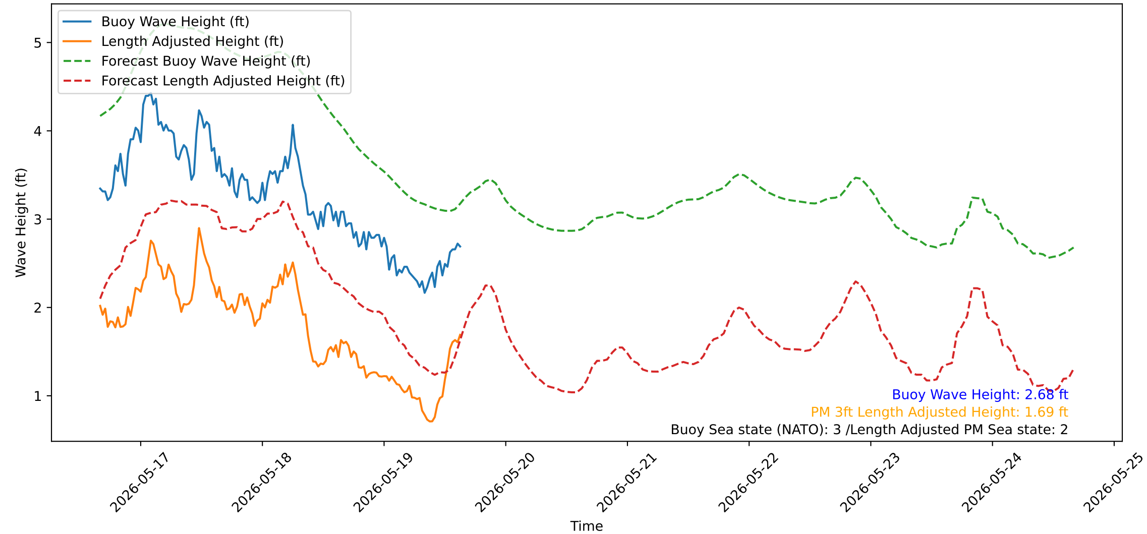
Wave Heights over Time for Green Beach at 2026-05-19 16:01:12
