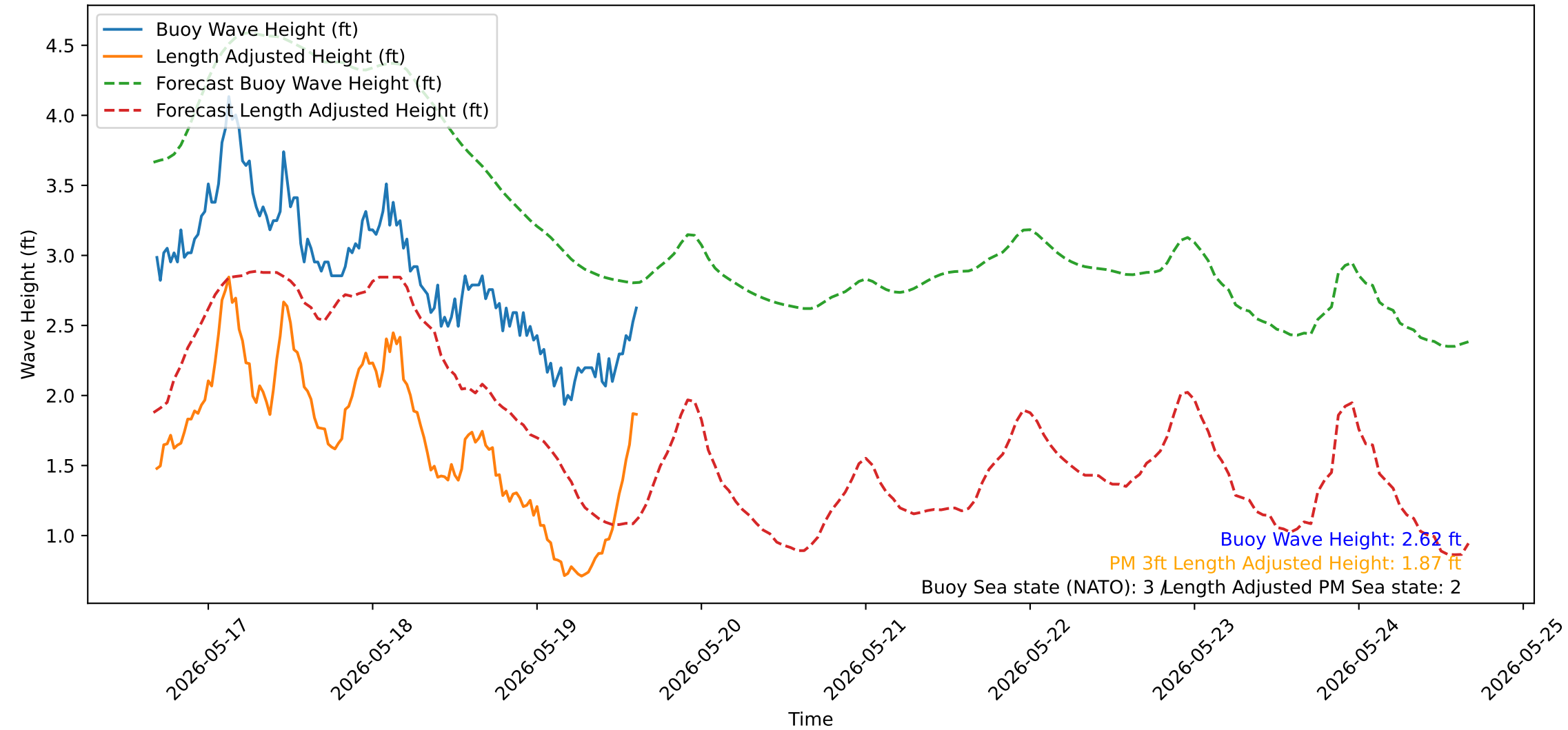
Wave Heights over Time for Red Beach at 2026-05-19 16:00:50
