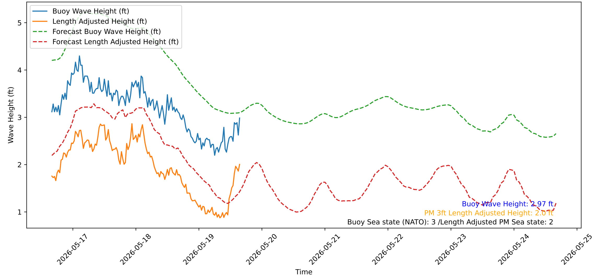
Wave Heights over Time for Oceanside Harbor at 2026-05-19 16:00:31
