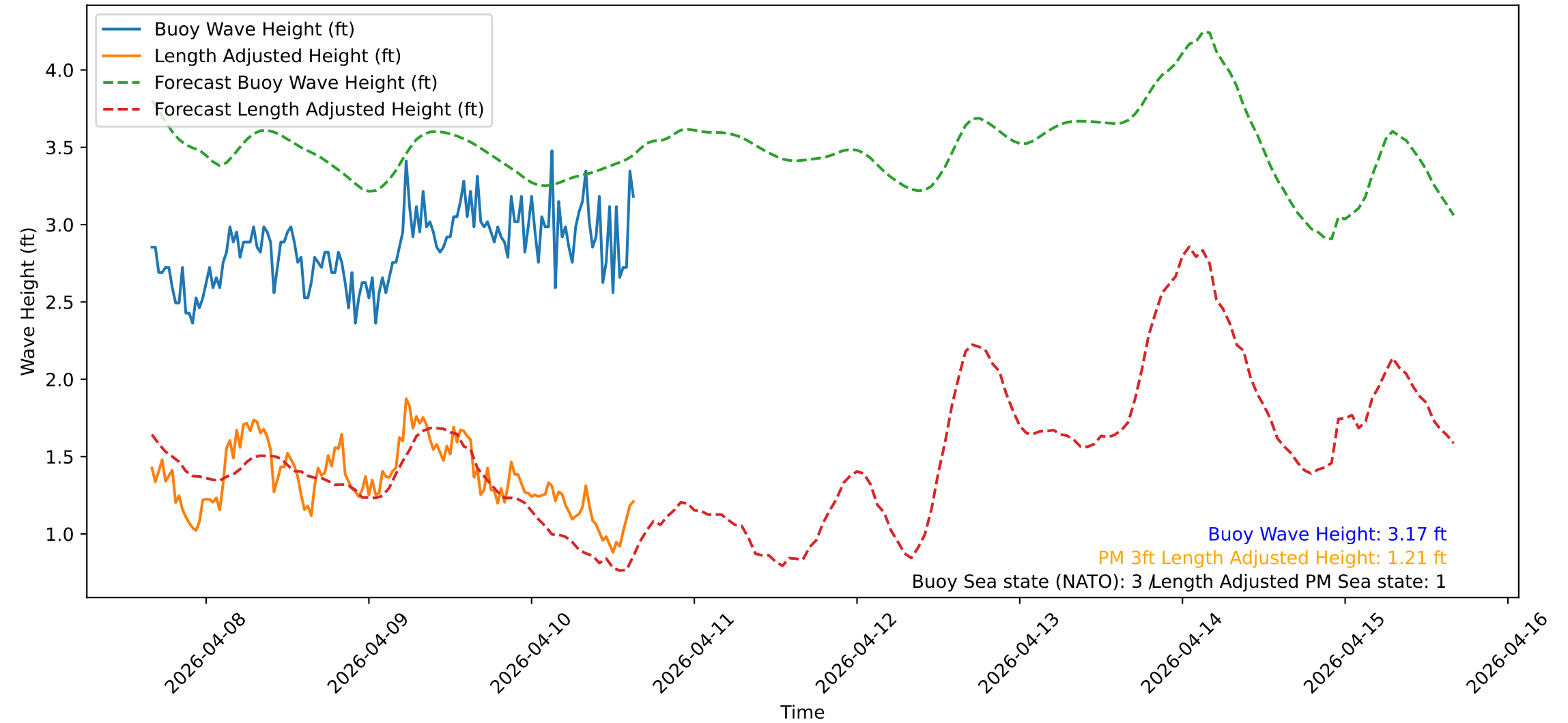
Wave Heights over Time for Green Beach at 2026-04-10 16:01:12
