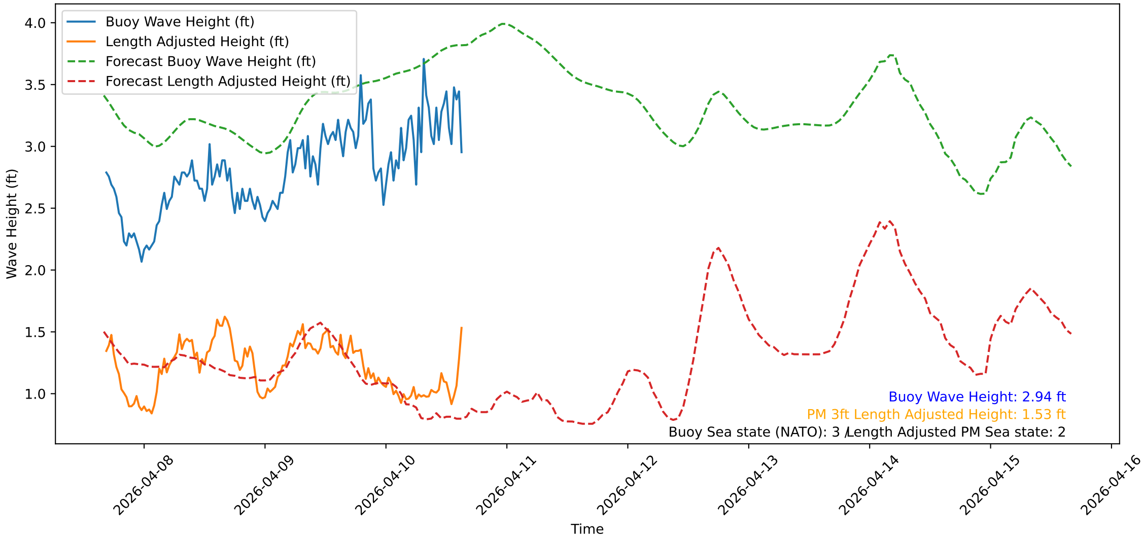
Wave Heights over Time for Red Beach at 2026-04-10 16:00:50
