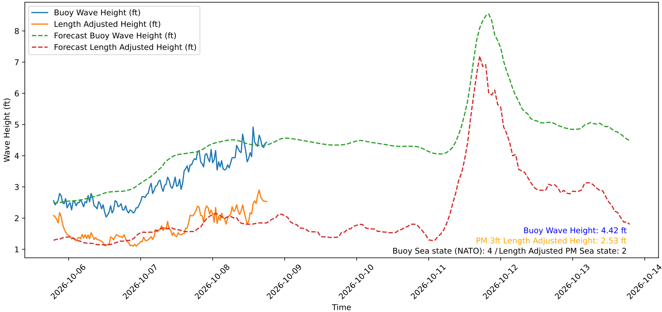
Wave Heights over Time for Oceanside Harbor at 2026-10-08 18:50:30
