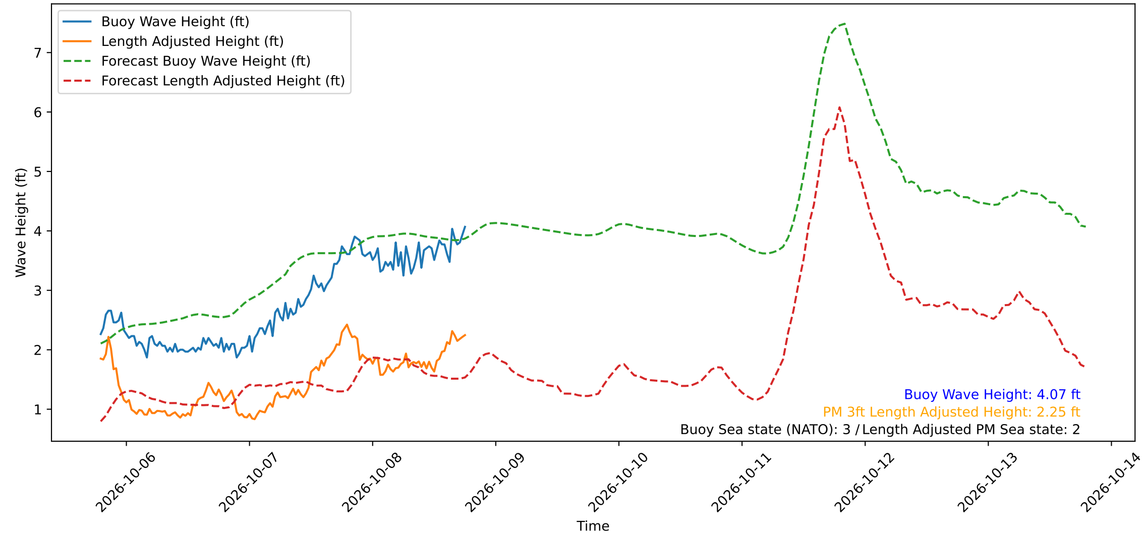
Wave Heights over Time for Red Beach at 2026-10-08 18:50:50
