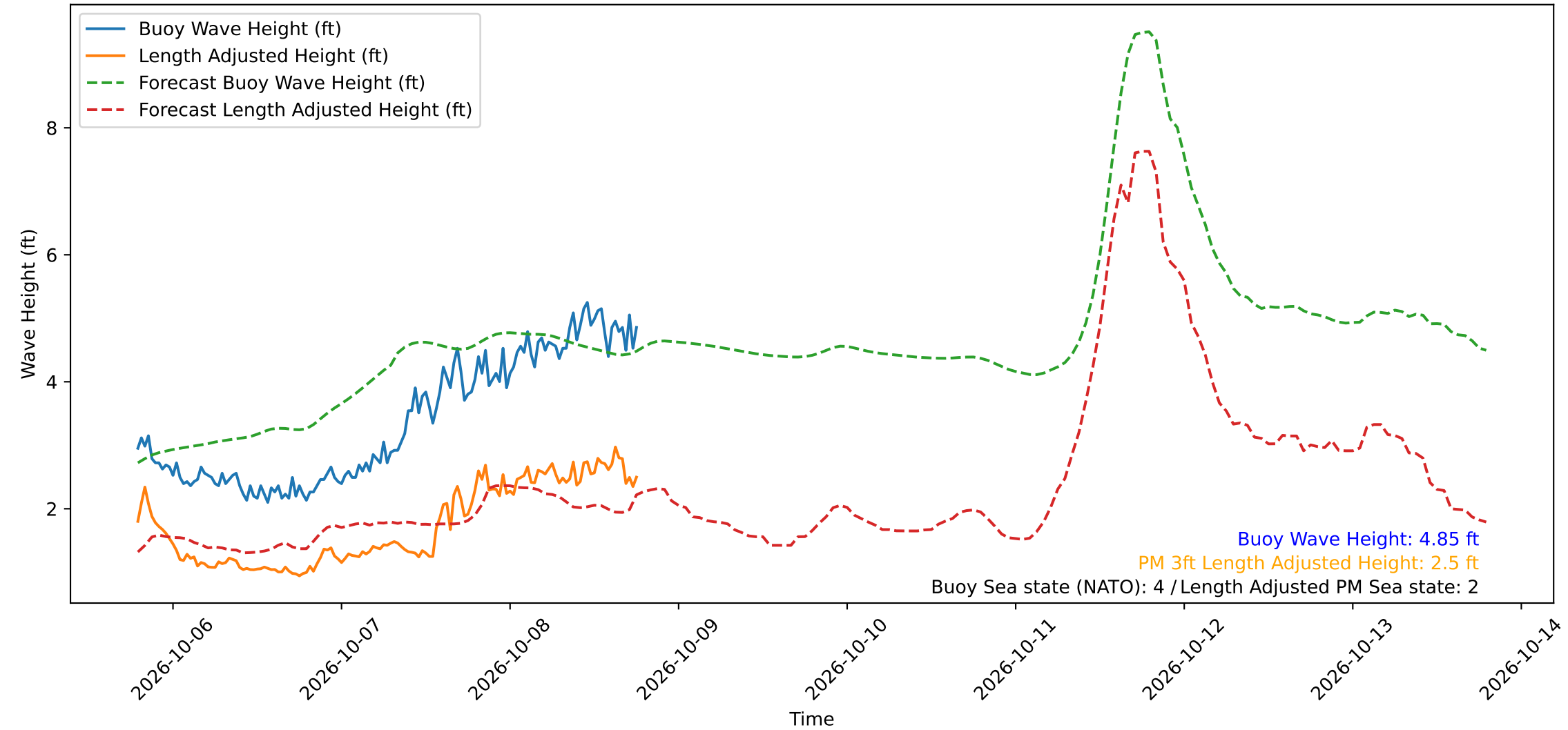
Wave Heights over Time for Green Beach at 2026-10-08 18:51:14
