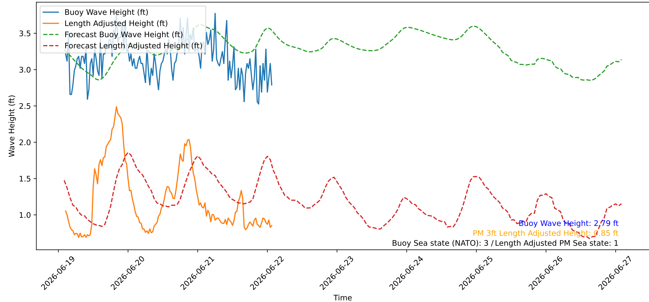
Wave Heights over Time for Red Beach at 2026-06-22 02:20:46
