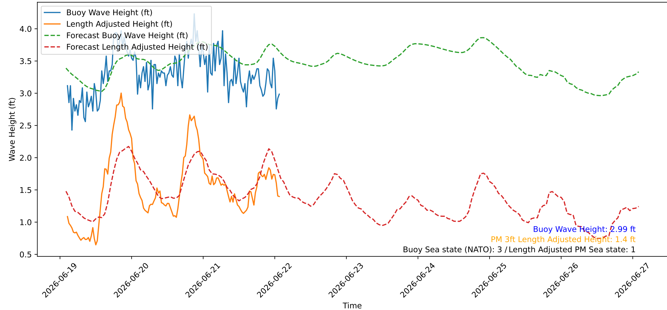
Wave Heights over Time for Green Beach at 2026-06-22 02:21:08
